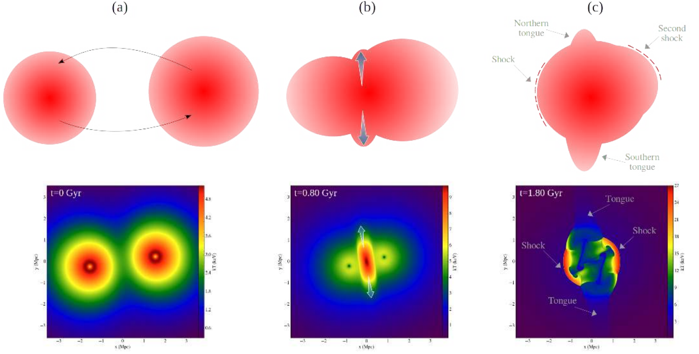
Fig. 12. Top panels: Schematic representation of the proposed merger scenario for A754. (a) Two clusters undergo a slightly off-axis collision nearly in the plane of the sky. (b) As clusters approach, the gas in-between is squeezed and propagates in equatorial directions. (c) In the current configuration of A754, tongues of cold and low entropy plasma develop and shock fronts propagate in opposite directions roughly along the merger axis. Bottom panels: temperature slices (for the z projection) from an idealized simulation by ZuHone et al. (2018) of a 1:1 merger with an impact parameter of 500 kpc taken at different times and used to support our sketched merger scenario of A754.
