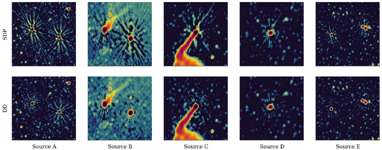
Fig. 4. Zoom-in images of sources A to E (left to right) for the images obtained with the SDP Continuum pipeline calibration ( top panels ) and after direction-dependent calibration with facetselfcal.py ( bottom panels ).
