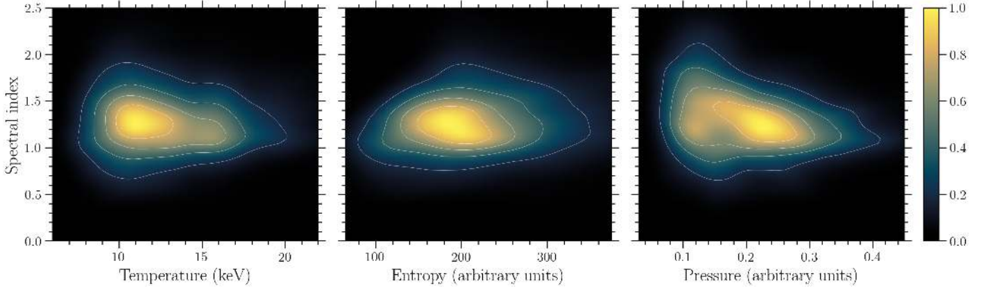
Fig. 13. Normalized 2D KDE distributions between spectral index and thermodynamic properties of the ICM, with isocontours drawn at the same levels (0.2, 0.4, 0.6, 0.8).
