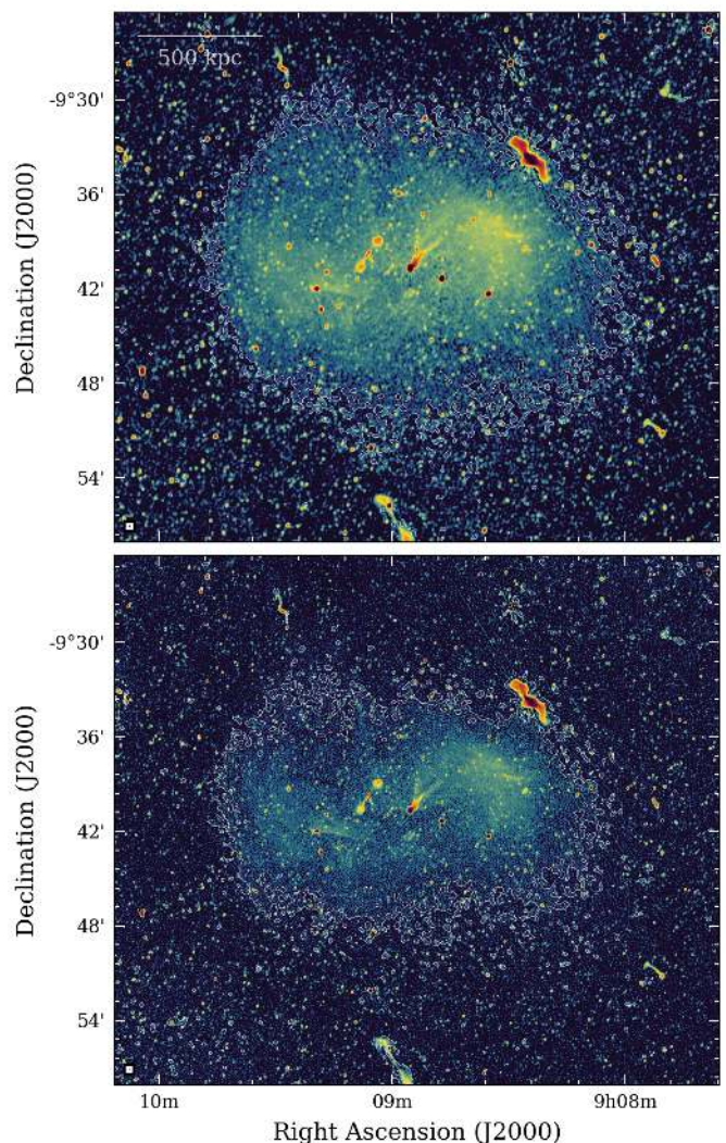
Fig. 5. Radio halo recovered with MeerKAT at 819 MHz (UHF, top panel ) and at 1.28 GHz (L, bottom panel ). The colors show high-resolution images while the contour represent the 3\sigma emission from a lower resolution image with discrete sources subtracted (see Tab. 2 for more details).
