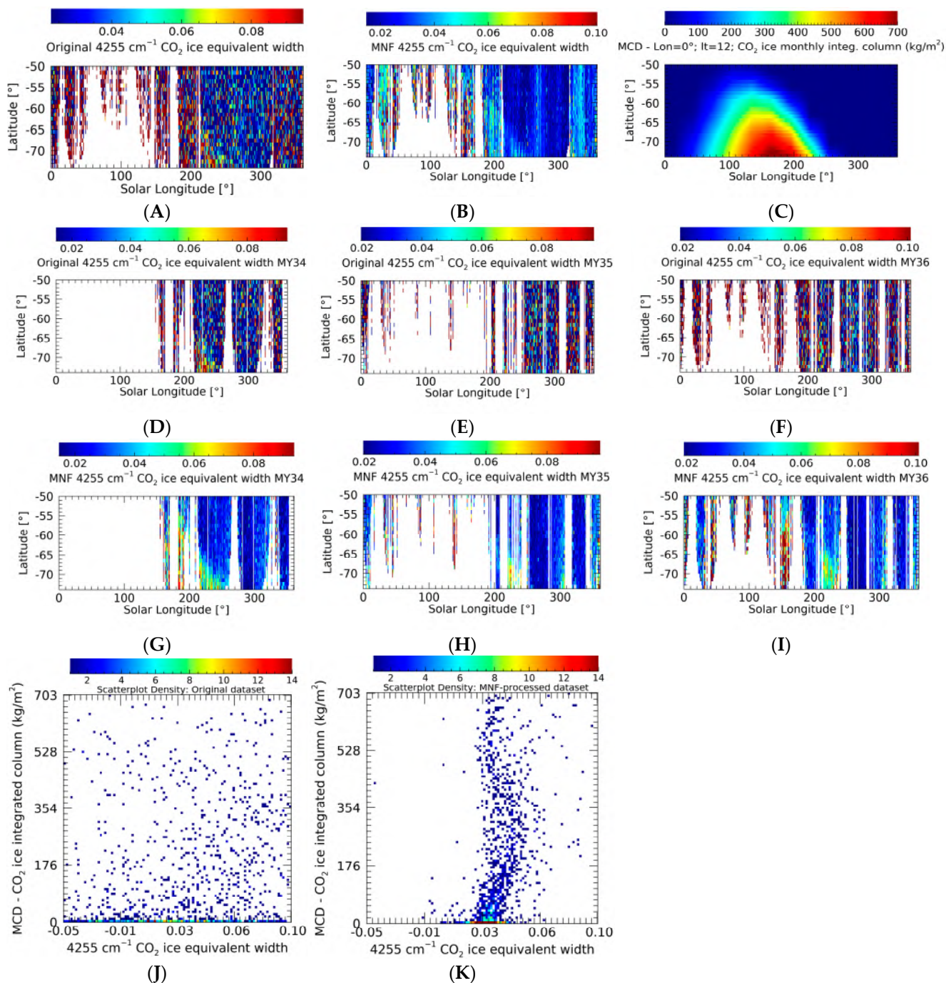
Figure 10. (A) Equivalent width of the CO 2 ice 4255 cm -1 absorption band computed on all MY34–35–36 LNO order 189 original data. (B) Same as in panel (A), but the equivalent width is computed on all MY34–35–36 MNF-processed data. (C) MCD simulation of the monthly integrated CO 2 ice column in kg/m 2 . Panels (D–F) are the same as panel (A), but the data are separated into MY34, 35, and 36, respectively. Similarly, panels (G–I) show the MNF-processed equivalent width for MY34, 35, and 36, respectively. Panels (J,K) provide the density scatter plots between the quantities in panels (C)/(B) and (C)/(A), respectively, considering observations in the Ls range of 190°–210°.
