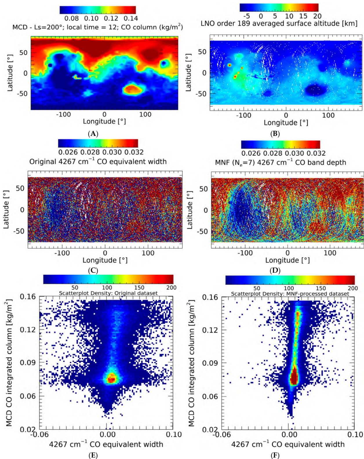
Figure 9. (A) MCD simulation of the CO-integrated column in kg/m². (B) LNO order 189 data averaged surface altimetry in km (from MOLA data, [37]). (C) Equivalent width of the CO 4267 cm⁻¹ absorption line computed on LNO order 189 original data. (D) Equivalent width of the CO 4267 cm⁻¹ absorption line computed on the MNF-processed data ( N_e = 7 ). (E) Density scatter plot of the quantities in panels (A,C). (F) As in panel (E), but here the quantities in panels (A,D) are being compared.
