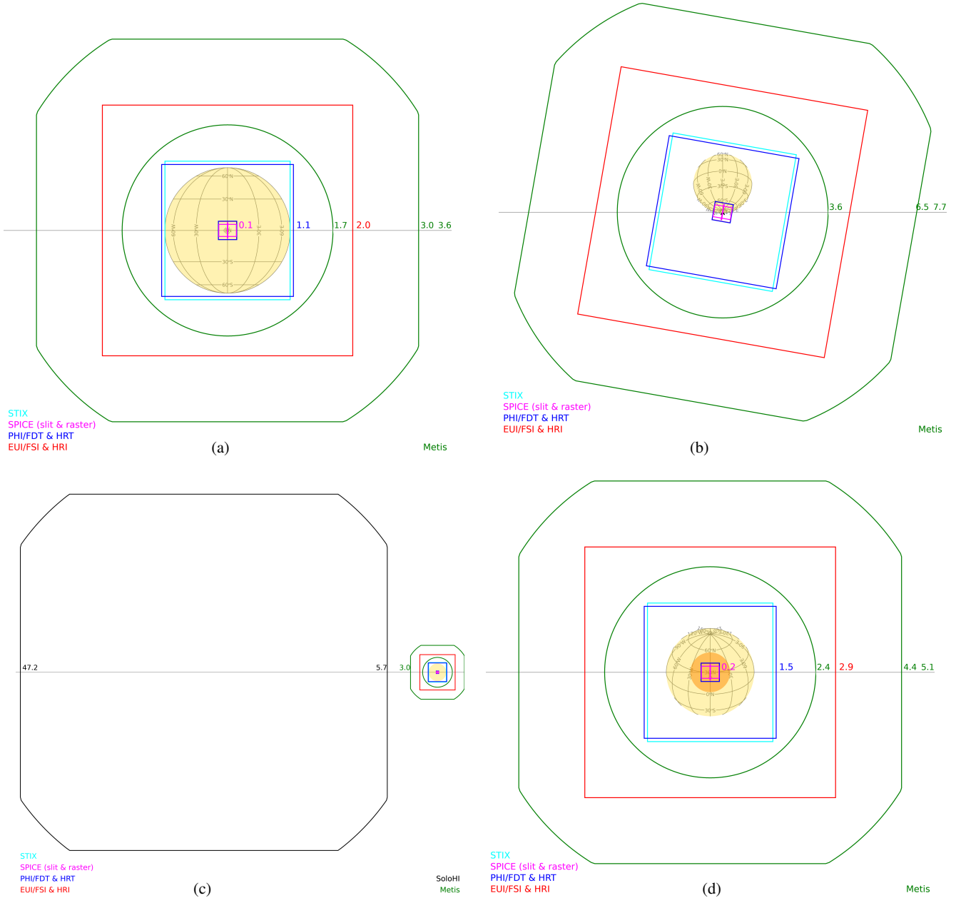
Fig. 1. Fields of view (FOVs) of the remote-sensing instruments in various orbital configurations and distances from the Sun. The extents of the FOVs are labelled in solar radii. The PHI/HRT, EU/FISI 174 , and EU/FISI L α FOVs are completely overlapping. In the cases where off-points are limited by the Metis safety constraint, the area on the solar disc within which off-pointing is allowed is highlighted in orange (see e.g. (d)). (a) Closest perihelion at 0.28 AU, disc centre pointing. (b) Off-point to solar pole, at 0.6 AU, S/C rolled 10° with respect to solar north. (c) All RS FOVs, incl. SoloHI, at 0.3 AU perihelion. (d) Maximum latitude case (30° N), at 0.4 AU.
