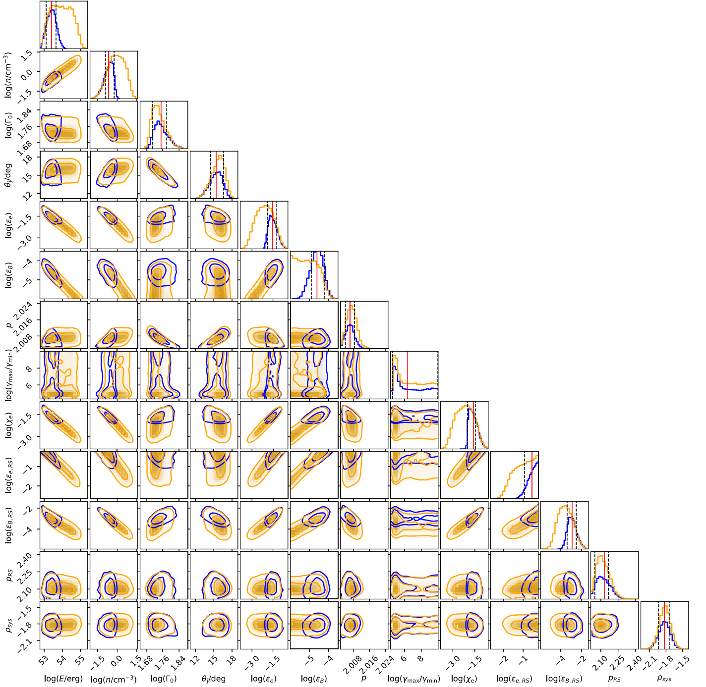
Figure 11. Corner plot of the MCMC posterior sample density distributions. Orange histograms and contours show the results for the wide \chi_e prior, while the blue ones are for the narrow prior. The black dashed lines in the plots on the diagonal bracket the 1\sigma credible interval, while the red solid lines mark the position of the estimated best fit.
