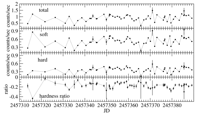
Figure 4. X-ray light curves of NGC 7469 in the hard (2.0–10.0 keV), soft (0.3–2.0 keV), and full bands. The light curve of the \text{HR} = (H - S)/(H + S) is also plotted.
