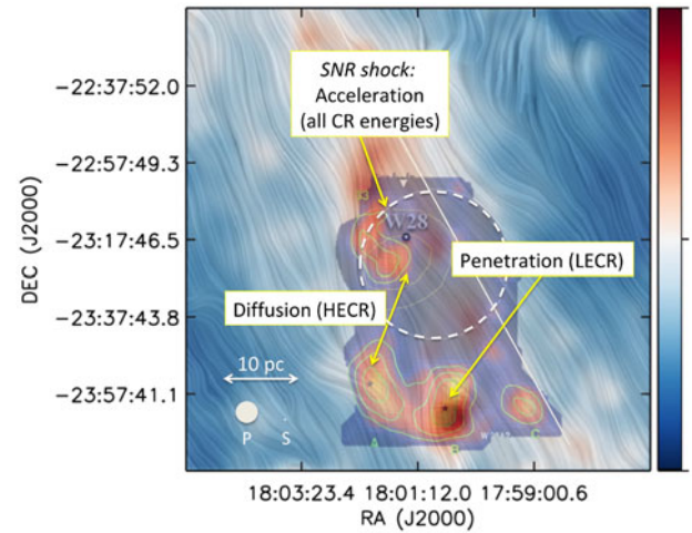
Figure 14. The region surrounding the W28 SNR ( d \approx 2 kpc; shock approximated by the dashed white circle), as seen in cold dust emission at 353 GHz by Planck (colour image with background B-field ‘drapery’ from polarisation data), in TeV–GeV \gamma -rays (white contours), and CO (green areas, well correlated with the \gamma -ray sources—Aharonian et al. 2008). The labels highlight the various CR processes discussed in the text, at high energies (HECR) and low energies (LECR). The Planck and B-BOP beams are indicated by a small circle (label ‘P’) and a dot (label ‘S’), respectively.
