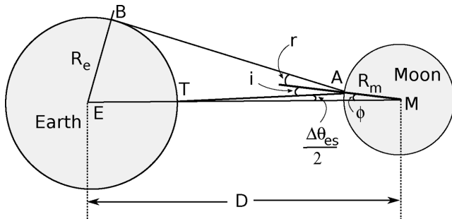
Figure C1. Not-to-scale schematic of the Earth-Moon geometry used in the calculation of the angular size of reflected earthshine.
