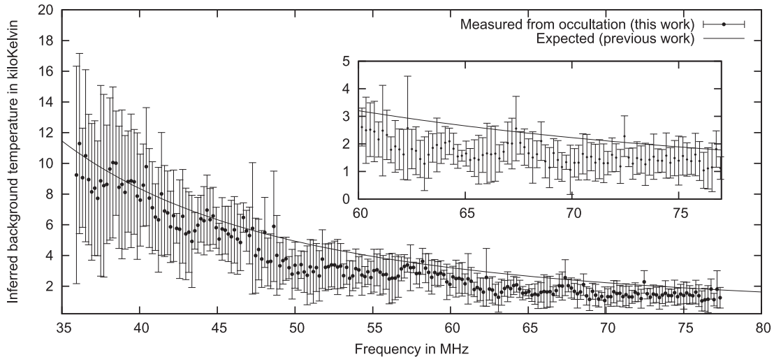
Figure 8. Plot showing the inferred background temperature occulted by the Moon. At each channel, we estimate seven background temperature values using seven one-hour synthesis images of the Moon. Plotted are the mean and standard deviation of the seven temperatures measured in each channel.
