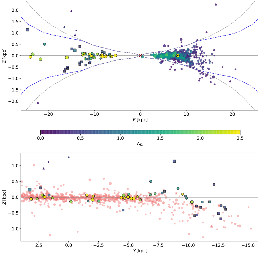
Fig. 4. Vertical distribution of our sample of far side disk CCs, compared to other well-known CCs from the literature. Top : galactocentric radius ( R ) versus Z distribution for CCs, color coded by their K_S extinctions, A_{K_S} . At positive R values, we plotted the CCs from Skowron et al. (2019a) that are on the near side of the Galactic disk, i.e., at X < 8.15 kpc (pentagons), while the CCs used in this work are shown at R < 0 (circles and squares are used as in Fig. 1). The sizes of the symbols are inversely proportional to the CC ages. The five CCs from Feast et al. (2014) are included here as a reference (triangles), as well as the flaring curve models from Kalberla et al. (2007), where the blue and gray dashed lines represent their S and N1 models, respectively. Bottom : projection of our CCs in Galactic Y versus Z coordinates. The whole sample of stars from Skowron et al. (2019b) with a period larger than five days is now plotted as background pink pentagons. The warped shape of the southern disk toward negative Z values is clear in this plot.
