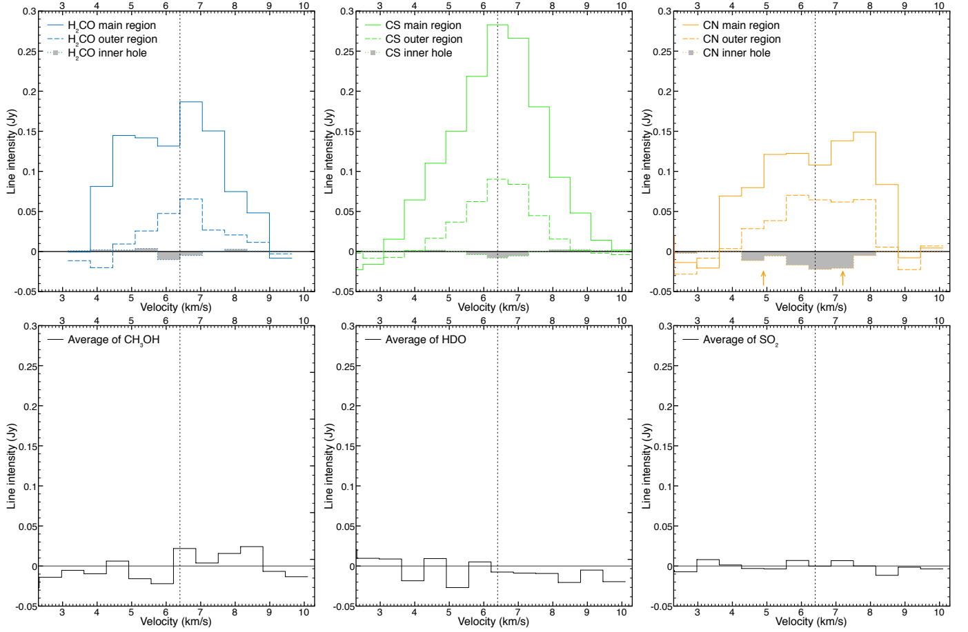
Fig. B.2. Spectral line profiles. Lines in the first row (detected) are integrated over three rings at different radii: 0'' – 0.2'' (the inner hole), 0.5'' – 2.0'' (the main region), and 3.5'' – 4.5'' (the outer region). The shaded region highlights the profile from the inner hole. Arrows on the CN line profile denote the presence of blended lines. For lines in the second row (undetected) only the profile over the main region is shown. For these lines, the profile is obtained by averaging all available lines for that species. The vertical line indicates the systemic velocity of the source ( 6.4 \text{ km s}^{-1} ).
