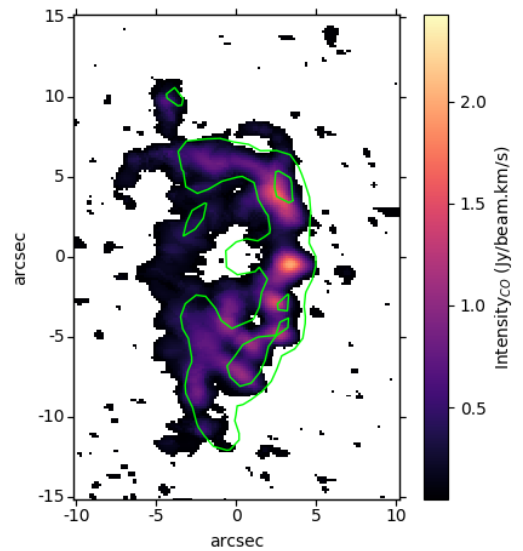
Figure 6. The CO J_{2-1} transition intensity map of JO201 in flux units of Jy/beam.Km/s. The green contour is taken from the NUV image shown in Fig 2. Note the cavity in CO map around the central AGN.
