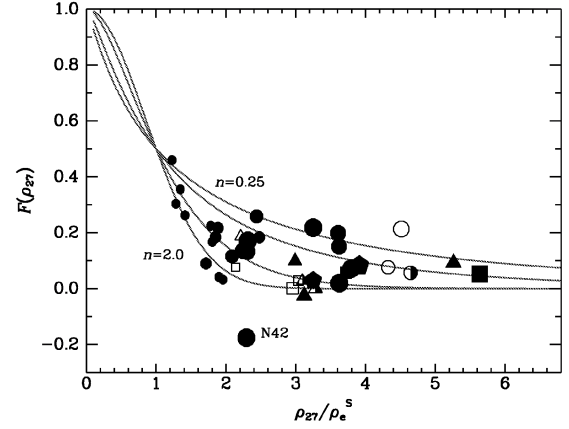
Figure 5. Fraction of galaxy light beyond the isophotal radius versus the ratio of isophotal to effective radius. Circles: E-dE; pentagons: S0-dS0; squares: Sa-Sc; triangles: Sd-Im. Filled symbols: definite members; open symbols: background objects; half-filled symbols: dubious cases. Symbol sizes are proportional to integrated magnitudes. Curves obtained from equation (1) are shown for n = 0.25 , n = 0.4 , n = 1 , and n = 2 . Note the outlier object (N42 in our catalogue) at F(\rho_{27}) = -0.18 , as discussed in the text.
