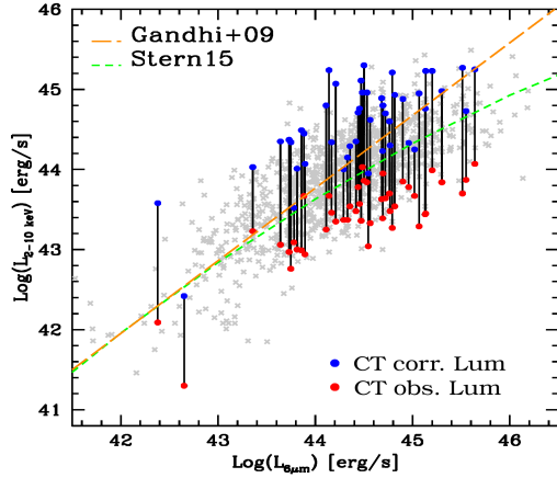
Fig. 3 Distribution of the AGN Mid-IR ( 6\mu m ) luminosity, as derived from SED fitting, after subtracting the host star-formation emission, and the 2-10 keV luminosity, for the \sim 2000 sources analyzed in Marchesi et al. 2016 (gray crosses). Red circles show the observed L_X for the CT candidates, while blue circles show the absorption-corrected L_X . The orange (green) curve shows the relation published in Gandhi et al. 2009 (Stern 2015).
