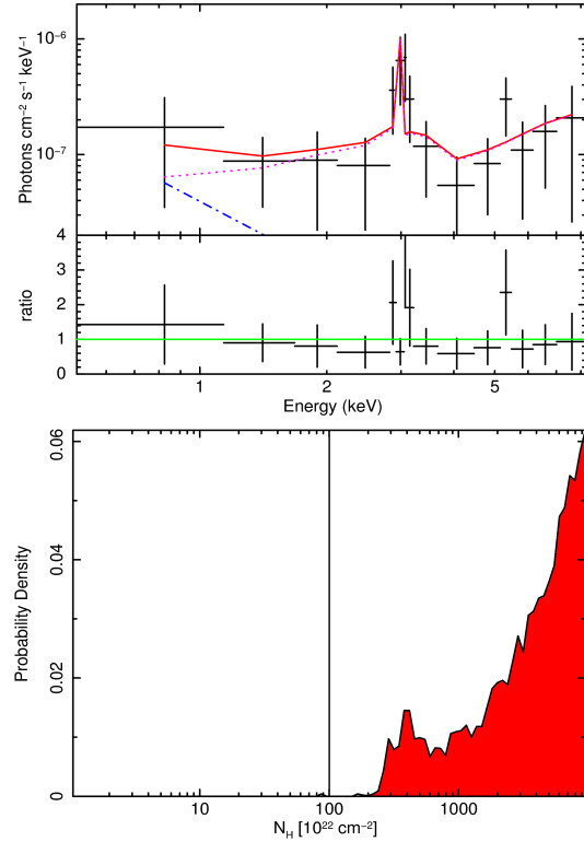
Fig. 6 As fig. 5, for source LID_390.
