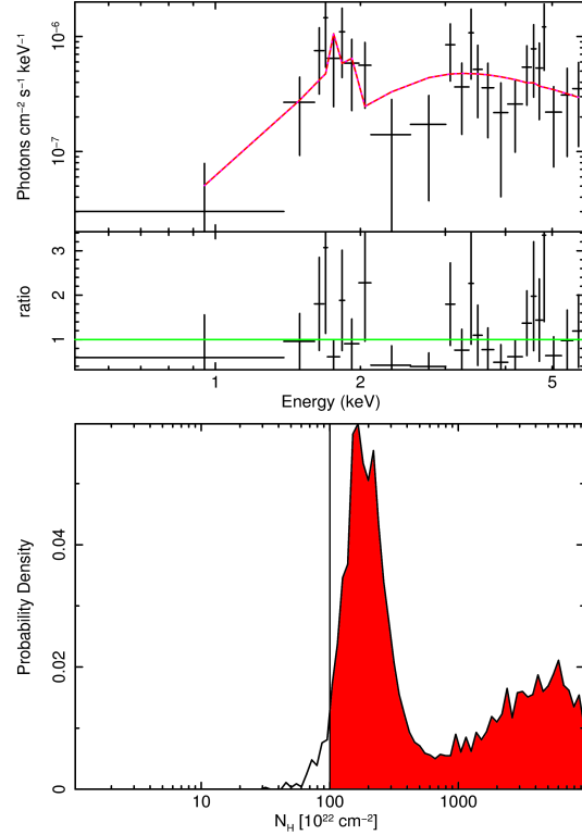
Fig. 2 Top: Unfolded spectrum and data-to-model ratio of the CT candidate LID_1002 at z = 2.612 . This source only required the BNtorus component. Bottom: PDF of N_H for the same source.
