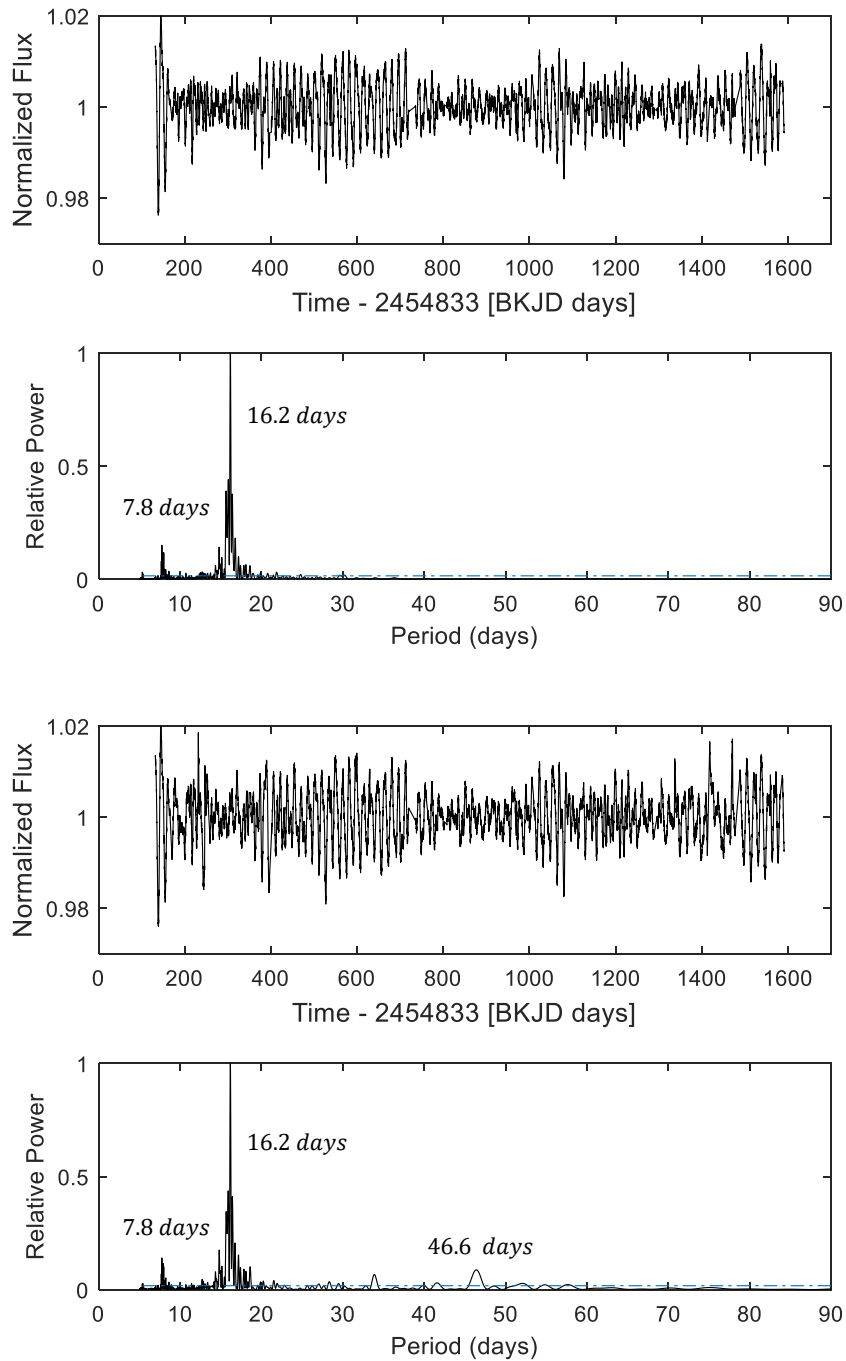
Fig. 5. Final PDC (first panel) and SAP (third panel) time series adjusted according to steps of Section 3. The Lomb-Scargle periodograms are on the bottom side correspondingly. The dashed-dot blue line is the significance threshold given by letting FAP (False Alarm Probability) equals to 10^{-4} . For SAP data, there is a significant peak to 46.6 days also found in Figure 6. As can be seen, the PDC timeseries has a flat periodogram for periods longer than 20 days confirming that the PDC pipeline tends to remove all the long-term trends.
