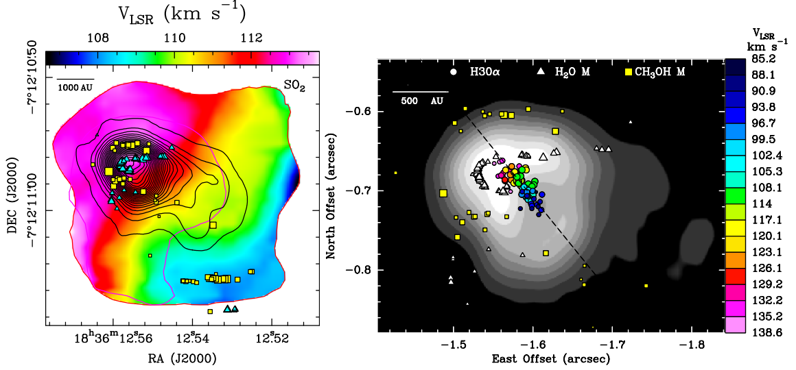
Figure 3: Left panel: The color map shows the intensity-averaged velocity of the \text{SO}_2 v=0 16(1,15)-15(2,14) transition in core A1. The black contours reproduce the JVL A-Array 1.3 cm continuum. The cyan triangles and yellow squares report the VLBI positions of the 22 GHz water and 6.7 GHz methanol masers, respectively. Right panel: The gray-scale image represents the VLA A-Array 7 mm continuum emission observed by [1]. The white triangles and yellow squares mark the VLBI positions of the \text{H}_2\text{O} 22 GHz and \text{CH}_3\text{OH} 6.7 GHz masers, respectively. The colored dots give the channel peak positions of the \text{H}30\alpha line emission, with colors denoting V_{\text{LSR}} as indicated in the wedge on the right of the plot. The dashed black line marks the axis of the spatial distribution of the \text{H}30\alpha peaks.
