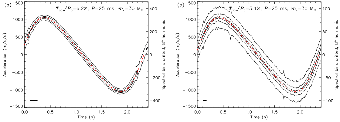
Figure 4: The effectiveness of acceleration searches in the detection of a simulated PSR-BH system. While such a system would be ideal for gravity tests, its detection through blind searches would be extremely challenging. Here we represent a “worst-case scenario”, where the pulsar has a short spin period of 25 ms; expected in systems that have formed via exchange interactions in dense stellar environments, or where the pulsar is the first-born object. The black hole mass is at the high end of what is expected for stellar mass black holes ( 30 M_{\odot} ), and the orbital period is small ( P_b = 2.4 hr) and has low eccentricity ( e = 0.1 ). To worsen matters the system is viewed edge-on, where the deleterious effects of line-of-sight motion are strongest. Contours mark the 30%, 60% and 90% pulsar signal recovery levels for constant acceleration searches of data integrations which are \sim 6\% and \sim 3\% of the orbital period (panels (a) and (b) respectively). Because a survey observation can start at any phase in the orbit, the starting point of the acceleration search has been incremented in steps of 50 s across the entire orbit. The thick black line shows the integration length analyzed. The red dashed line shows the true acceleration value at the mid-point of integration (Liu et al. in prep).
