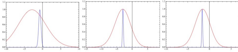
Fig. 5. Joint likelihood of \alpha for \Delta\ell = 2-6 in the left panel, \Delta\ell = 2-23 in the middle panel and \Delta\ell = 2-47 in the right panel. Red designates the WMAP data and blue the Planck forecast. See also the text.
