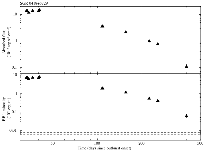
Figure D10. Left-hand panel: temporal evolution of the fluxes and luminosities for the BB model applied to the Swift XRT data of the outburst of SGR 0418+5729. The dashed lines mark the 1\sigma c.l. range for the quiescent luminosity (see Table 4). A distance of 2 kpc was assumed. Right-hand panel: temporal evolution of the bolometric luminosity with the best-fitting decay model superimposed.
