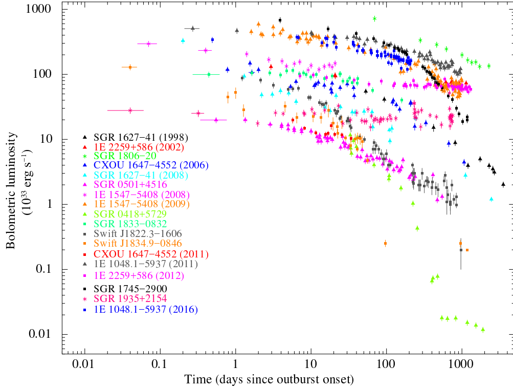
Figure 1. Temporal evolution of the bolometric (0.01–100 keV) luminosities for all outbursts re-analysed in this work. The distances assumed are those quoted in Table 5.
