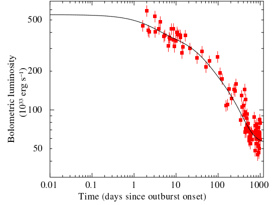
Figure D9. Left-hand panel: temporal evolution of the fluxes and luminosities for the BB+PL model applied to the Swift XRT data of the 2009 outburst of 1E 1547–5408. The dashed lines mark the 1\sigma c.l. range for the quiescent luminosity (see Table 4). A distance of 4.5 kpc was assumed. Right-hand panel: temporal evolution of the bolometric luminosity with the best-fitting decay model superimposed.
