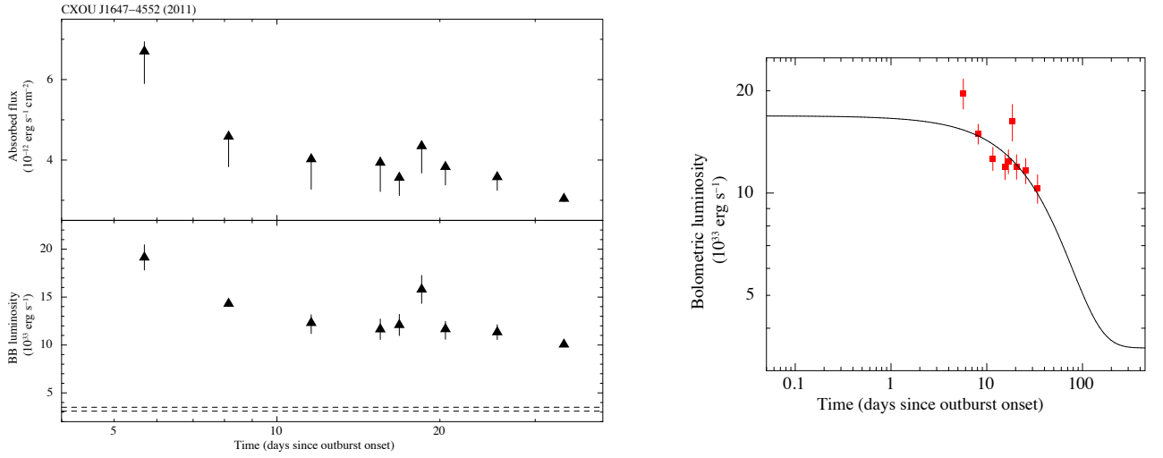
Figure D14. Left-hand panel: temporal evolution of the fluxes and luminosities for the BB model applied to the X-ray data of the 2011 outburst of CXOU J164710.2–455216. The dashed lines mark the 1\sigma c.l. range for the quiescent luminosity (see Table 4). A distance of 4 kpc was assumed. Right-hand panel: temporal evolution of the bolometric luminosity with the best-fitting decay model superimposed.
