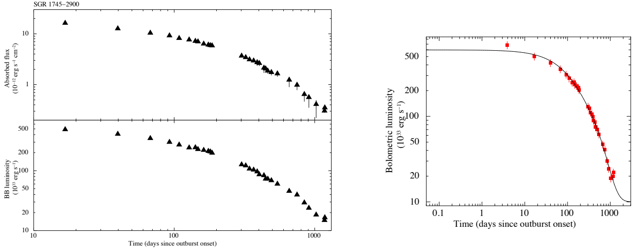
Figure D17. Left-hand panel: temporal evolution of the fluxes and luminosities for the BB+PL model applied to the Chandra data of the outburst of SGR 1745–2900. A distance of 8.3 kpc was assumed. Right-hand panel: temporal evolution of the bolometric luminosity with the best-fitting decay model superimposed.
