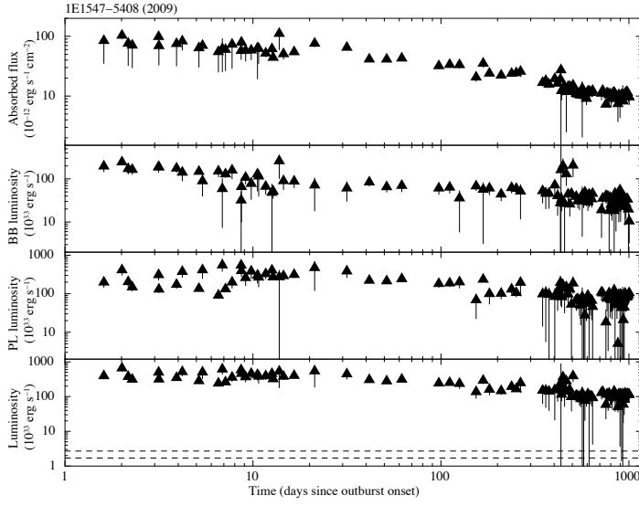
Figure D9. Left-hand panel: temporal evolution of the fluxes and luminosities for the BB+PL model applied to the Swift XRT data of the 2009 outburst of 1E 1547–5408. The dashed lines mark the 1\sigma c.l. range for the quiescent luminosity (see Table 4). A distance of 4.5 kpc was assumed. Right-hand panel: temporal evolution of the bolometric luminosity with the best-fitting decay model superimposed.
