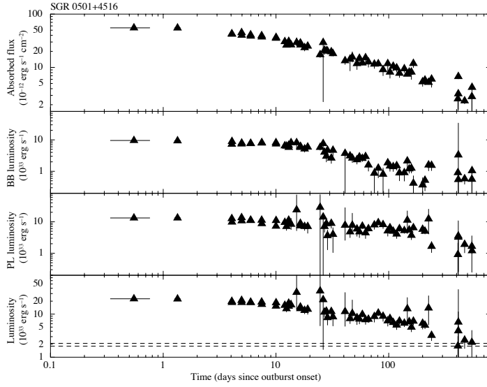
Figure D7. Left-hand panel: temporal evolution of the fluxes and luminosities for the BB+PL model applied to the Swift XRT data of SGR 0501+4516. The dashed line marks the approximate value for the quiescent luminosity (see Table 4). A distance of 1.5 kpc was assumed. Right-hand panel: temporal evolution of the bolometric luminosity with the best-fitting decay model superimposed.
