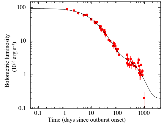
Figure D12. Left-hand panel: temporal evolution of the fluxes and luminosities for the BB+PL model applied to the outburst of Swift J1822.3–1606. The dashed line marks the value for the quiescent luminosity (see Table 4). A distance of 1.6 kpc was assumed. Right-hand panel: temporal evolution of the bolometric luminosity with the best-fitting decay model superimposed.
