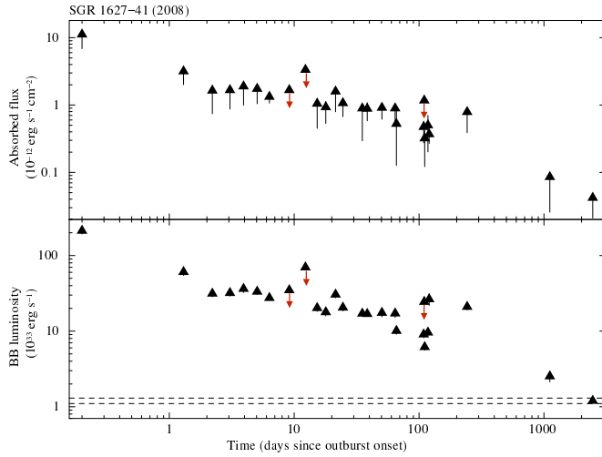
Figure D6. Left-hand panel: temporal evolution of the fluxes and luminosities for the BB model applied to the X-ray data of the 2008 outburst of SGR 1627–41. The dashed lines mark the 1\sigma c.l. range for the quiescent luminosity (see Table 4). The red downward arrowheads indicate the 3\sigma upper limits. A distance of 11 kpc was assumed. Right-hand panel: temporal evolution of the bolometric luminosity with the best-fitting decay model superimposed.
