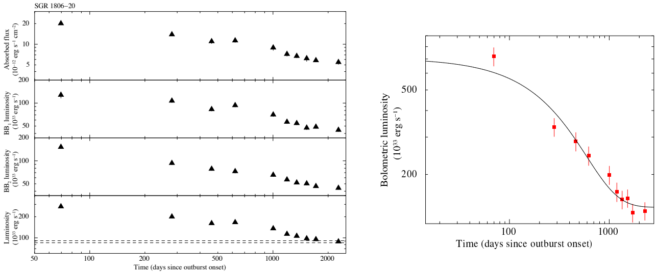
Figure D4. Left-hand panel: temporal evolution of the fluxes and luminosities for the 2BB model applied to the XMM-Newton data of SGR 1806–20. The dashed lines mark the 1\sigma c.l. range for the quiescent luminosity (see Table 4). A distance of 8.7 kpc was assumed. Right-hand panel: temporal evolution of the bolometric luminosity with the best-fitting decay model superimposed.
