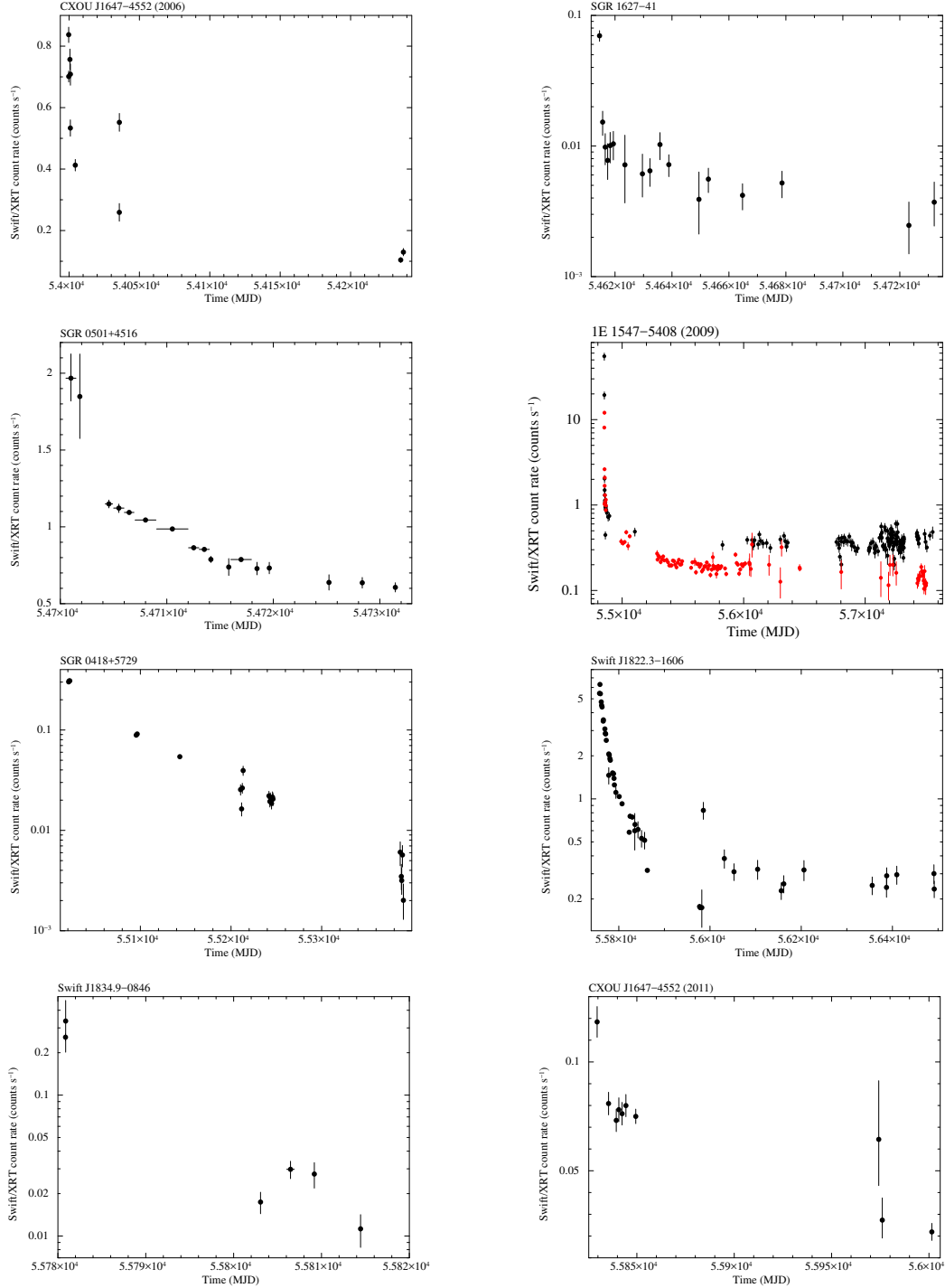
Figure B1. Swift XRT long-term 0.3–10 keV light curves of densely monitored magnetar outbursts, created using the online Swift XRT data products generator (Evans et al. 2009). In case both PC- and WT-mode data are available, black (red) dots refer to data acquired with the XRT set in WT (PC) mode.
