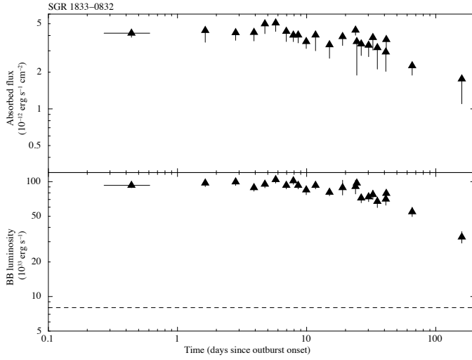
Figure D11. Left-hand panel: temporal evolution of the fluxes and luminosities for the BB+PL model applied to the Swift XRT data of the outburst of SGR 1833–0832. The dashed line marks the upper limit (at the 3\sigma c.l.) for the quiescent luminosity (see Table 4). A distance of 10 kpc was assumed. Right-hand panel: temporal evolution of the bolometric luminosity with the best-fitting decay model superimposed.
