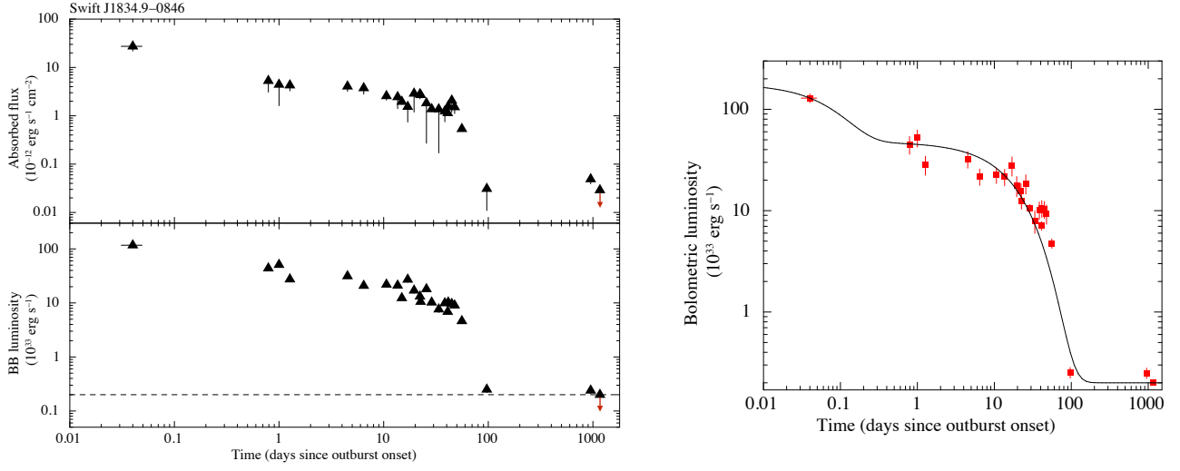
Figure D13. Left-hand panel: temporal evolution of the fluxes and luminosities for the BB model applied to the X-ray data of the outburst of Swift J1834.9–0846. The dashed line marks the upper limit (at the 3\sigma c.l.) for the quiescent luminosity (see Table 4). The red downward arrowheads indicate the 3\sigma upper limits. A distance of 4.2 kpc was assumed. Right-hand panel: temporal evolution of the bolometric luminosity with the best-fitting decay model superimposed.
