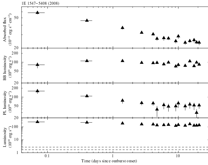
Figure D8. Left-hand panel: temporal evolution of the fluxes and luminosities for the BB+PL model applied to the Swift XRT data of the 2008 outburst of 1E 1547-5408. The dashed lines mark the 1\sigma c.i. range for the quiescent luminosity (see Table 4). A distance of 4.5 kpc was assumed. Right-hand panel: temporal evolution of the bolometric luminosity with the best-fitting decay model superimposed.
