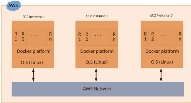
Figure 1. AWS EC2 method for the distribution of the workload: the cttools suite is containerized through a Docker in each instance. Each instance allows a large number of realizations to be run simultaneously.
