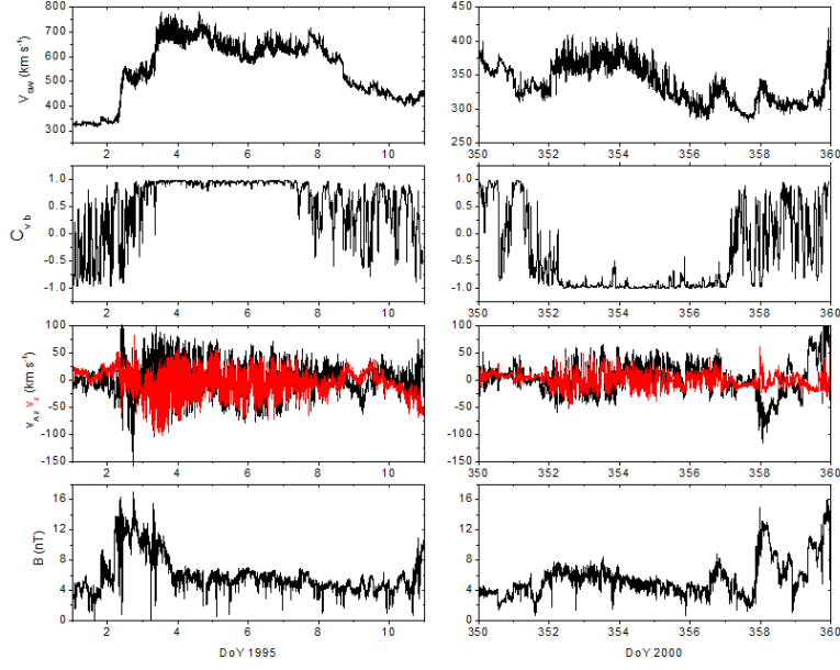
Figure 1. Summary plots for the time intervals extending from day 1 to 11 of year 1995 (solar minimum, left panels) and from day 350 to 360 of year 2000 (solar maximum, right panels): (from top to bottom) time series of solar wind bulk speed ( V_{sw} ), v-b correlation coefficient computed at 1 h scale ( C_{vb} ), (red) the z component of velocity ( v_z ) and (black) the z component of the magnetic field in Alfvén units ( v_{Az} ) in GSE, magnetic field magnitude ( B ).
