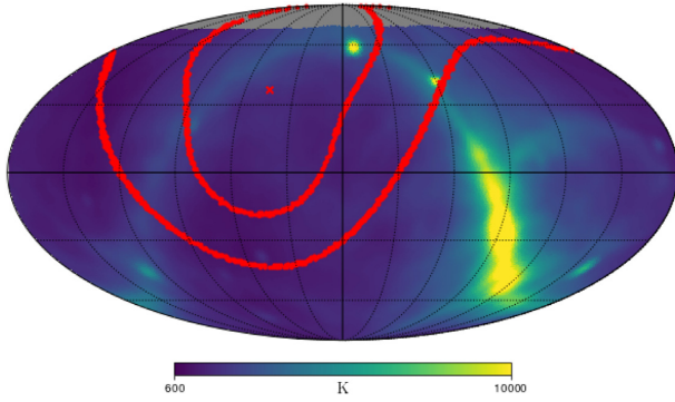
Figure 6. Red contours show -3\text{dB} and -10\text{dB} projection, in celestial coordinates, of the E–W oriented LEDA antenna model at 75 MHz, for LST=3. The Guzman 45 MHz map scaled at 75 MHz with a constant spectral index of -2.5 is shown in the background for illustration purposes. The grey area shows the missing data at \rho > 65^\circ . As the sky drifts the antenna is seeing different structures at the different LSTs.
