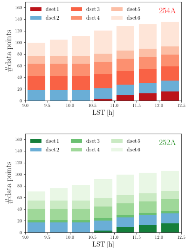
Figure A1. Total number of data points for each frequency in LST slots of \sim 0.5 h in the preferred 9–12.5 h LST range, for antenna 254A (top panel) and antenna 252A (bottom panel). We highlight how they are distributed between the different data sets following the same colour code of Fig. 5.
