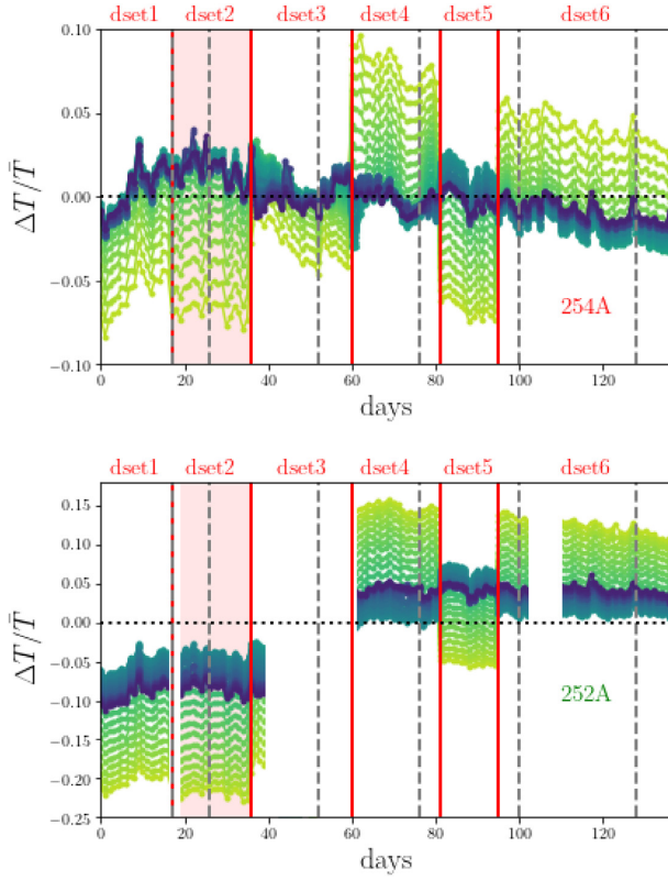
Figure 4. Variations of the measured sky temperature T_d(\nu) , for 1-h integration time around LST = 12h, as a function of observing day (d), for antenna 254A (upper panel) and 252A (lower panel). We plot the relative difference between T_d(\nu) and its mean value \bar{T} (equation 1). Different colours indicate different frequencies: lower (higher) frequencies are shown in lighter greens (darker blues). Dashed vertical lines denote the separation between months. 2018 May appears at the beginning of the x-axis (note the dashed line superimposing with the first red vertical line), followed by 2018 December up to 2019 May. Note that observations do not span all days of every month, therefore the number of days between two consecutive vertical dashed lines is smaller than 30. The relative temperature shows time discontinuities common to both antennas, more pronounced at low frequencies. These are highlighted in the plot with red vertical lines and define the six different data sets . 2018 December and 2019 January data (dset2), marked as a red shaded region, constitute our reference data set as they are optimal in terms of soil condition. Note that, despite a less prominent discontinuity, we keep 2018 May separated from 2018 December 2018.
