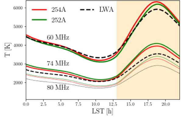
Figure 9. Comparison between the reference data set mean sky temperature as a function of LST (antenna 254A in red and 252A green) with the average values of the LWA maps from Dowell et al. (2017) weighted by antenna response (equation 8) at 60, 74, and 80 MHz (black dashed lines with decreasing thickness). For illustrative purposes, the light yellow shaded area indicates the daylight time for LEDA observations, starting approximately at sunrise.
