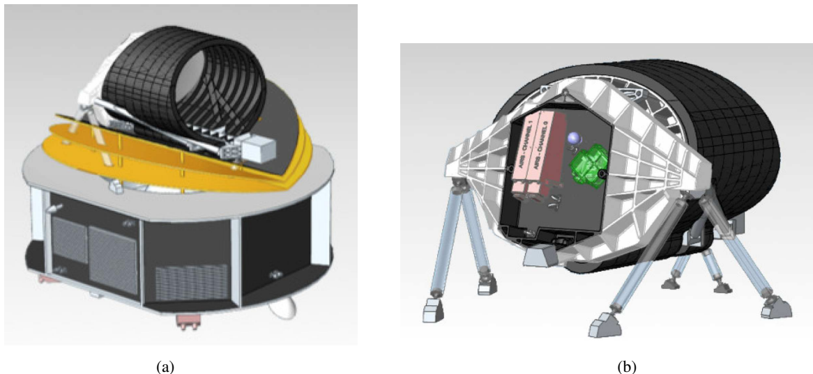
Figure 1. In (a) ARIEL mechanical layout including the warm service module at the bottom and the cold telescope plus instrument unit at the top. In yellow the V-Grooves. In (b) mechanical design of the OB with highlighted in green the FGS and in pink the AIRS modules.
