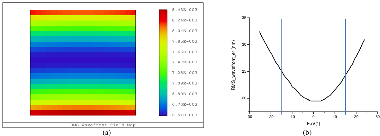
Figure 4. In (a) RMS wavefront error field map calculated for the 3\ \mu\text{m} wavelength over the 30" nominal telescope FoV. Units are \lambda . In (b) cross section along the Y direction of the RMS wavefront error expressed in nm; in the X direction the wavefront error is constant.
