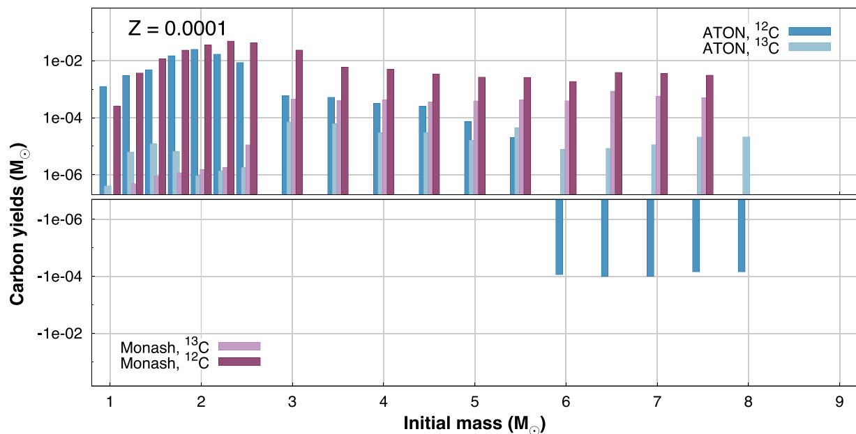
Figure 7. Net yields of ^{12}\text{C} and ^{13}\text{C} from LIMS and super-AGB stars after Ventura et al. (2013), in shades of blue, and Karakas (2010) and Doherty et al. (2014a, b), in shades of purple, for Z = 0.0001 . A negative yield means the element is destroyed, rather than produced, in the star.
