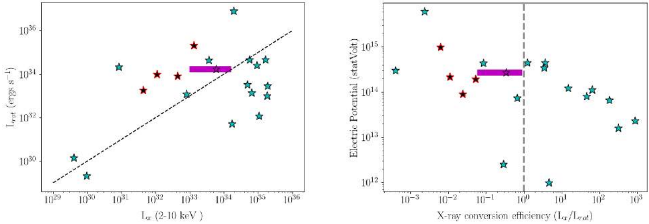
Figure 5. Left-hand panel: spin-down luminosity versus quiescent 2–10 keV X-ray luminosity of magnetars. The black dashed line represents the region where L_x = L_{\text{rot}} . Right-hand panel: electric potential in the magnetosphere as a function of X-ray conversion efficiency. The grey dashed line corresponds to an efficiency of 1. For both plots, cyan stars represent the magnetar population taken from the McGill Magnetar Catalogue (Olausen & Kaspi 2014). The black stars with red outlines represent radio loud magnetars, while SGR J1935+2154 is shown as the magenta star. The shaded region represents the range of values L_x and conversion efficiency based on the distance to the magnetar (see the text for more details). The position of the magenta star corresponds to the distance of 6.6 kpc as used in Borghese et al. (2020a).
