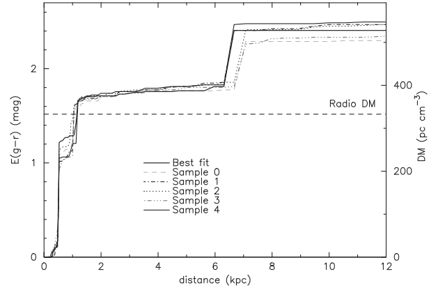
Figure 6. Colour-excess E(g-r) (left-hand axis) and dispersion measure (DM, right-hand axis) as a function of distance, derived from optical data, for the position of SGR J1935+2154, as extracted from the data of Green et al. (2019). Thin lines show the various sample data sets and the thick lines the best fit from Green et al. (2019). To calculate the dispersion measure, equation (5) has been used.
