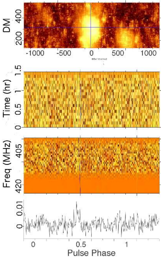
Figure 4. A radio pulse detected during observations of SGR J1935+2154 with the NC (obtained on 2020 May 30). From the bottom to top, the plots show the best integrated pulse profile (vertical axis is in arbitrary units); a waterfall plot of the frequency subbands versus pulse phase (the lighter the colour, the stronger the signal); a waterfall plot of time subintegrations (5 min each) versus pulse phase; and a colour scale showing the S/N of the integrated pulse profile in function of the spin period and dispersion measure (brighter colors correspond to higher values). The values of P and DM maximizing the S/N and corresponding to the bottom profiles are reported in the text. The optimized value of P is inconsistent with that derived from an ephemeris generated from NICER data.
