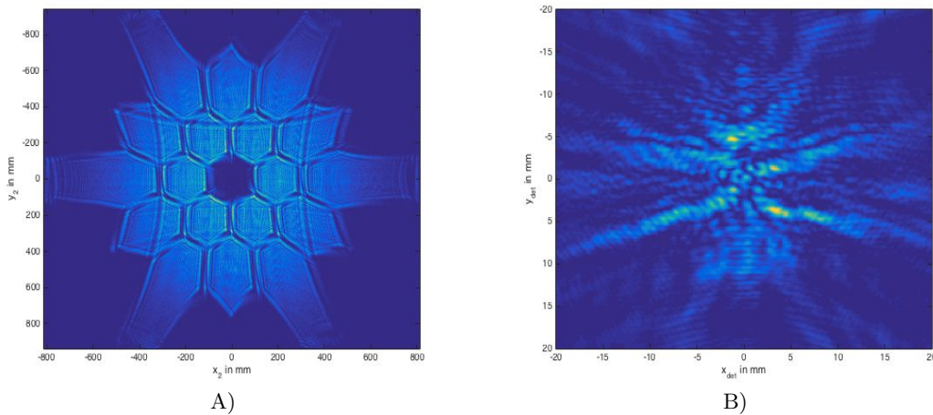
Figure 13. Simulated image of a source on axis located 10 km away from the ASTRI-M1 fully illuminating the pupil at a wavelength of 100\text{ }\mu\text{m} for accounting for M1 figure errors A) Reflection from ASTRI-M1 in the plane of ASTRI secondary mirror M2. B) 2^{nd} reflection from ASTRI-M2 in the plane of the detector.
