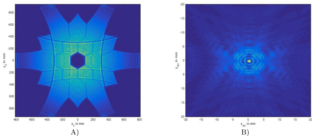
Figure 11. Simulated image of a source on axis located 10 km (a typical height of Cherenkov flashes) away from the ASTRI-M1 fully illuminating the pupil at a wavelength of 100\ \mu\text{m} . A) Reflection from ASTRI-M1 in the plane of ASTRI secondary mirror M2. B) 2^{\text{nd}} reflection from ASTRI-M2 in the detector plane.
