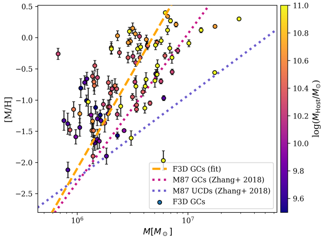
Fig. 6. MZR for the F3D GCs in comparison to the MZR for GCs and UCDs in M87 (pink and purple dotted lines, respectively, Zhang et al. 2018). The least-square fit to our data is shown in orange. The F3D GCs are colour-coded by the stellar mass of their host.
