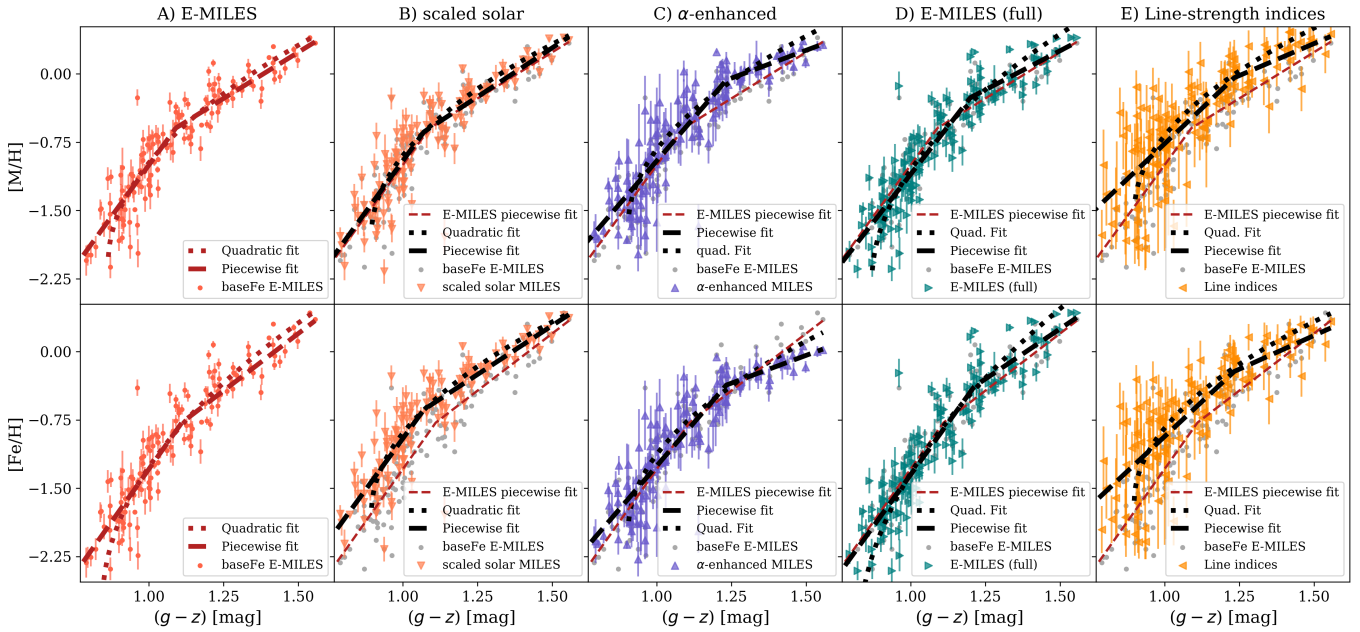
Fig. A.1. CZR for different metallicity measurement approaches (listed in Table A.1) based on total metallicities (top) and iron metallicities (bottom). From left to right: CZR using the E-MILES library with age constraint \geq 8 Gyr (method A), scaled-solar MILES models (method B), \alpha -enhanced MILES models (method C), E-MILES models without age constraint (method D), and line-strength indices (method E). The grey symbols show the points from method A as reference, and the lines show the respective fits. The best-fitting parameters are found in Table A.2.
