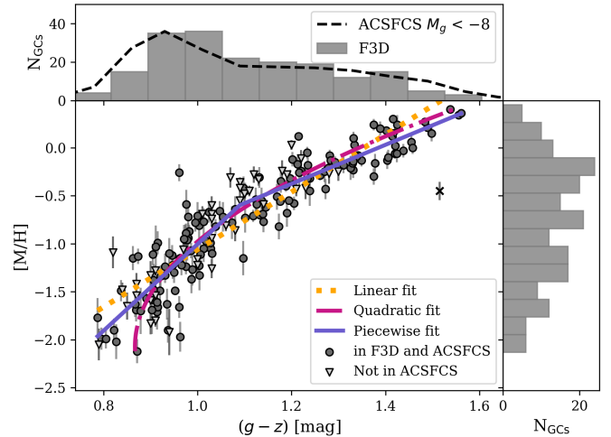
Fig. 1. Colour-metallicity distribution of F3D GCs. Spectroscopic GC metallicities from full spectral fitting versus (g - z) colour. Filled circles and triangles refer to GCs with and without ACSFCS (g - z) colours from Jordán et al. (2015), respectively. For the latter, we obtained the colour from the MUSE spectrum directly. The orange, pink and purple lines give the fit using the linear, quadratic or piecewise function (Eqs. (1)–(3)). The corresponding residuals are found in Fig. 2. As described in the text, we excluded an outlier from the fit marked by a cross. Separate distributions of colour and metallicities are shown on the top and the right-hand side. Top panel: we included the histogram from the full ACSFCS GC sample after applying a magnitude cut corresponding to our sample.
