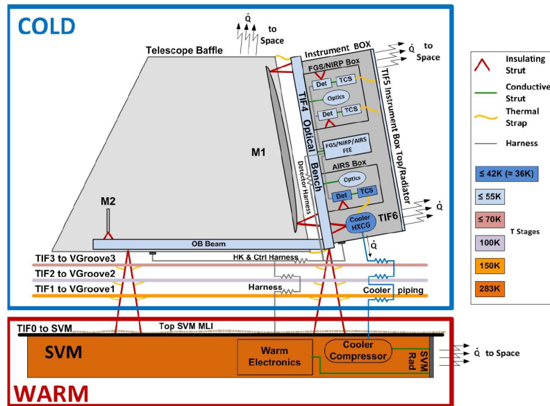
Figure 5. PLM thermal architecture scheme.
