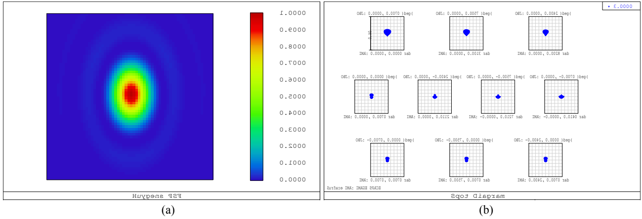
Figure 3. In (a) PSF calculated at the telescope FoV centre for a wavelength of 3 μm depicted over a 1 mrad square box. In (b) Spot Diagrams in the afocal space; the scale (box) is 0.4 mrad.
