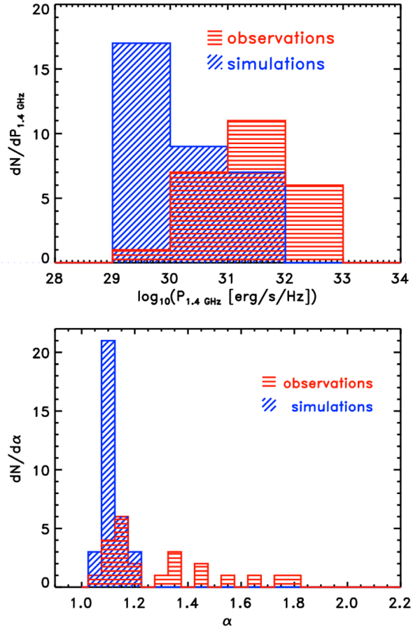
Figure 4. 3D analysis: Comparison of the distributions of the radio power (top) and the integrated spectral indices (bottom). The blue histograms present the data taken from the simulations and the red histograms show the observations, see Table 1.
