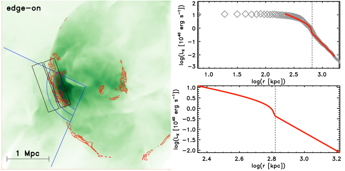
Figure 6. 3D analysis: Extraction of the X-ray surface brightness profile. The left-hand panel shows the map of the spectroscopic temperature overplotted with the radio contours at 1.4 GHz, [10^{25}, 10^{26}, \dots, 10^{30} \text{ erg s}^{-1} \text{ Hz}^{-1} \text{ pixel}^{-1}] . The black rectangles mark the regions in which the temperature jump was estimated. The blue solid lines show the shape of the circular annuli used to derive the X-ray surface brightness profile. On the right, the top panel shows the surface brightness profile extracted from the cluster centre beyond the relic. The red solid line marks the region of the fit that was used to estimate the density jump-based X-ray Mach number. The bottom panel shows the fitted profile across the relic. In both panels, the vertical line is the estimated position of the relic's outer edge.
