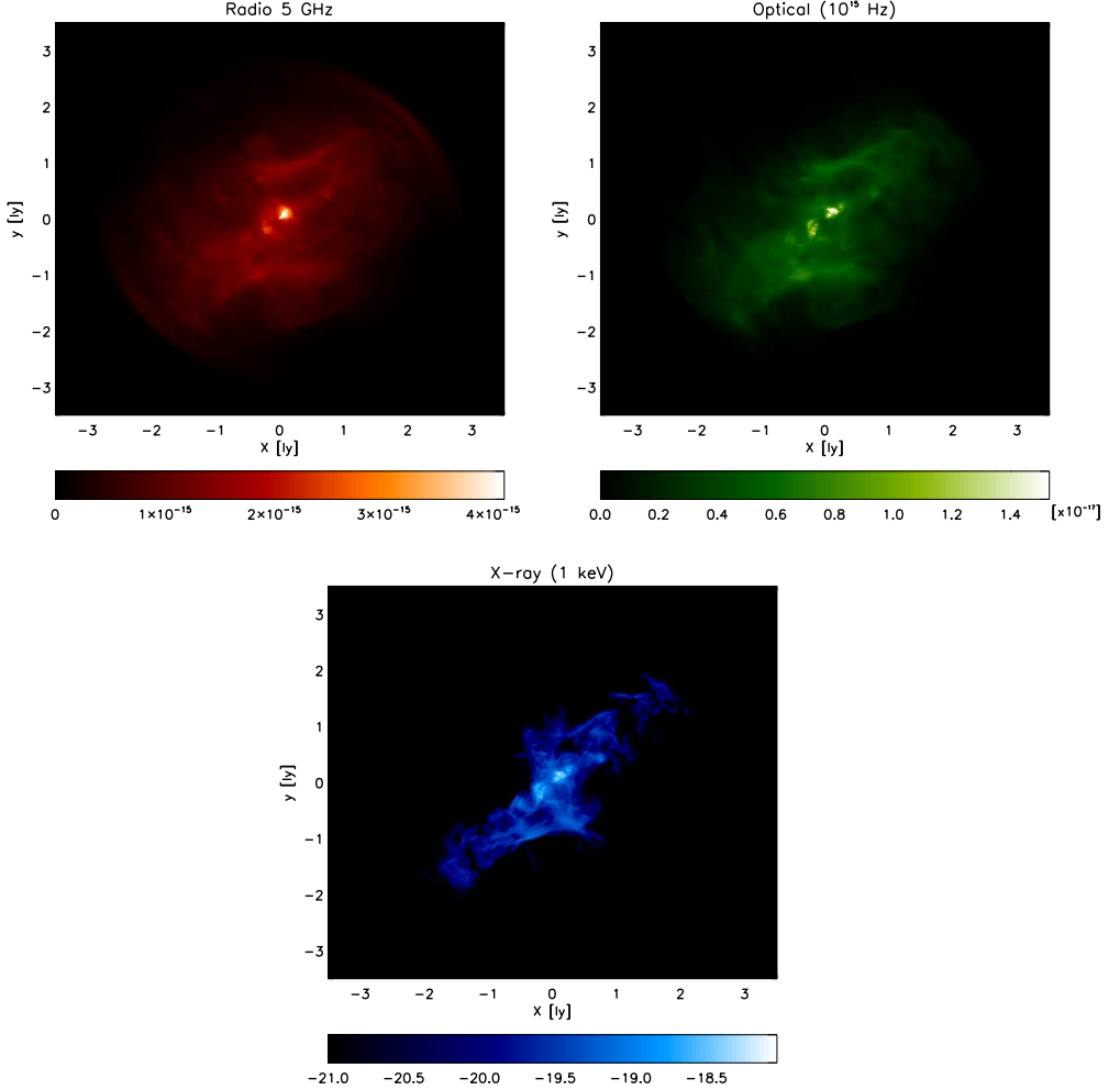
FIGURE 10. Left panel, top row: Map of the radio surface brightness at 5 GHz ( t = 250 yr, corresponding to the evolution time t_{\text{eq}} \simeq 500 yr). Intensity is indicated by the color bar, in linear scale. Right panel, top row: Linear map of the optical surface brightness at 10^{15} Hz ( t_{\text{sim}} = 250 yr, t_{\text{eq}} \simeq 500 yr). Bottom row: Map of the emission at X-rays (1 keV). In all the maps the intensity is expressed in \text{mJy/arcsec}^2 units and distance from the pulsar is in ly.
