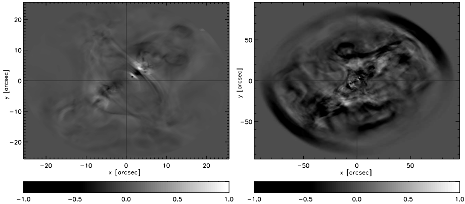
FIGURE 11. Map of the wisp-like structures at radio frequencies (5 GHz) in the inner nebula (left panel) and in the whole nebula (right panel). The images are obtained as the difference between two surface brightness maps separated by a time interval of 5 years around t=250 years. The position of the pulsar is identified by the black crosses and intensity is normalized to its maximum.
