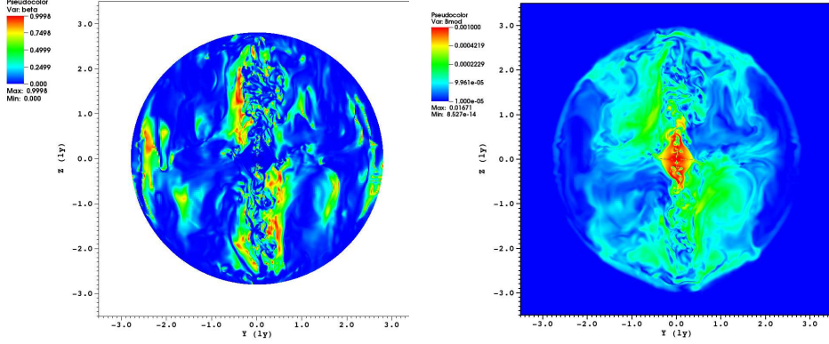
FIGURE 8. Left panel : The ratio of the polar to the total magnetic field magnitude in a 2D slice of the data cube at t=250 yr. Data are also cropped within a circle of radius equal to the nebular radius (2.8 ly) for ease of interpretation. As expected, the polar component is mostly important near the polar jets. Right panel : image of the 2D distribution of the total magnetic field magnitude in the 0, y, z plane, shown in units of Gauss at the time 250 yr. The magnetic field appears to be stronger close to the TS, where the mean value is around 1 mG.
