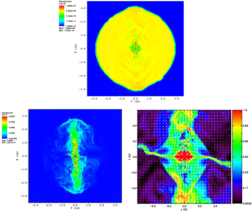
FIGURE 9. Upper row : 2D map of the particle pressure distribution, with intensity varying according to the color (logarithmic) scale. Left panel, bottom row : Magnitude of the velocity field in a 2D slice at t=250 yr. Right panel, bottom row : blow-up of the inner nebula in a plot of the velocity magnitude with arrows indicating the velocity field. Effects of the hoop stresses, guiding the flow in the polar direction to form jets, are clearly visible.
