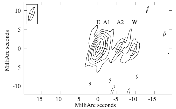
Fig. 3. VLBA image of IRAS 17020+4544 on the combined dataset from the 2000 June and August observations at 5 GHz, with contours traced at (-1, 1, 2, 4, \dots, 32) \times the \sim 3\sigma noise level, which is 0.27 mJy beam ^{-1} . The half peak beam width is shown in the upper left corner and it is 3.8 mas \times 1.2 mas in PA -21^\circ . Crosses and letters indicate and label model-fit elliptical Gaussian components.
