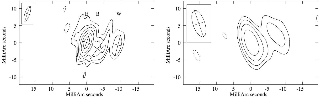
Fig. 1. VLBA images of IRAS 17020+4544 on 2014 February 12 at 5 GHz (left panel) and 8.4 GHz (right panel), with contours traced at (-1, 1, 2, 4, \dots, 32) \times the \sim 3\sigma noise level, which is 0.2 and 0.6 mJy beam ^{-1} at 5 and 8 GHz, respectively. The half peak beam width is shown in the upper left corner of each panel, and is 4.6 mas \times 1.4 mas in position angle (PA) -19^\circ and 8.0 mas \times 3.4 mas in PA 19^\circ at 5 and 8 GHz, respectively. Note the unusually larger beam at 8 GHz, due to the lack of fringe detections on the longest baselines at this frequency. In the 5 GHz image, model-fit elliptical Gaussian components are shown as crosses and labelled E, B, W, from east to west.
