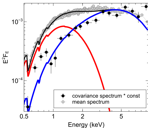
Figure 4. The covariance spectrum (black) computed over the frequencies [1 - 5] \times 10^{-4} Hz, compared to the time-integrated energy spectrum (gray; same as Fig. 1). The covariance spectrum (i.e. the spectrum of the emission that is linearly correlated to the broad 0.3–10 keV reference band) has been scaled by an arbitrary factor of 3 in order to more clearly compare the shapes of these two spectra. The covariance spectrum is much harder than the time-integrated spectrum, and follows the shape of the hotter disk blackbody component (blue), and not the lower temperature component (red).
