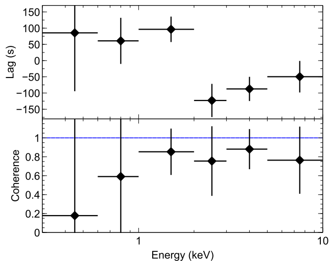
Figure 3. The lag-energy spectrum ( top ) and coherence spectrum ( bottom ) averaged over the frequency range from [1 - 5] \times 10^{-4} Hz. By convention, the larger the lag, the more delayed the energy bin. The coherence is best constrained above 1 keV.
