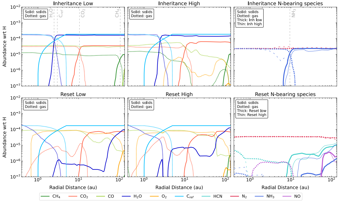
Figure 2. Radial profiles of molecular abundances of the key volatile C-, O-, and N-bearing species with respect to total H atoms. The profiles are taken from Eistrup et al. (2016) and properly rescaled to account for the different disks and the different compositional models considered in this work. In all panels, solid and dotted lines indicate the solid and gas phases, respectively. The top three panels describe the two inheritance scenarios, while the bottom three ones describe the two reset scenarios. The left-hand and central panels show the abundances of the key volatile molecules carrying C and O, including the contribution of refractory organic carbon ( C_{\text{ref}} ). N-bearing molecules are shown in the two right-hand panels for visual ease. Here, the low (SLRs only) and high (SLRs and CRs) ionization levels are shown in the same plot by means of thick and thin lines, respectively. The gray, dashed, vertical lines in the plots of the inheritance low scenario indicate the position of the snowlines of \text{H}_2\text{O} (2.5 au), C_{\text{ref}} (3 au), \text{NH}_3 (9.4 au), \text{CO}_2 (10.5 au), and \text{CH}_4 (105 au). CO and \text{N}_2 condense beyond 130 au in our model, and their snowlines are therefore not seen. Snowlines are omitted in the other scenarios, as the complexity of the chemistry requires the introduction of multiple snowlines.
