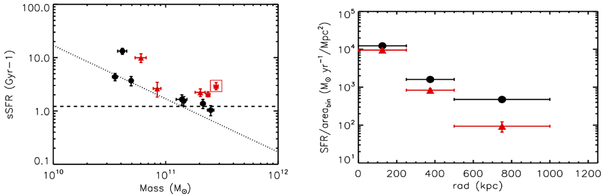
Figure 3. Left: sSFR versus stellar mass of the spectroscopic members (red triangles) and photometric redshift candidates (black circles) with Herschel emission, in the galaxy cluster XDCP0044. The dashed line indicates the expected main-sequence level of galaxies at the cluster redshift and the dotted line marks the 3\sigma detection limit of our Herschel data. The square indicates galaxy ID 95. Right: differential SFR divided by bin area versus projected radius of the spectroscopic members only (red) and adding the photo- z candidates (black).
