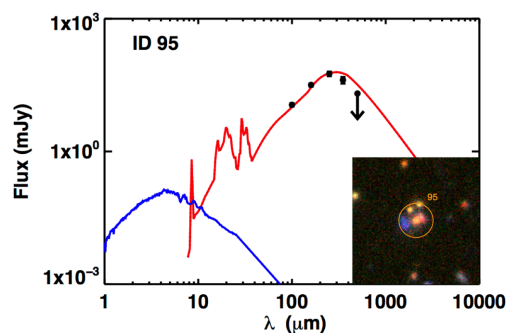
Figure 2. Best-fitting FIR SED (red line) of cluster member ID 95, with Ks/II inset (15 arcsec \times 15 arcsec). Data points are shown in black.
