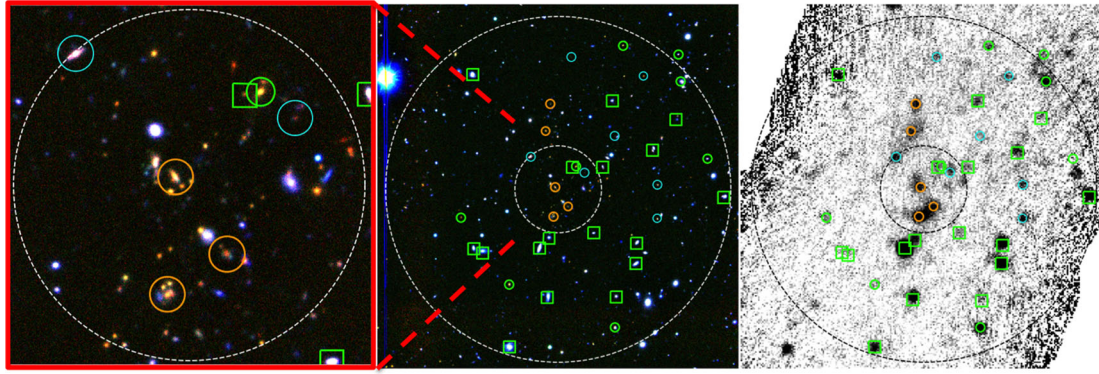
Figure 1. Ks/II colour composite of the central \sim 500 kpc (left) of the field of XDCP0044 (middle) and corresponding Herschel /PACS 100 \mu\text{m} map (right). Dashed circles have radii of 30 arcsec and 2 arcmin centred on the cluster X-ray centre. The five spectroscopic members with FIR emission are shown in orange circles, cyan regions indicate the photometric candidates with FIR emission and green regions correspond to spectroscopic (circles) and visual/photo- z (squares) interlopers.
