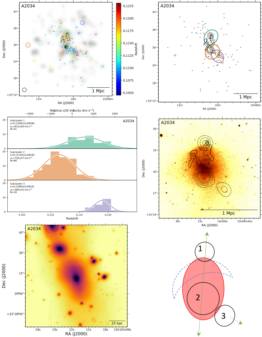
Figure 18. Top left: DS-test over red sequence R-band luminosity distribution with linearly spaced white contours. The black contours show the 1.4 GHz WSRT contours (van Weeren et al. 2011b). Top right: Subcluster membership of spectroscopic cluster members assigned with our GMM analysis. The same WSRT contours (solid) and red sequence luminosity contours (dashed) are depicted. Middle left: Subcluster redshift histograms with colors matching the image at the top right. Middle right: 261 ks Chandra image with the same WSRT radio contours (solid) and red sequence luminosity contours (dashed). The relics and disturbed ICM are suggestive of a merger between at least two subclusters; however, the lack of X-ray emission with subcluster 3 suggests it was also involved. Bottom left: 150 kpc cutout of the Subaru/SuprimeCam R-band image centered on the cluster BCG in subcluster 2. Bottom right: Proposed merger scenario. A2034 is primarily a north to south merger with two complications. First, the shock has been classified as a cold front in the literature, which would better explain subcluster 1's location; however, the relic candidate is coincident with this edge in the ICM. Second, subcluster 3 appears to have exited toward the southwest having its ICM stripped.
