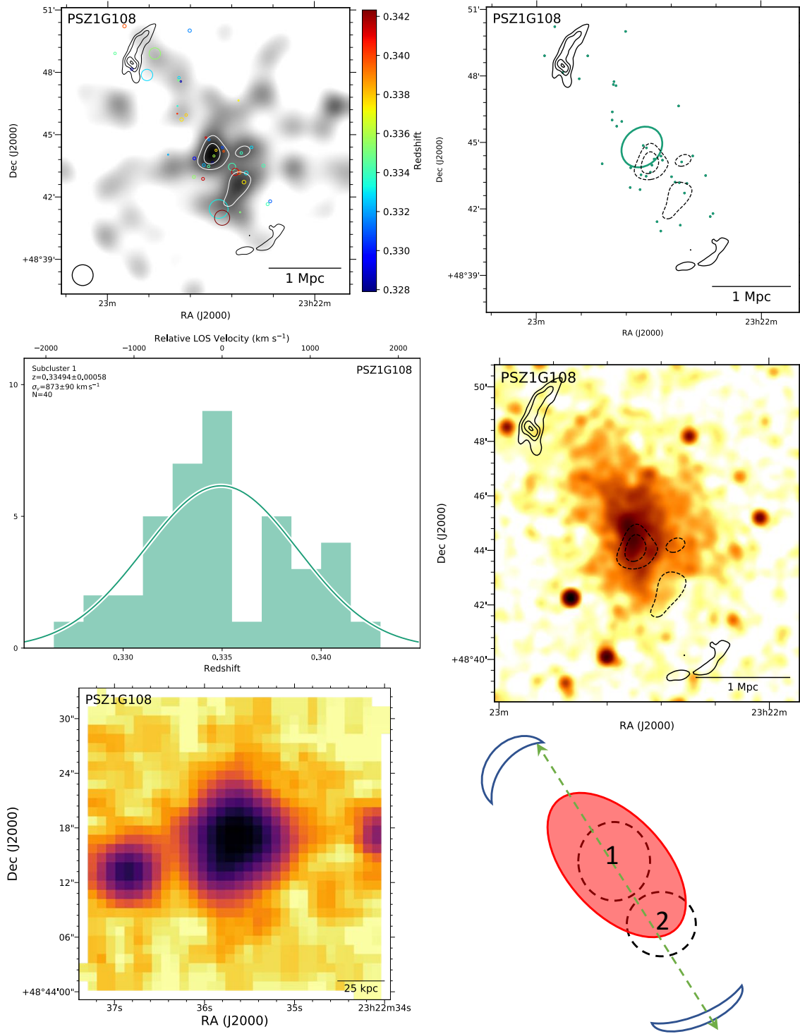
Figure 31. Top left: DS-test over red sequence DSS R-band luminosity distribution with linearly spaced white contours. The black contours show GMRT 323 GHz contours (de Gasperin et al. 2015). Top right: Subcluster membership of spectroscopic cluster members assigned with our GMM analysis. The same GMRT contours (solid) and red sequence luminosity contours (dashed) are depicted. Middle left: Subcluster redshift histogram with colors matching the image at the top right. Middle right: 27 ks Chandra image with the same GMRT radio contours (solid) and red sequence luminosity contours (dashed). Bottom left: 150 kpc cutout of the DSS R-band image centered on the cluster BCG. Bottom right: Preferred merger scenario. We do not have enough spectra to resolve composite structure, but the red sequence luminosity is multi-modal and aligned with the two radio relics and extended X-ray emission. Since the X-ray, radio, and optical light is all aligned, we propose a simple bimodal merger along this axis.
