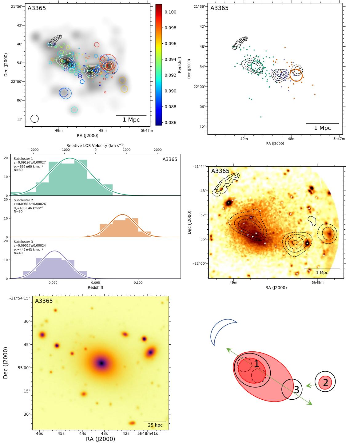
Figure 25. Top left: DS-test over red sequence Subaru/SuprimeCam r-band luminosity distribution with linearly space white contours. The black contours show the 1.4 GHz VLA contours (van Weeren et al. 2011b). Top right: Subcluster membership of spectroscopic cluster members assigned with our GMM analysis. The same VLA contours (solid) and red sequence luminosity contours (dashed) are depicted. Middle left: Subcluster redshift histogram with colors matching the image at the top right. Middle right: 161 ks XMM image with the same VLA radio contours (solid) and red sequence luminosity contours (dashed). Bottom left: 150 kpc cutout of the Subaru r-band image centered on the cluster BCG in subcluster 2. Bottom right: Preferred merger scenario. A3365 is composed of at least three subclusters with a merger occurring between subclusters 1 and 3 giving rise to the disturbed ICM and northeast relic. Subcluster 2 has a large line of sight velocity difference and undisturbed ICM suggesting it is still infalling with some component along the line of sight from the foreground, since it is redshifted relative to the rest of the cluster. There is evidence of composite structure in subcluster 1 which has two bright galaxies at either end of its associated red sequence luminosity peak as well as an elongated ridge of X-ray emission.
