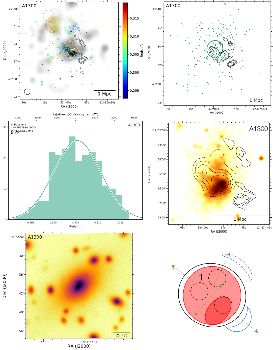
Figure 16. Top left: DS-test over red sequence r-band luminosity distribution with linearly space white contours. The black contours show the 325 MHz GMRT contours (Venturi et al. 2013). Top right: Subcluster membership of spectroscopic cluster members assigned with our GMM analysis. The same GMRT contours (solid) and red sequence luminosity contours (dashed) are depicted. The small projected separation and low spectroscopic survey density likely contributes to a single halo model being preferred by the BIC analysis. Middle left: Subcluster redshift histograms with colors matching the image at the top right. Middle right: 100 ks Chandra image with the same GMRT radio contours (solid) and red sequence luminosity contours (dashed). The relics and disturbed ICM are suggestive of a complex merger between at least three subclusters. Bottom left: 150 kpc cutout of the Subaru/SuprimeCam r-band image centered on the cluster BCG. Bottom right: Proposed merger scenario. A1300 is a difficult to interpret merger with likely at least three subclusters. The X-ray surface brightness morphology is suggestive of an additional merger axis associated with the an additional merger in the southwest to northeast direction. The BCG is elongated along the same axis. Inspection of the higher resolution HST RELICS images at https://www.spacetelescope.org/images/potw1745a/ show the BCG is actually composed of two luminosity peaks along this axis.
