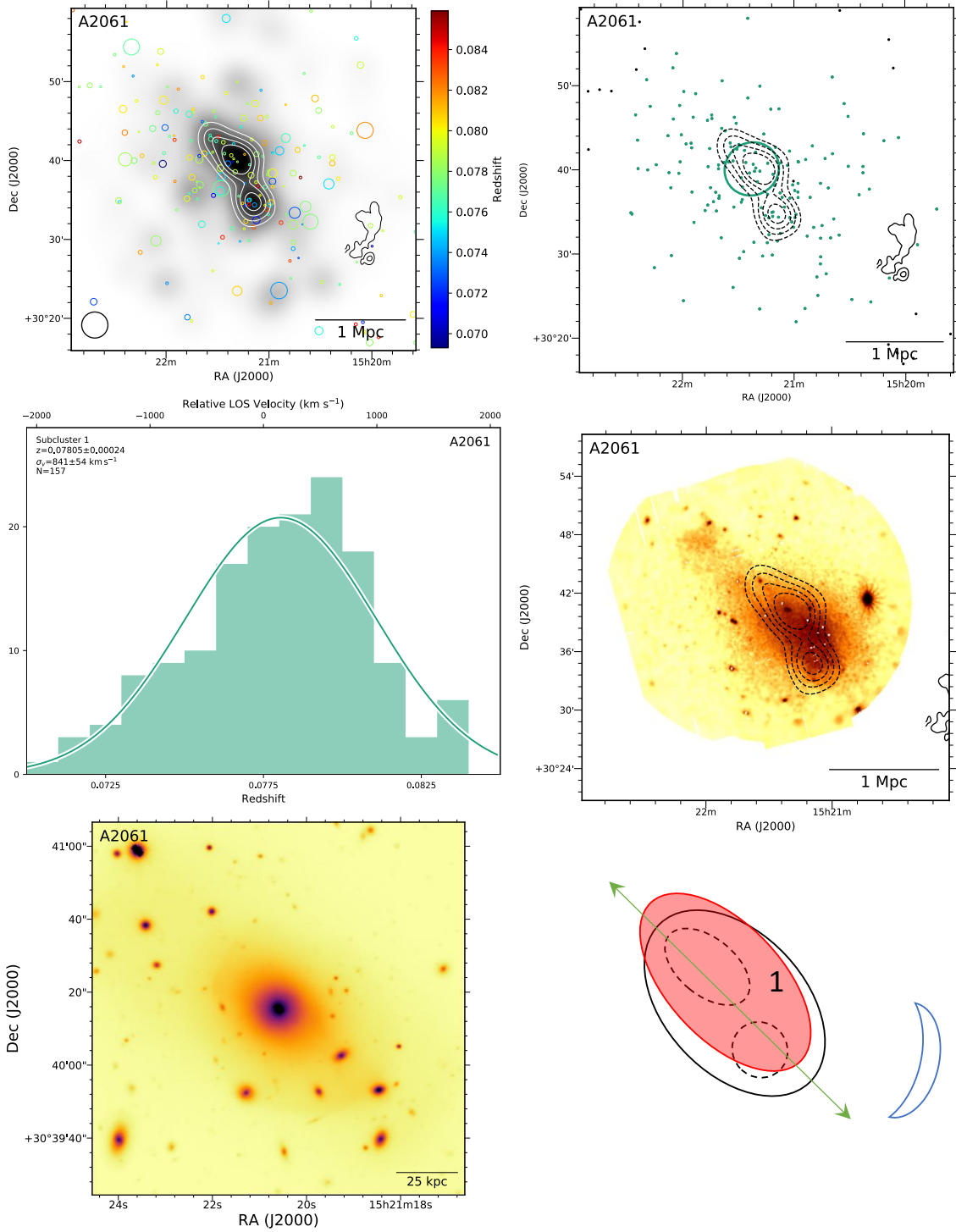
Figure 19. Top left: DS-test over red sequence r-band luminosity distribution with linearly space white contours. The black contours show the 1.4 GHz WSRT contours (van Weeren et al. 2011b). Top right: Subcluster membership of spectroscopic cluster members assigned with our GMM analysis. The same WSRT contours (solid) and red sequence luminosity contours (dashed) are depicted. The small projected separation and low spectroscopic survey density likely contributes to a single halo model being preferred by the BIC analysis. Middle left: Subcluster redshift histograms with colors matching the image at the top right. Middle right: 50 ks XMM image with the same WSRT radio contours (solid) and red sequence luminosity contours (dashed). The relic at the edge of the frame in the southwest and the disturbed ICM are suggestive of a merger between at least two subclusters. The extended stream of X-ray emission to the northeast toward A2067 is unlikely due to a merger between the two. A2067 sits 2.7 Mpc away. Bottom left: 150 kpc cutout of the Subaru/SuprimeCam r-band image centered on the cluster BCG in the southwest. Bottom right: Proposed merger scenario. Two subclusters are apparent in multiple wavelengths, but the GMM is unable to separate them due to low spectroscopic sampling and a small projected separation.
