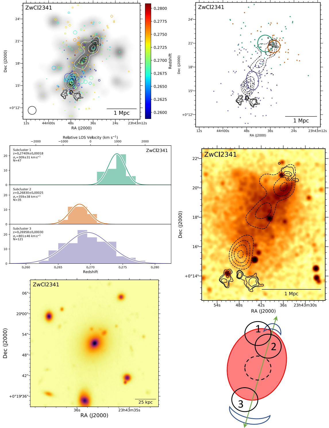
Figure 37. Top left: DS-test over red sequence Subaru/SuprimeCam r-band luminosity distribution with linearly space white contours. The black contours show GMRT 610 MHz contours (van Weeren et al. 2009b). Top right: Subcluster membership of spectroscopic cluster members assigned with our GMM analysis. The same WSRT contours (solid) and red sequence luminosity contours (dashed) are depicted. Middle left: Subcluster redshift histogram with colors matching the image at the top right. Middle right: 227 ks Chandra image with the same GMRT radio contours (solid) and red sequence luminosity contours (dashed). Bottom left: 150 kpc cutout of the Subaru r-band image centered on the cluster BCG in subcluster 1. Bottom right: Preferred merger scenario. We detect three subclusters with our GMM as well as a fourth that is evident in the red sequence luminosity distribution. Two subclusters (subclusters 2 and 3) and the candidate third situated in the middle of the cluster are aligned with the two radio relics. This suggests the dominant component of the merger is occurring along this axis with at least two subclusters partaking. Subcluster 1 is positioned to the east of subcluster 2, and is evident in both the X-ray surface brightness profile and red sequence luminosity. The disturbed gas suggests it has already merged, and the large line of sight velocity difference suggests line of sight motion.
