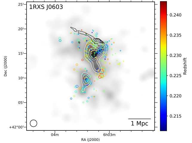
Figure 3. DS-test for 1RXSJ0603. The circles each correspond to spectroscopically confirmed cluster members and are colored according to their redshift. The size of the circles is given by 10^\delta . The gray scale map corresponds to the red sequence luminosity density smoothed by the optimal KDE bandwidth, and the corresponding white contours start at 3\sigma above the median pixel luminosity value and increase in units of \sigma , where \sigma is the standard deviation of the pixel values within R_{200} . The smoothing scale is chosen with an optical KDE bandwidth estimation, and is displayed in the lower left. The black contours are linearly spaced and show the so-called “Toothbrush” radio relic based upon the 610 MHz WSRT image of van Weeren et al. (2012b). The field is 2R_{200} \times 2R_{200} based on the global velocity dispersion and scaling relations (Evrard et al. 2008).
