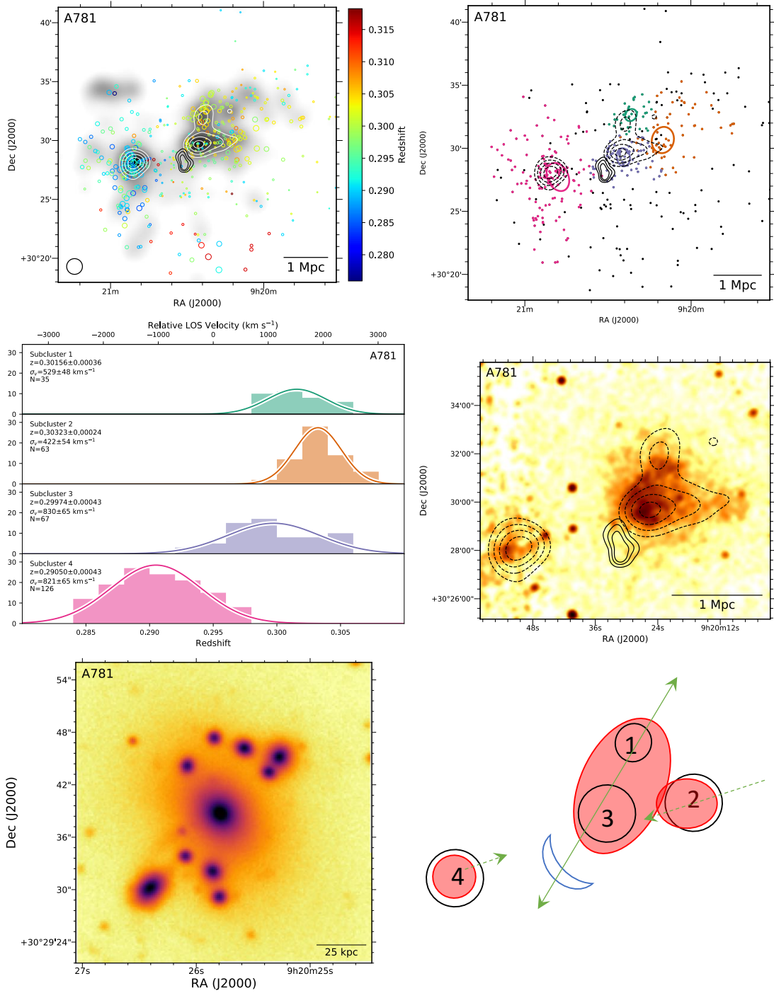
Figure 14. Top left: DS-test over red sequence i-band luminosity distribution with linearly space white contours. The black contours show the 325 MHz GMRT contours (Venturi et al. 2013). Top right: Subcluster membership of spectroscopic cluster members assigned with our GMM analysis. The same GMRT contours (solid) and red sequence luminosity contours (dashed) are depicted. Middle left: Subcluster redshift histograms with colors matching the image at the top right. Middle right: 48 ks Chandra image with the same WSRT radio contours (solid) and red sequence luminosity contours (dashed). The relic and disturbed ICM are suggestive of a merger between subclusters 1 and 3. Bottom left: 150 kpc cutout of the Subaru/SuprimeCam i-band image centered on the cluster BCG, which is associated with subcluster 3. Bottom right: Proposed merger scenario. The ICM is most disrupted between subclusters 1 and 3 with subcluster 2 having a less disturbed ICM coincident with its galactic light. Subcluster 4 has yet to interact, but it will coalesce with the other subclusters in the future.
