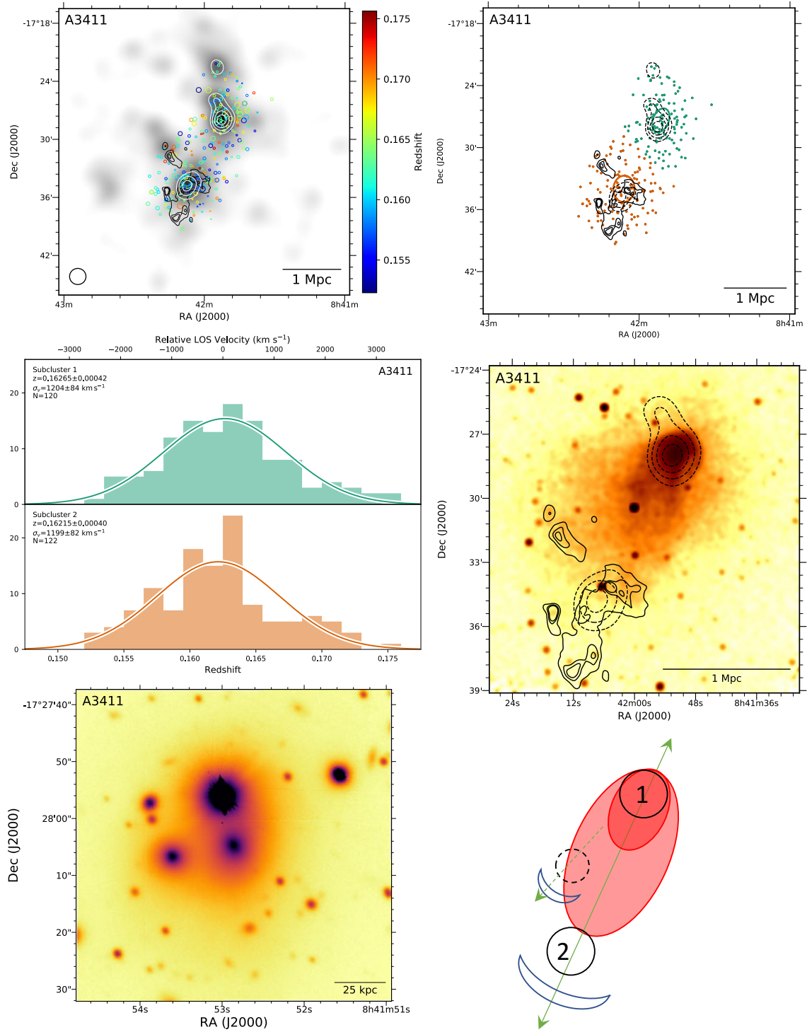
Figure 26. Top left: DS-test over red sequence Subaru/SuprimeCam r-band luminosity distribution with linearly space white contours. The black contours show GMRT 325 MHz contours (van Weeren et al. 2017). Top right: Subcluster membership of spectroscopic cluster members assigned with our GMM analysis. The same GMRT contours (solid) and red sequence luminosity contours (dashed) are depicted. Middle left: Subcluster redshift histogram with colors matching the image at the top right. Middle right: 215 ks Chandra image with the same GMRT radio contours (solid) and red sequence luminosity contours (dashed). Bottom left: 150 kpc cutout of the Subaru r-band image centered on the cluster BCG in subcluster 1. Bottom right: Preferred merger scenario. A3411 is composed of at least two subclusters, where the northern subcluster 1 is A3411 and the southern 2 is A3412. Subcluster 1 is associated with a cool-core remnant and wake feature indicating the ICM is traveling northward. The two subclusters have very similar velocity dispersions and redshifts suggesting a 1:1 mass ratio merger in the plane of the sky. There is evidence of composite structure in subcluster 2 as presented in van Weeren et al. (2017), where a small subcluster has created a shock that reaccelerated particles associated with an AGN.
