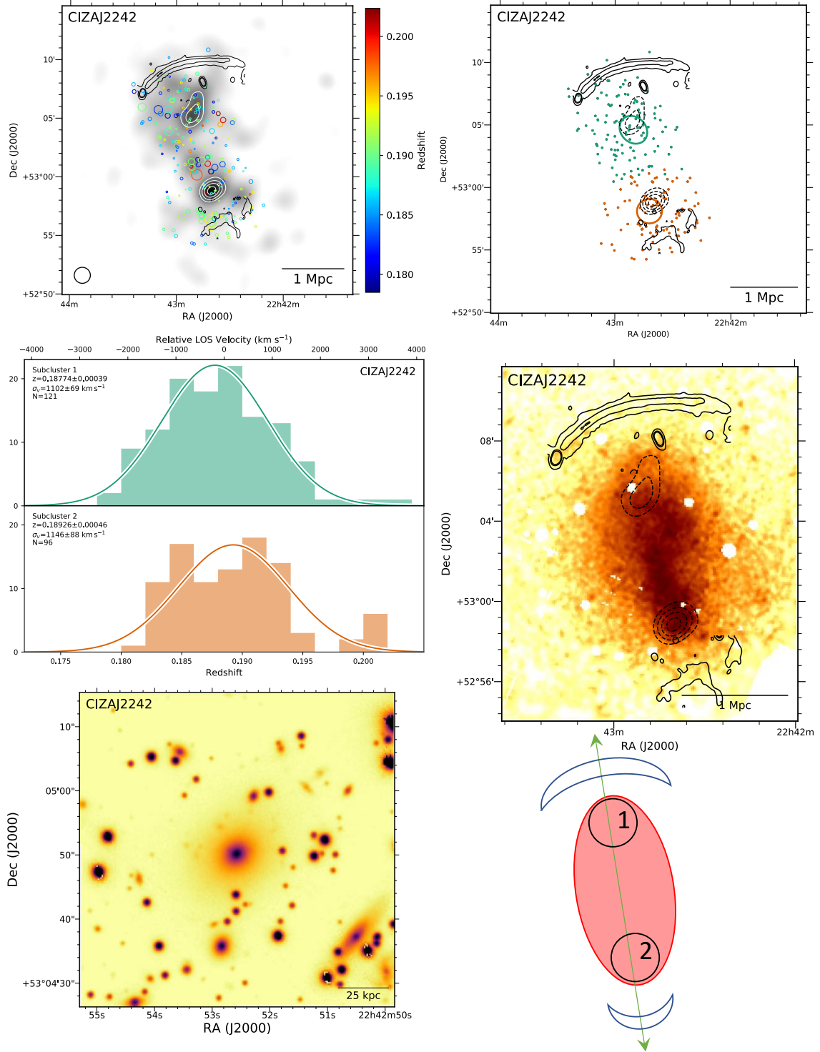
Figure 27. Top left: DS-test over red sequence Subaru/SuprimeCam i-band luminosity distribution with linearly space white contours. The black contours show WSRT 1382 MHz contours (van Weeren et al. 2010). Top right: Subcluster membership of spectroscopic cluster members assigned with our GMM analysis. The same WSRT contours (solid) and red sequence luminosity contours (dashed) are depicted. Middle left: Subcluster redshift histogram with colors matching the image at the top right. Middle right: 206 ks Chandra image with the same WSRT radio contours (solid) and red sequence luminosity contours (dashed). Bottom left: 150 kpc cutout of the Subaru i-band image centered on the cluster BCG in subcluster 1. Bottom right: Preferred merger scenario. CIZA J2242 is composed of at least two subclusters with similar velocity dispersions and redshifts suggesting a 1:1 merger in the plane of the sky. The ICM has been extremely disrupted and is situated between the two subclusters. The famous ‘Sausage’ radio relic in the north has been studied across a wide range of frequencies, and dark matter-galaxy offsets have been detected in this cluster (Jee et al. 2016). The high mass, simple geometry, and extreme shock features have motivated a number of simulation studies as well.
