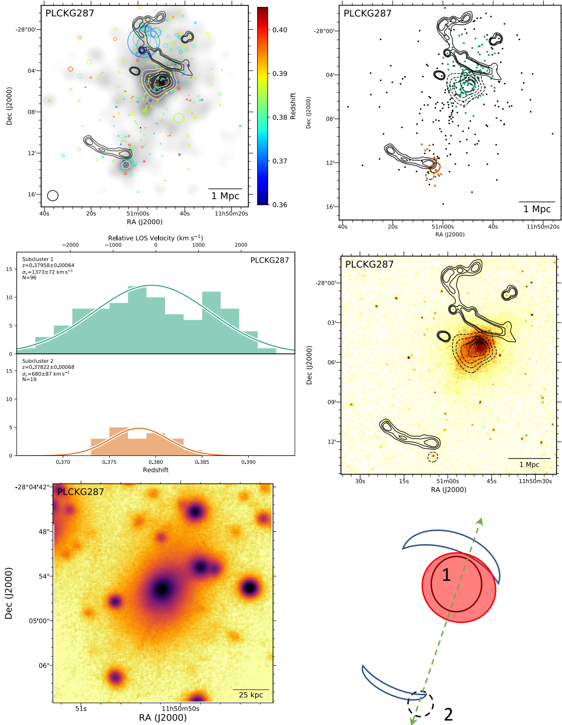
Figure 30. Top left: DS-test over red sequence Subaru/SuprimeCam r-band luminosity distribution with linearly space white contours. The black contours show GMRT 325 GHz contours (Bonafede et al. 2014). Top right: Subcluster membership of spectroscopic cluster members assigned with our GMM analysis. The same GMRT contours (solid) and red sequence luminosity contours (dashed) are depicted. Middle left: Subcluster redshift histogram with colors matching the image at the top right. Middle right: 200 ks Chandra image with the same GMRT radio contours (solid) and red sequence luminosity contours (dashed). Bottom left: 150 kpc cutout of the Subaru i-band image centered on the cluster BCG in subcluster 1. Bottom right: Preferred merger scenario. The merger scenario is unclear. There is evidence for a small subcluster in the south near the southern radio relic; however, it leads the relic. There is disturbed X-ray emission streaming to the south of subcluster 1, which could motivate this merger scenario. A detailed weak gravitational lensing analysis detected composite structure in subcluster 1 (Finner et al. 2017), and more complex scenarios have been proposed (Bonafede et al. 2014).
