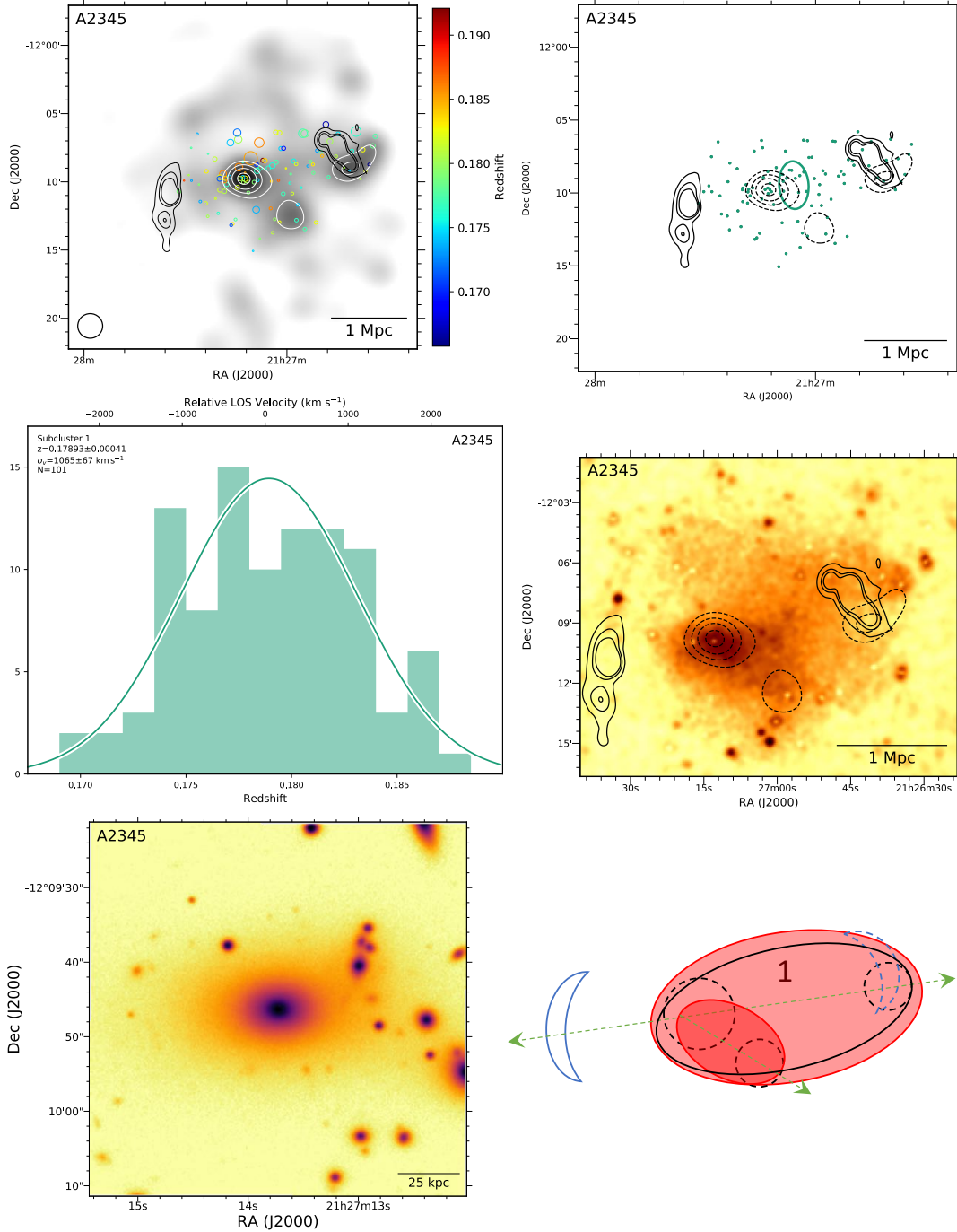
Figure 22. Top left: DS-test over red sequence R-band luminosity distribution with linearly space white contours. The black contours show the 1.4 GHz VLA contours (Bonafede et al. 2009). Top right: Subcluster membership of spectroscopic cluster members assigned with our GMM analysis. The same VLA contours (solid) and red sequence luminosity contours (dashed) are depicted. The low spectroscopic survey density likely contributes to a single halo model being preferred. Middle left: Subcluster redshift histogram with colors matching the image at the top right. Middle right: 93 ks XMM image with the same VLA radio contours (solid) and red sequence luminosity contours (dashed). The relic at the northeast and the disturbed ICM are suggestive of a merger between at least three subclusters, perhaps with a large impact parameter for the northwest subcluster. Bottom left: 150 kpc cutout of the Subaru/SuprimeCam R-band image centered on the cluster BCG in the northeastern subcluster. Bottom right: Preferred merger scenario. The proximity of the western relic to the corresponding subcluster is difficult to explain in a scenario where the two relics were launched with the same merger.
