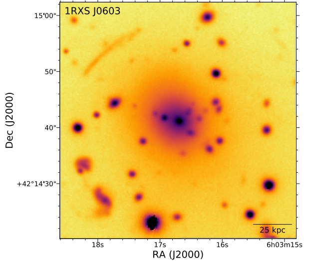
Figure 8. Subaru/SuprimeCam r-band cutout of the inner 150 \times 150 kpc of the BCG of 1RXSJ0603. A strongly lensed arc is apparent along with several light peaks within the inner region of the overall light profile. This figure, along with the 28 analogous figures in the respective following subsections will be analyzed in detail in a forthcoming paper.
