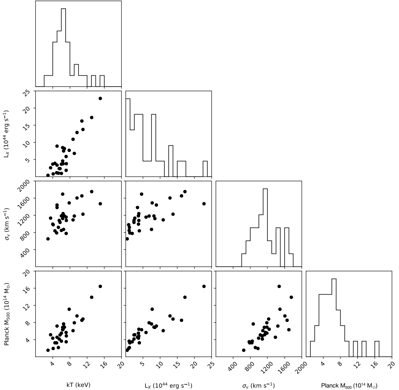
Figure 42. Relationships between four global measures for 29 merging clusters. The clear positive correlation between each suggests that, measuring these values gives a first order understanding of the mass of a merging system. Furthermore, with further lensing and dynamical study, we may understand why given systems have higher \sigma_v with respect to merger dynamics.
