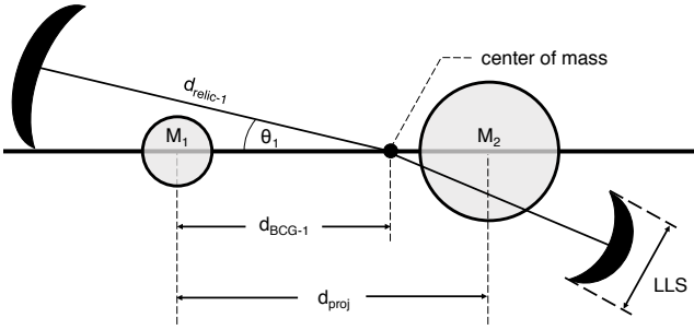
Figure 39. Schematic representation of the relic geometry for a double relic system (e.g. A1240). Each relic is located with a position angle and distance from the center of mass of the system determined from the velocity dispersions of subclusters aligned with the radio relics. Single relic systems follow the same conventions. LLS is an abbreviation for the largest linear scale of a radio relic, which is often quoted in radio astronomy literature and has been shown to correlate with the propagation distance of a shock.
