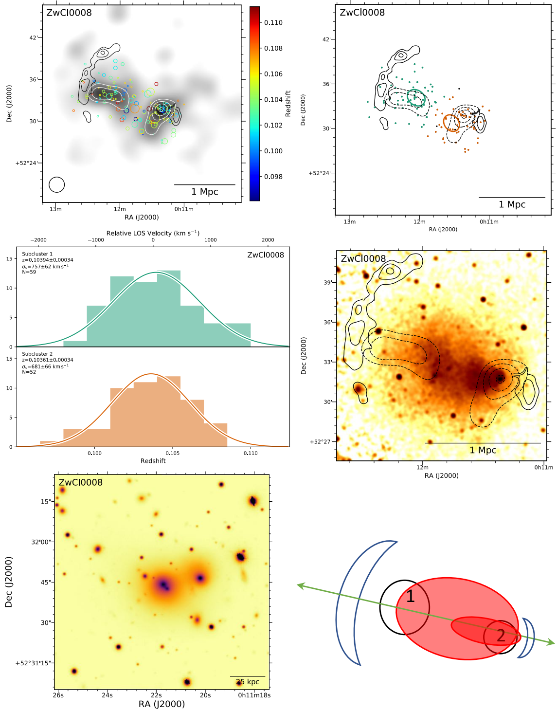
Figure 34. Top left: DS-test over red sequence Subaru/SuprimeCam r-band luminosity distribution with linearly space white contours. The black contours show WSRT 1382 MHz contours (van Weeren et al. 2011c). Top right: Subcluster membership of spectroscopic cluster members assigned with our GMM analysis. The same WSRT contours (solid) and red sequence luminosity contours (dashed) are depicted. Middle left: Subcluster redshift histogram with colors matching the image at the top right. Middle right: 411 ks Chandra image with the same WSRT radio contours (solid) and red sequence luminosity contours (dashed). Bottom left: 150 kpc cutout of the Subaru r-band image centered on the cluster BCG in subcluster 2. Bottom right: Preferred merger scenario. The two subclusters and radio relics are aligned with the extended X-ray emission. A ‘bullet’ like cool-core remnant and wake feature are associated with subcluster 2, which is traveling to the west. The cluster exhibits simple, bimodal geometry indicative of the Bullet Cluster.
