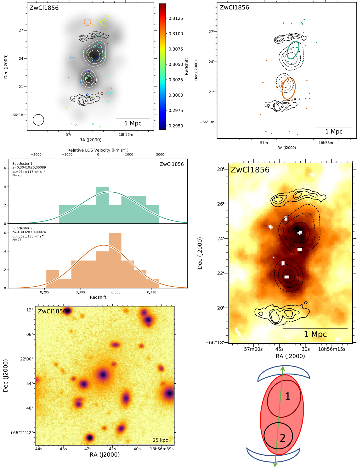
Figure 36. Top left: DS-test over red sequence Gemini/GMOS r-band luminosity distribution with linearly space white contours. The black contours show WSRT 1382 GHz contours (de Gasperin et al. 2014). Top right: Subcluster membership of spectroscopic cluster members assigned with our GMM analysis. The same WSRT contours (solid) and red sequence luminosity contours (dashed) are depicted. Middle left: Subcluster redshift histogram with colors matching the image at the top right. Middle right: 12 ks XMM image with the same WSRT radio contours (solid) and red sequence luminosity contours (dashed). Bottom left: 150 kpc cutout of the Gemini r-band image centered on the cluster BCG in subcluster 2. Bottom right: Preferred merger scenario. We detect two subclusters aligned with the X-ray surface brightness elongation and two radio relics suggesting a simple bimodal merger along a north-south axis. The two subclusters have similar velocity dispersions and redshifts; although, these are based on few galaxies per subcluster.
