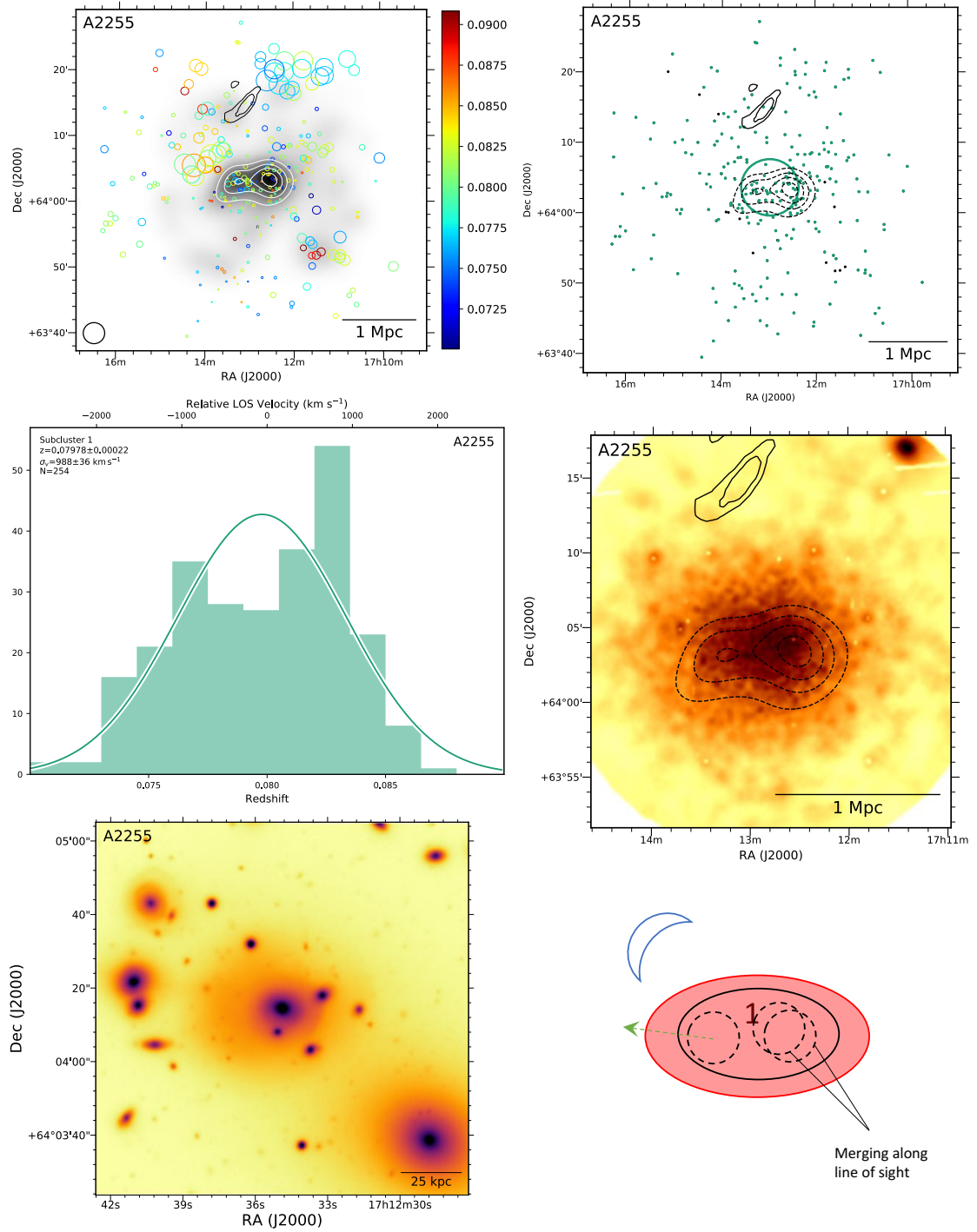
Figure 21. Top left: DS-test over red sequence R-band luminosity distribution with linearly spaced white contours. The black contours show the 350 MHz WSRT contours (Pizzo & de Bruyn 2009). Top right: Subcluster membership of spectroscopic cluster members assigned with our GMM analysis. The same WSRT contours (solid) and red sequence luminosity contours (dashed) are depicted. The small projected separation and low spectroscopic survey density likely contributes to a single halo model being preferred. Middle left: Subcluster redshift histograms with colors matching the image at the top right. Middle right: 42 ks XMM image with the same WSRT radio contours (solid) and red sequence luminosity contours (dashed). The relic at the northeast and the disturbed ICM are suggestive of a merger between at least three subclusters. Bottom left: 150 kpc cutout of the Subaru/SuprimeCam R-band image centered on the cluster BCG in the western half of the cluster. The second BCG apparent in the image has a \sim 2000 km s -1 line of sight velocity difference, which is suggestive of a merger along the line of sight. Bottom right: Preferred merger scenario. The elongation of the X-ray surface brightness suggests a second plane of the sky merger component in addition to the line of sight merger. We do not make a prediction of which subclusters merged to launch the radio relic. We can not rule out further complications in this system.
