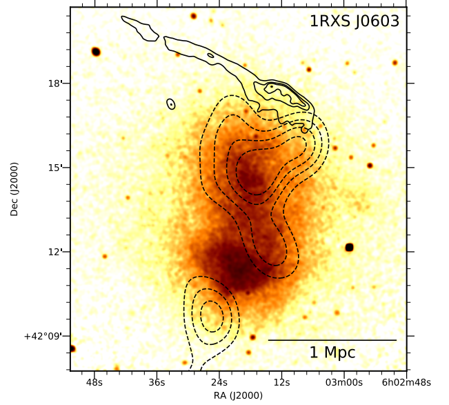
Figure 7. X-ray surface brightness map for 1RXSJ0603 based on a 250 ks of Chandra ACIS exposure. The map is created in the 0.5–2.0 keV band and is exposure corrected. GMRT 610 MHz solid black contours and red sequence luminosity dashed black contours are presented.
