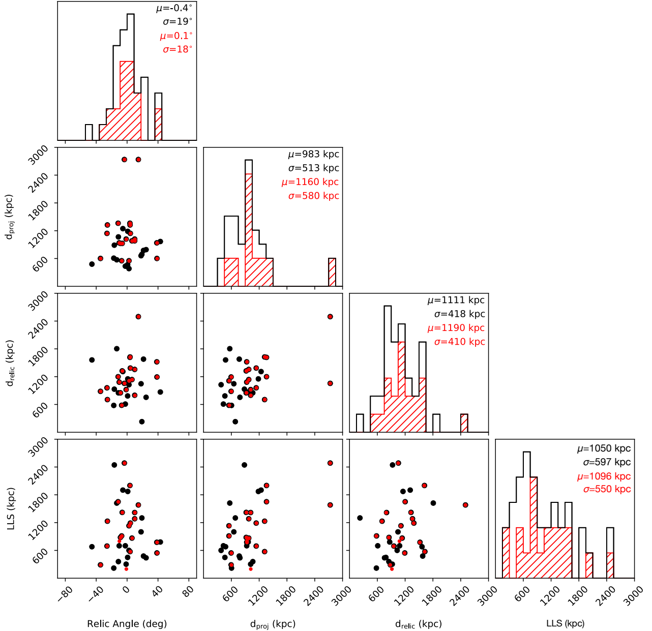
Figure 40. Radio relic geometry for 35 radio relics in 24 merging galaxy clusters. Relics tend to be well aligned with the axis connecting BCGs of merging subclusters. By convention here, negative angles imply clockwise angles from the BCG axis toward the relic position vector. The black distribution is for all relics, and the red distribution is for double relic clusters only. See Figure 39 for a schematic representation of the defined geometry.
