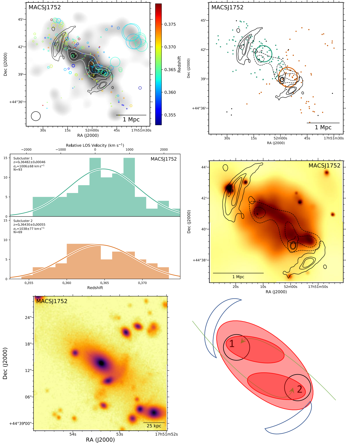
Figure 29. Top left: DS-test over red sequence Subaru/SuprimeCam i-band luminosity distribution with linearly space white contours. The black contours show WSRT 1.4 GHz contours (van Weeren et al. 2012a). Top right: Subcluster membership of spectroscopic cluster members assigned with our GMM analysis. The same WSRT contours (solid) and red sequence luminosity contours (dashed) are depicted. Middle left: Subcluster redshift histogram with colors matching the image at the top right. Middle right: 13 ks XMM image with the same WSRT radio contours (solid) and red sequence luminosity contours (dashed). Bottom left: 150 kpc cutout of the Subaru i-band image centered on the cluster BCG in subcluster 2. Bottom right: Preferred merger scenario. The X-ray image shows evidence for two ‘bullets’ that just missed and are beginning to orbit one another counter-clockwise. There two relics are bright and suggest a major merger despite not being head-on. The two subclusters have similar velocity dispersions and line of sight velocities suggesting the orbital plane is perpendicular to the line of sight.
