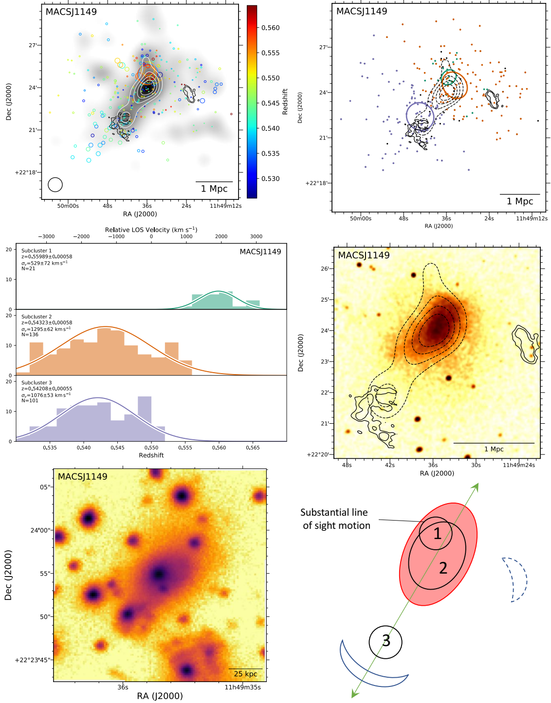
Figure 28. Top left: DS-test over red sequence Subaru/SuprimeCam R-band luminosity distribution with linearly space white contours. The black contours show GMRT 323 MHz contours (Bonafede et al. 2012). Top right: Subcluster membership of spectroscopic cluster members assigned with our GMM analysis. The same GMRT contours (solid) and red sequence luminosity contours (dashed) are depicted. Middle left: Subcluster redshift histogram with colors matching the image at the top right. Middle right: 372 ks Chandra image with the same GMRT radio contours (solid) and red sequence luminosity contours (dashed). Bottom left: 150 kpc cutout of the Subaru R-band image centered on the cluster BCG in subcluster 2. Bottom right: Preferred merger scenario. A detailed dynamical study of MACSJ1149 was presented in Golovich et al. (2016).
