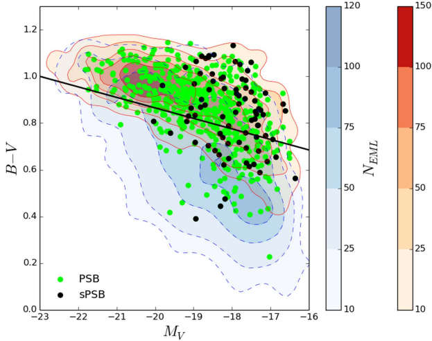
Figure 3. Rest-frame (B - V) - V relation for cluster galaxies of the different spectral types. Red-solid and blue-dashed contours are the number densities of PAS and EML galaxies, respectively. Green dots: PSB; black dots: sPSB. The black line represents the selection limit we adopt to select red and blue galaxies.
