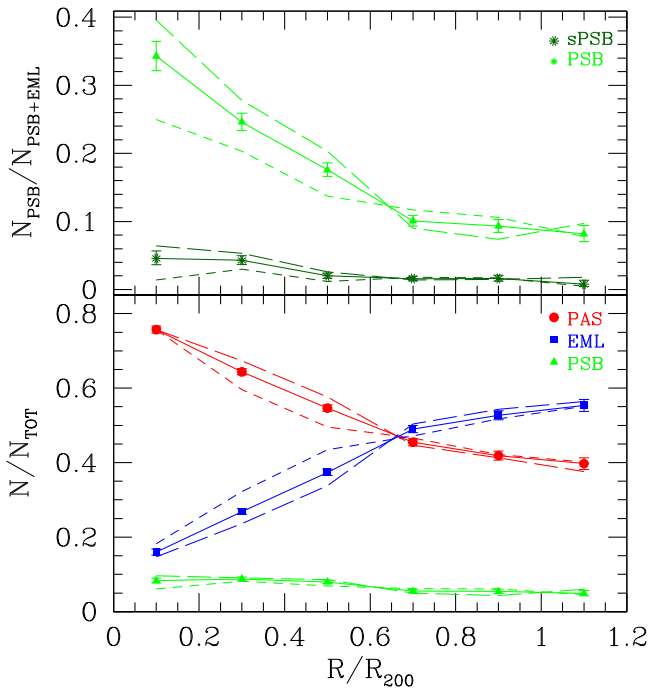
Figure 4. Ratio of post-starburst to active galaxies (top panels) and ratio of post-starburst, passive, and emission-line galaxies to the total (bottom panels) as a function of R/R_{200} . Points with error bars represent cluster fractions, dashed lines give the trends of the respective fractions in two bins of velocity dispersion \sigma ( \sigma < 840 \text{ km s}^{-1} —short dashed lines—and \sigma > 840 \text{ km s}^{-1} —long dashed lines). Errors are binomial (Gehrels 1986).
