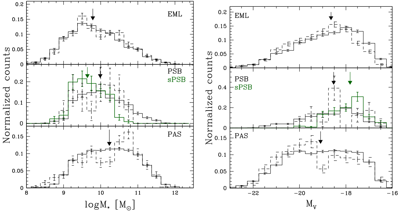
Figure 2. Number of cluster (solid) and field (dashed) galaxies in the three main spectral types as a function of stellar mass (left panel) and absolute V magnitude (right panel). Dark green histograms in the middle panels show the sPSB subsample. Arrows indicate the median value for each type. Errors are Poissonian (Gehrels 1986).
