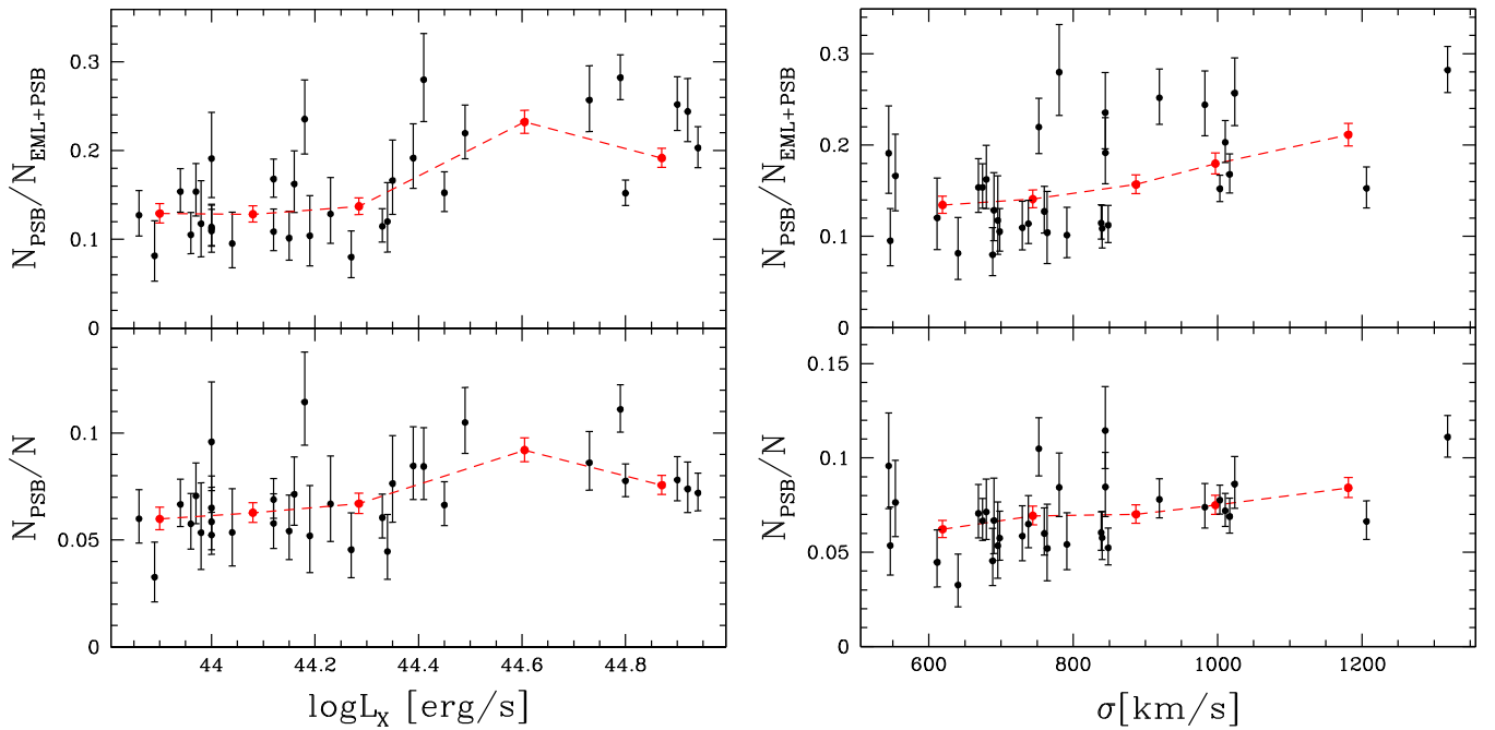
Figure 7. Fraction of post-starburst galaxies as a function of the cluster X-ray luminosity (left) and velocity dispersion (right). Black points represent individual clusters, red points give the fractions in five equally populated bins. Lower panels: weighted fraction of post-starburst galaxies among the whole population. Upper panels: weighted fraction of post-starburst galaxies among the active population. Errors are binomial.
