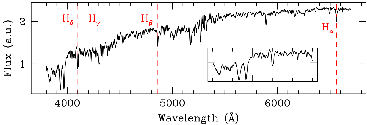
Figure 1. Rest-frame composite spectrum of the post-starburst cluster sample. The inset shows a zoom in of the spectral region around H\delta .
