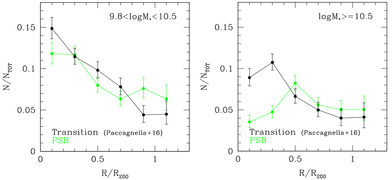
Figure 8. Radial distribution of transition galaxies (black) as defined by Paccagnella et al. (2016) and of PSB galaxies (green), in two bins of stellar mass. Errors are binomial.
