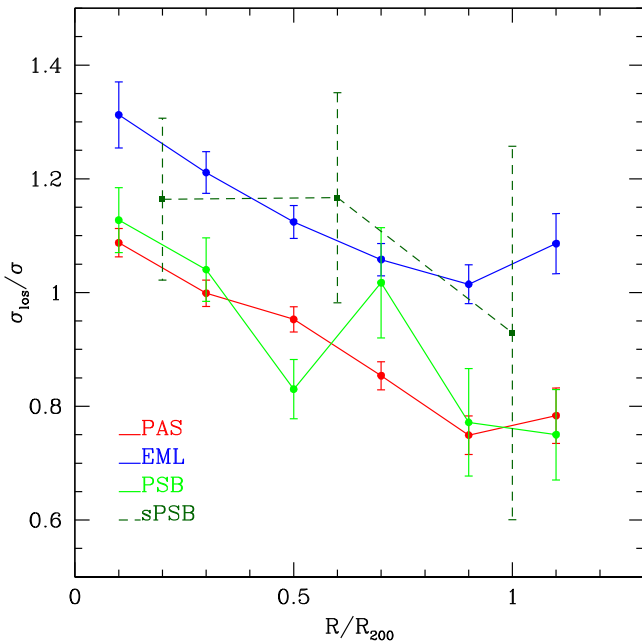
Figure 6. Velocity-dispersion profiles ( \sigma_{\text{LOS}}(r)/\sigma ) of each galaxy population; colors refer to the different populations as described in the labels and as in Figure 4. Errors are jackknife standard deviations (Efron 1982).
