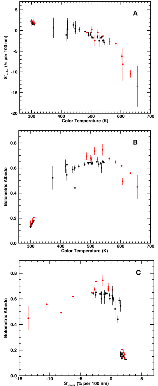
Figure 6. Correlation trends between colour temperature ( T_{\text{col}} ), 2–2.5 \mu m colour ( S'_{\text{col}} ), and bolometric albedo ( A(\theta) ). Black and red symbols are for 13 Sept. and 14 Sept. data, respectively.
