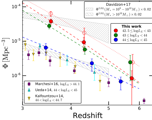
Figure 20. Comoving space density of three luminosity classes of AGN, divided in three redshift bins ( z = 3-4 , 4-5 , 5-6 ). The points are located at the weighted average redshift of each subsample. For the low-luminosity bin, the empty circles indicate the results derived applying the correction factors described in § 4. At higher luminosities, the corrections have negligible effects, and are not shown for clarity. Since high-luminosity sources are not well sampled by the deep, pencil-beam fields used in this work, we report previous results in similar luminosity bins derived analyzing data from wider fields. The dashed curves are the best-fitting models described in § 6. The dotted curve is the best-fitting model for the low-luminosity bin, after the correction for incompleteness. The space density of galaxies in two different mass regimes from Davidzon et al. (2017), rescaled by an arbitrary factor of 0.02, is shown as a grey stripe.
