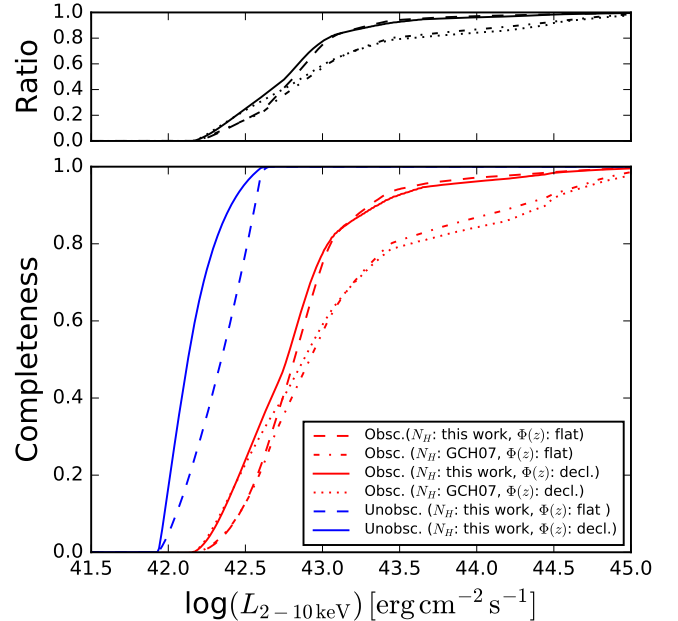
Figure 14. Detection completeness at the 7 Ms CDF-S depth as a function of luminosity for obscured (red lines) and unobscured (blue lines) sources, assuming different intrinsic distributions of column density (the one presented in this work in Fig. 7 and the one used in Gilli et al. 2007 ) and redshift (flat or more realistically declining with redshift as \propto 10^{-6(1+z)} ; e.g. Hiroi et al. 2012 ; Vito et al. 2013 ), as described in § 4. For the unobscured case, the curve corresponding to the two column-density distributions are almost indistinguishable and therefore are not plotted for clarity. The solid lines have been used to derive the correction factors applied to Fig. 16 and 18. The upper panel presents the ratio of the completeness of obscured and unobscured sources.
