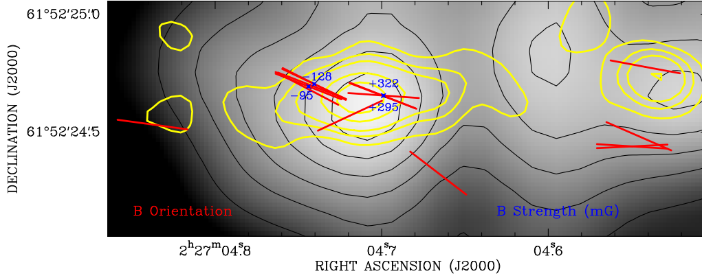
Figure 2. Magnetic field orientation (in the plane of the sky) for 17 individual masers with P_l < 5\% (red segment) and strength for 4 (non-saturated) masers for which the Zeeman splitting was measured. The 8.4 GHz emission imaged with the VLA (beamsize \sim 0''.2 ) by Wilner et al. (1999) (yellow contours) is overplotted onto the 1.4 mm continuum emission mapped with the PdBI (beamsize \sim 0''.5 ) by Wyrowski et al. (1999) (gray scale and black contours: same as in Fig. 1).
