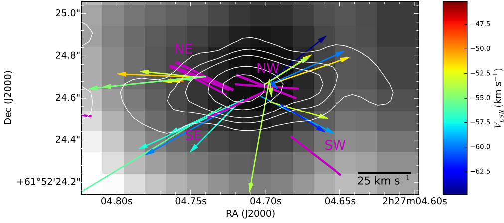
Figure 3. Comparison between the magnetic field orientations of H 2 O masers (purple segments) and proper motions of H 2 O masers (arrows). The 8.4 GHz emission imaged with the VLA by Wilner et al. (1999) (white contours) is overlaid onto the 1.4 mm continuum emission mapped with the PdBI by Wyrowski et al. (1999) (gray scale). Colors denote l.o.s. velocity (color scales on the right-hand side) and the scale for the proper motion amplitude is given in the lower right corner (both in \text{km s}^{-1} ). There are four main knots of masers, located towards NE, NW, SE, and SW, with respect to the radio continuum peak. The proper motions identify a biconical, bipolar molecular outflow. Note the misalignment between magnetic field and velocity vectors, particularly in the NE and NW knots.
