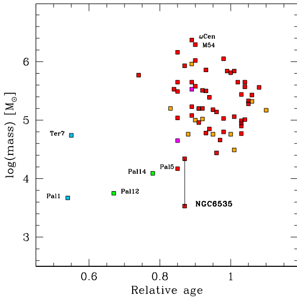
Fig. 10. As in the previous figure, but only for GCs and using mass instead of M_V . Shown are the two values for NGC 6535 ( McLaughlin & van der Marel 2005 ; and that derived in Sect. 6), joined by a line.
