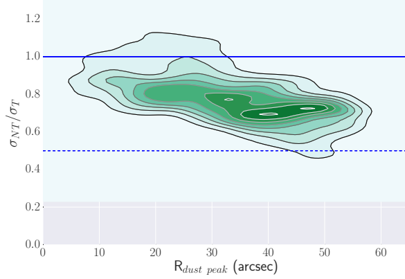
Figure 5. Ratio of non-thermal components of the three methanol lines to the thermal line width of a mean particle as a function of distance from the dust peak. The solid and dashed blue horizontal lines show the \sigma_{NT}/\sigma_T ratios equal to 1 and 0.5. The colour scale and grey contours represent the number of the data points. Only the data points within the primary beam are used for the plot. The grey area does not contain any data points.
