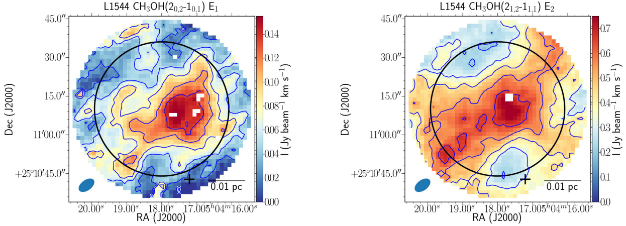
Figure A.1. Integrated intensities of the methanol lines (NOEMA+30 m) for the E_1 (left) and E_2 (right) lines. The blue contours represent integrated intensity, and start at 0.027 Jy beam -1 km s -1 with a step of 0.027 Jy beam -1 km s -1 for the E_1 line (left), and at 0.108 Jy beam -1 km s -1 with a step of 0.108 Jy beam -1 km s -1 for the E_2 line (right). 3\sigma_I = 0.005 Jy beam -1 km s -1 . The circle shows the primary beam of NOEMA. The cross shows the dust emission peak (Ward-Thompson et al. 1999). The synthesized beam of NOEMA is shown in the bottom left corner. The white pixels are those masked because of low quality spectra.
