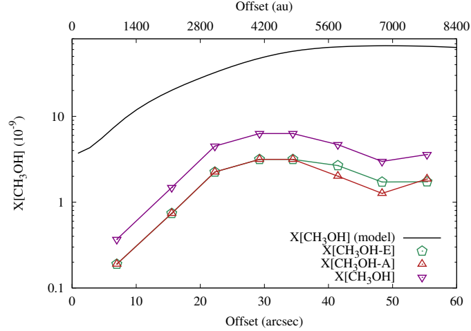
Figure 14. The abundances of \text{CH}_3\text{OH} from non-LTE modelling with MOLLIE (A shown with red, E with green, and the total abundance, the sum of A-methanol and E-methanol abundances shown with purple) and the methanol abundances predicted by Vasyunin et al. (2017) (black line).
