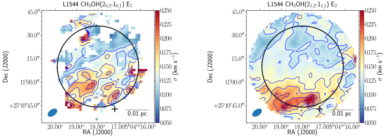
Figure A.2. Velocity dispersions of the methanol lines for the E_1 (left) and E_2 (right) lines. The blue contours show velocity dispersions of 0.125, 0.150, 0.175, 0.200, and 0.225 km s -1 . The circle shows the primary beam. The cross shows the 1.3 mm dust emission peak (Ward-Thompson et al. 1999). The synthesized beam is shown in the bottom left corner. The white pixels are those masked because of low quality spectra.
