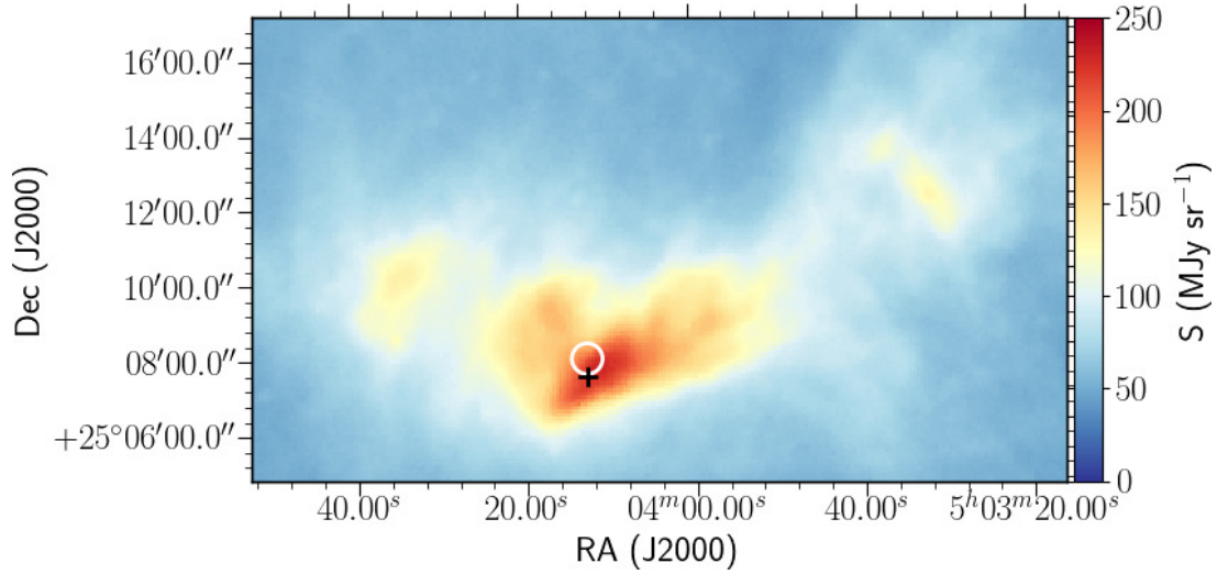
Figure 13. The 250 \mu m dust continuum emission Herschel /SPIRE map towards the L1544 region (André et al. 2010). The white circle shows the NOEMA primary beam centred at the methanol peak. The black cross shows the 1.3 mm dust emission peak (Ward-Thompson et al. 1999).
