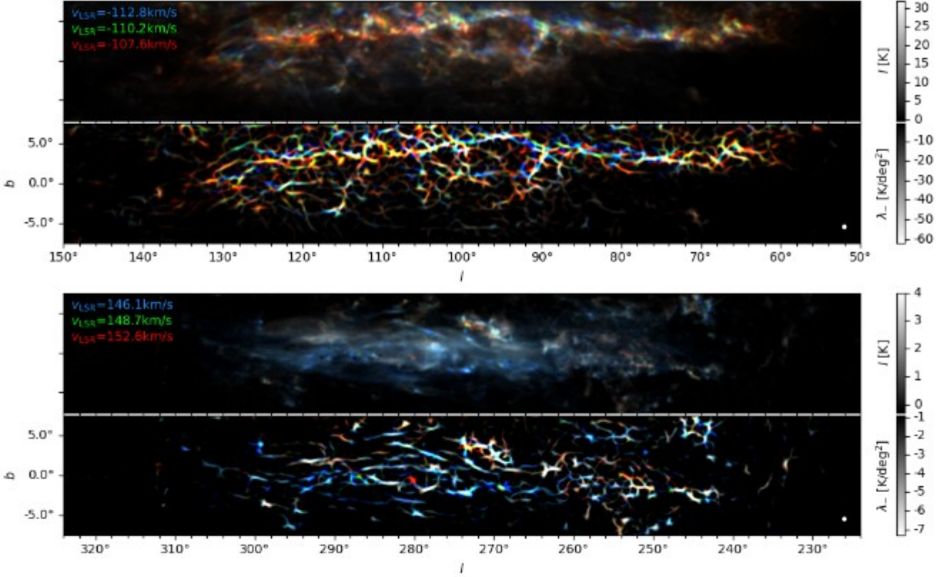
Fig. 3: Examples of the H I emission and filamentary structures toward the l and v_{\text{LSR}} ranges with predominantly horizontal filamentary structures. The top image in each panel corresponds to the H I emission intensity in three velocity-channel maps presented in red, green, and blue colors. The bottom image corresponds to the second eigenvalue of the Hessian matrix, \lambda_- , which highlights the filamentary structures in each velocity-channel map. The white disk in the lower right corner corresponds to the size of the derivative kernel used to calculate the Hessian matrix.
