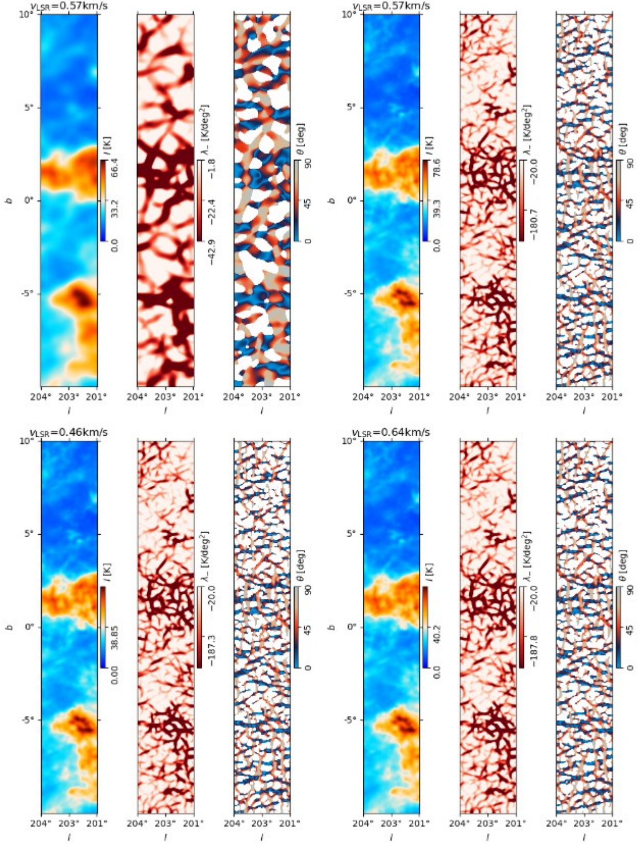
Fig. C.1: Hessian matrix analysis applied to the HI4PI and the GALFA-HI observations. Top. Results obtained on a 3^\circ \times 20^\circ \times 1.29 \text{ km s}^{-1} tile in the HI4PI and the GALFA-HI observations, shown in the left and right panels, respectively. Bottom. Results obtained on two 3^\circ \times 20^\circ \times 0.184 \text{ km s}^{-1} tiles in the GALFA-HI observations. In each of the panels, the left-hand side map shows the HI emission convolved with a 2D Gaussian with the same diameter of the derivative kernel. The map in the center shows the second eigenvalues of the Hessian matrix, \lambda_- , which highlights the filamentary structure. The right-hand side map shows the orientation angle of the filamentary structure.
