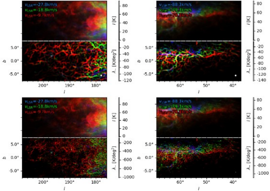
Fig. 13: Examples of the HI emission and filamentary structures identified in the HI4PI and the GALFA-HI data, shown in the top and bottom panels respectively. The disk in the lower right corner of each panel indicates the size of the derivative kernels used for the calculation of the Hessian matrix, 18' and 5' for the HI4PI and the GALFA-HI observations, respectively.
