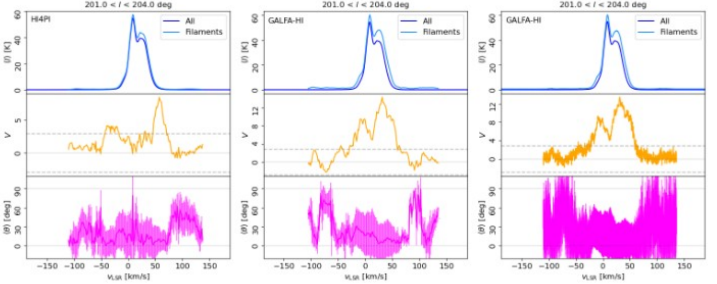
Fig. 16: Mean intensity ( \langle I \rangle , top ), projected Rayleigh statistic ( V , middle ), and mean orientation angle of the filaments ( \langle \theta \rangle , bottom ) for the tiles centered on l = 202.5 in the HI4PI and GALFA-HI. The left panel corresponds to the HI4PI observations analysis with a 18' FWHM kernel for a 1.29\text{-km s}^{-1} velocity resolution. The center and right panels correspond to the GALFA-HI observations analysis with a 5' FWHM kernel for 1.29\text{-km s}^{-1} and 0.184\text{-km s}^{-1} velocity resolutions, respectively.
