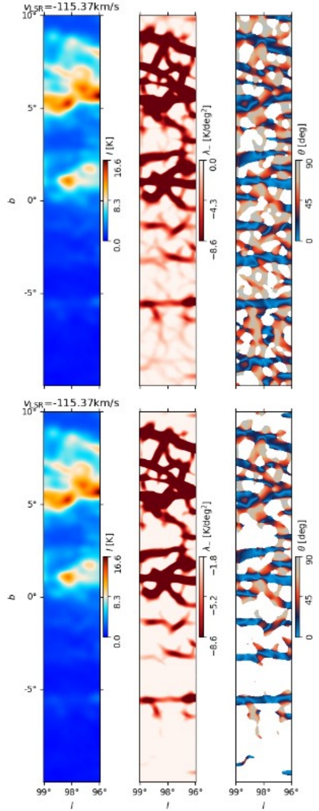
Fig. A.11: Example of the filamentary structures identified using the Hessian method with curvature thresholds \lambda_- < 0 (top) and \lambda_- < -1.8 \text{ K/deg}^2 (bottom). The three maps represent: Left . HI intensity after the smoothing by a Gaussian kernel with the size of the derivative kernel. Center . Second eigenvalue of the Hessian matrix, \lambda_- , calculated using Eq. 2. Right . Filament orientations, \theta , calculated using Eq. 3. The radial velocity corresponds to a kinematic distance d = 12.7 \text{ kpc} and Galactocentric radius R_{\text{gal}} = 16.1 \text{ kpc} , as derived using the assumptions in App. B
