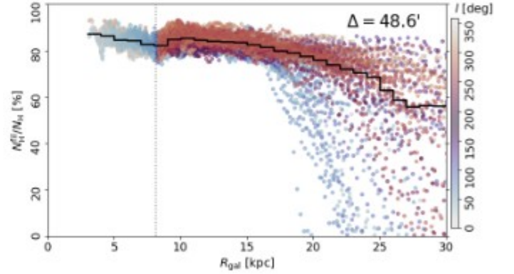
Fig. A.9: Same as Fig. 12, but for 32.4' and 48.6' FWHM derivative kernels, shown in the top and the bottom panels, respectively.
