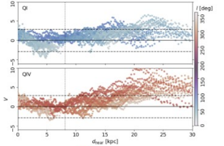
Fig. B.2: Same as Fig. B.2, but for the near heliocentric kinematic distances.
