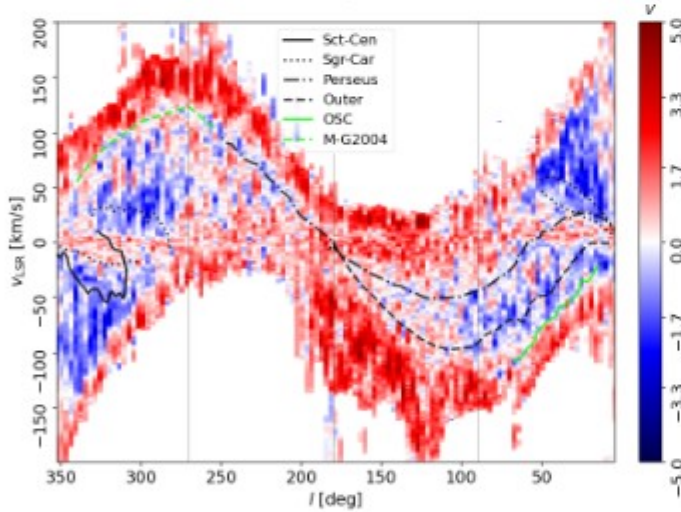
Fig. A.7: Same as Fig. A.3, but for 3^\circ \times 20^\circ \times 1.29 \text{ km s}^{-1} tiles analyzed using 32.4' and 48.6' FWHM derivative kernels, shown in the top and the bottom panels, respectively.
