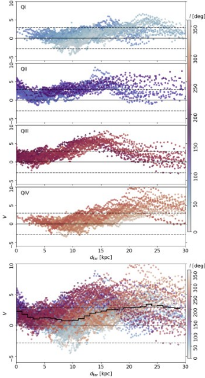
Fig. 4: Kinematic heliocentric distance ( d ) and projected Rayleigh statistic ( V , Eq. 4) for the 3^\circ \times 20^\circ \times 1.29 \text{ km s}^{-1} tiles. We report the largest (far) solution to the heliocentric distance equation, as detailed in App. B. From top to bottom, the panels correspond to each Galactic quadrant and to the whole Galactic longitude range. The colors indicate the Galactic longitude of the tiles. The horizontal dashed lines indicate V = \pm 2.87 , which correspond to the 3\sigma significance in the preferential orientation around \theta = 0^\circ or \theta = 90^\circ , respectively. The solid line in the bottom panel corresponds to the mean V values in 1-kpc R_{\text{gal}} bins.
