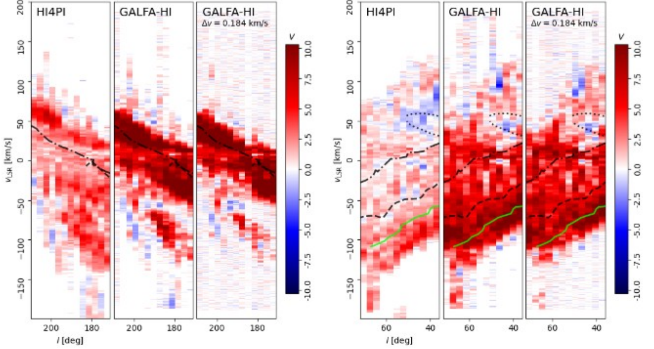
Fig. 14: Longitude-velocity ( lv ) diagrams of the filament orientation quantified by the projected Rayleigh statistic ( V , right) in the two portions of the Galactic plane covered in the range |b| \leq 10^\circ by both HI4PI and GALFA-HI. The GALFA-HI observations were analyzed at 1.29 and 0.184 \text{ km s}^{-1} resolution using a 5' FWHM derivative kernel. The curves correspond to the same spiral arm features introduced in Fig. 1.
