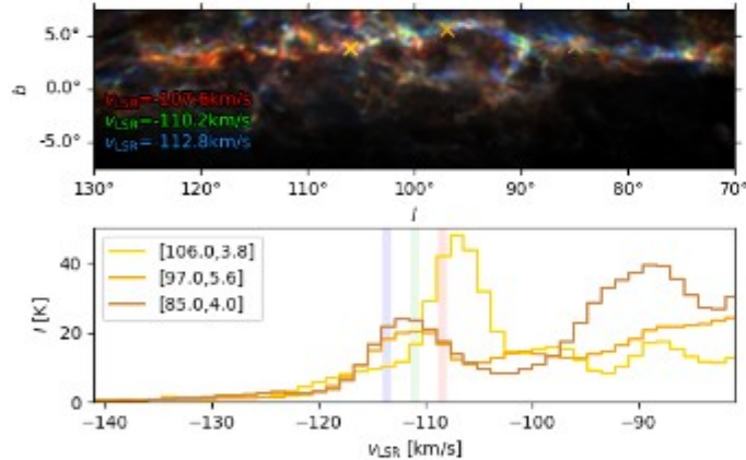
Fig. 19: H I emission ( top ) and selected spectra toward filamentary structures ( bottom ). The spectra correspond to the positions indicated by the crosses in the upper panel. The colored vertical bars in the bottom panel correspond to the three velocity channels presented in the corresponding colors in the top panel.
