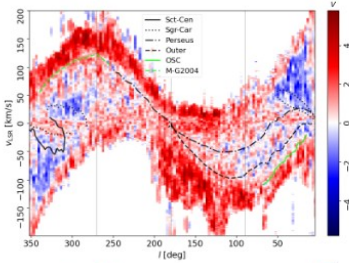
Fig. A.6: Same as Fig. 7, but for tile sizes 10^\circ \times 20^\circ \times 1.29 \text{ km s}^{-1} .
