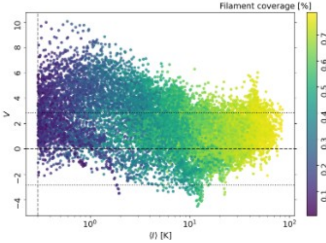
Fig. 2: Mean H I emission intensity ( \langle I \rangle ) and projected Rayleigh statistic ( V , Eq. 4) for the 3^\circ \times 20^\circ \times 1.29 \text{ km s}^{-1} tiles. The colors indicate the tile percentage covered by the filamentary structures selected following the criteria described in Sec. 3.2. The horizontal dotted lines show V = \pm 2.87 , which indicate the 3\sigma significance in the preferential orientation parallel, \theta = 0^\circ , or perpendicular, \theta = 90^\circ , to the Galactic plane, respectively. The vertical dashed line indicates the intensity threshold.
