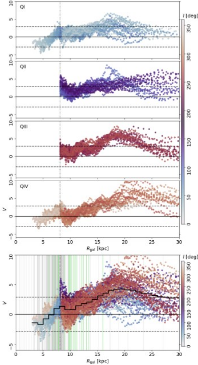
Fig. 7: Galactocentric radius ( R_{\text{gal}} ) and projected Rayleigh statistic ( V , Eq. 4) for the 3^\circ \times 20^\circ \times 1.29 \text{ km s}^{-1} tiles. From top to bottom, the panels correspond to each Galactic quadrant and to the whole Galactic longitude range. The colors indicate the Galactic longitude of the tiles. The horizontal dashed lines indicate V = \pm 2.87 , which indicate the 3\sigma significance in the preferential orientation around \theta = 0^\circ or \theta = 90^\circ , respectively. The vertical dotted line indicates the radius of the solar orbit. The solid line in the bottom panel corresponds to the mean V values in 1-kpc R_{\text{gal}} bins. The vertical solid lines mark the central locations of the HI shells identified in the LAB survey (Ehlerová & Palouš 2013) and the SGPS (McClure-Griffiths et al. 2002) in the range |b| < 10^\circ , shown in gray and green colors, respectively.
