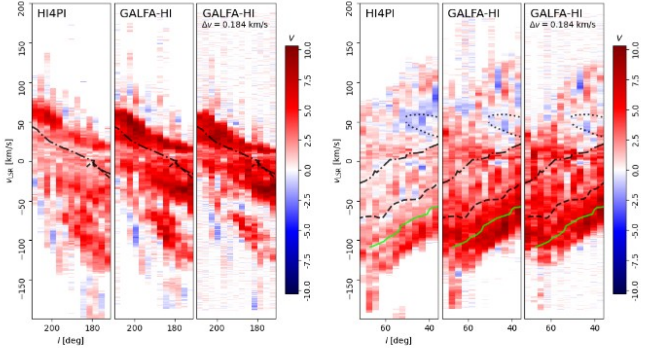
Fig. C.2: Same as Fig. 14, but for an 8' FWHM kernel.
