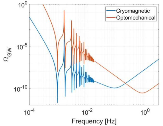
Figure 4. Predicted LGWA sensitivity to stochastic GW backgrounds.
