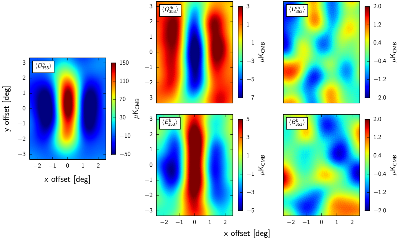
Fig. 10. Mean images of the Planck \langle D^b_{353} \rangle , \langle Q^b_{353} \rangle , \langle U^b_{353} \rangle , \langle E^b_{353} \rangle , and \langle B^b_{353} \rangle maps over the \lambda_- filaments.
