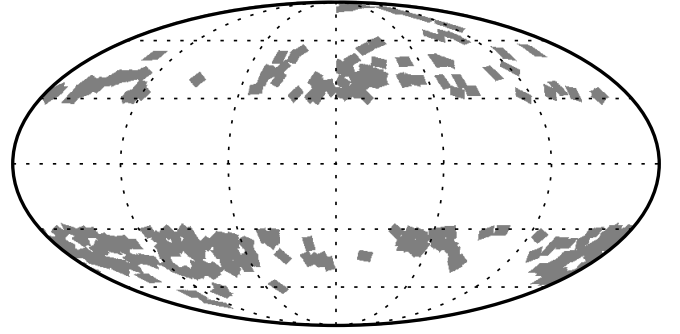
Fig. 12. Map of the selected pixels (grey colour) used in the stacking analysis. It covers 28% of the high-latitude sky. Each tile in the image is a 7^\circ \times 5^\circ patch around the filament centre and rotated by \bar{\theta}_- .
