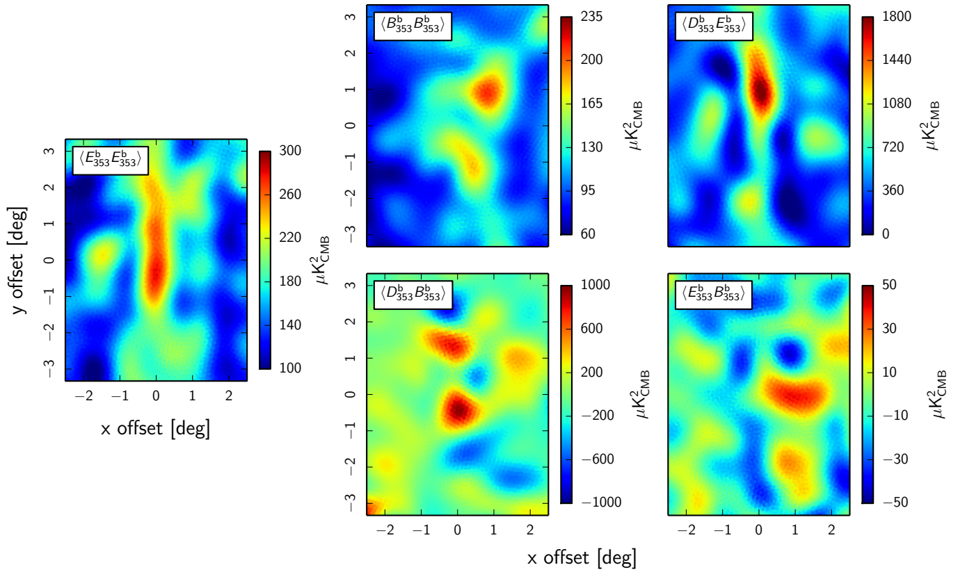
Fig. 11. Mean images of the Planck \langle E^b_{353} E^b_{353} \rangle , \langle B^b_{353} B^b_{353} \rangle , \langle D^b_{353} E^b_{353} \rangle , \langle D^b_{353} B^b_{353} \rangle , and \langle E^b_{353} B^b_{353} \rangle maps over the \lambda_- filaments.
