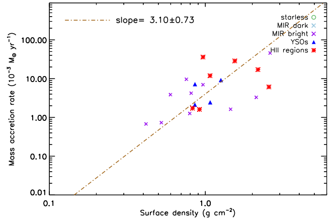
Figure 13. Mass accretion rate as a function of surface density. The Pearson correlation coefficient is 0.61, suggesting a good correlation between these two quantities. The best fit gives a slope of 3.10 \pm 0.73 , suggesting an increase of \dot{M} as a function of \Sigma .
