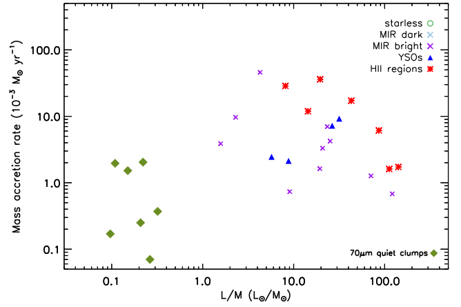
Figure 12. Mass accretion rate as a function of the L/M ratio, an indicator of clump evolution. Our sample of 21 clumps has been combined with the survey of 70- \mu m quiet clumps in Traficante et al. (2017, green diamonds). These data show a moderate correlation ( \rho = 0.44 ) and suggest that the mass accretion rate might increase with evolution.
