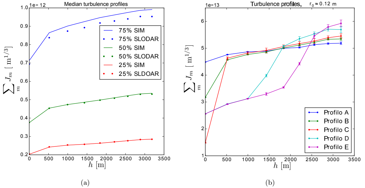
FIGURE 2: Reconstruction of realistic turbulence profiles.
