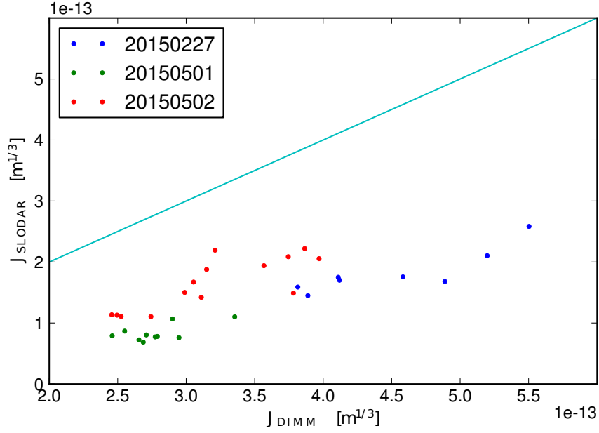
FIGURE 4: Turbulence strength ( h < 3\text{ km} ) measured with the SLODAR technique as function of the DIMM measure.
