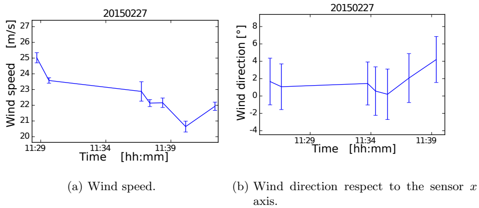
FIGURE 6: Wind measurements in the 20150227 night.
