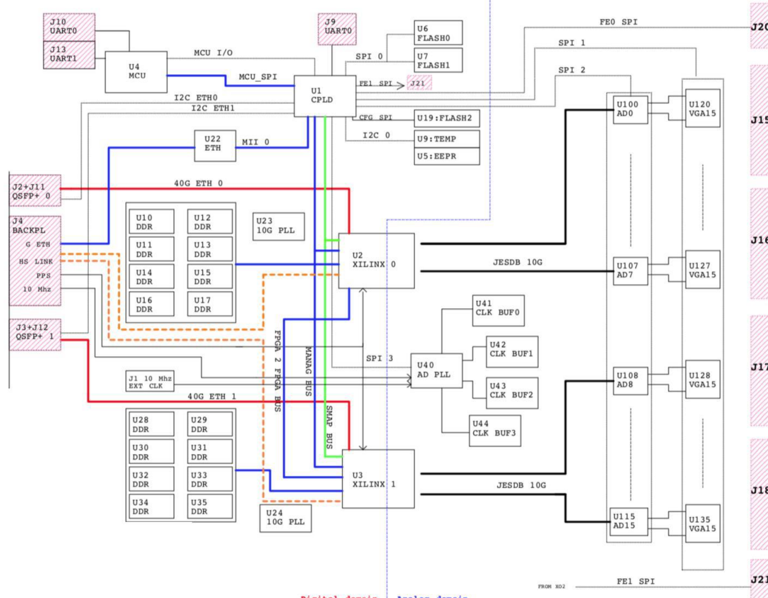
ITPM 1.6 ADU Board Schematic
