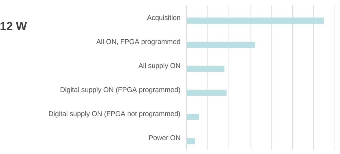
Power Supply for Operational Mode (W)
