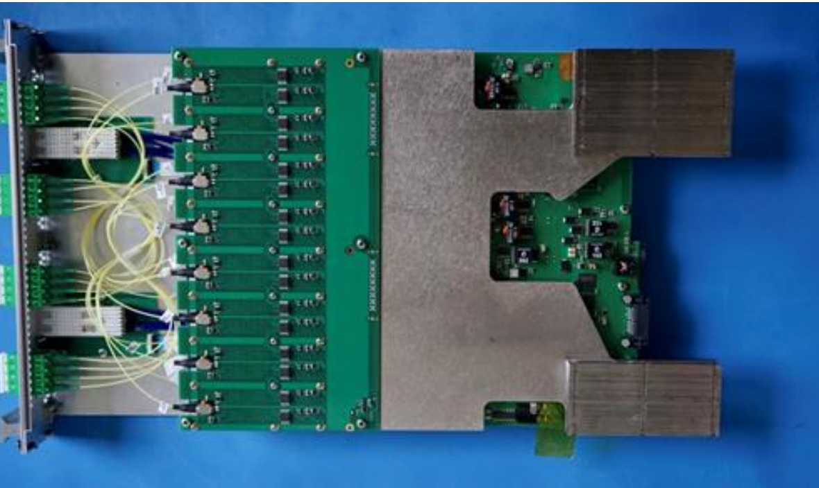
ITPM 1.6 assembly: PRE-ADU (left), ADU (right)
