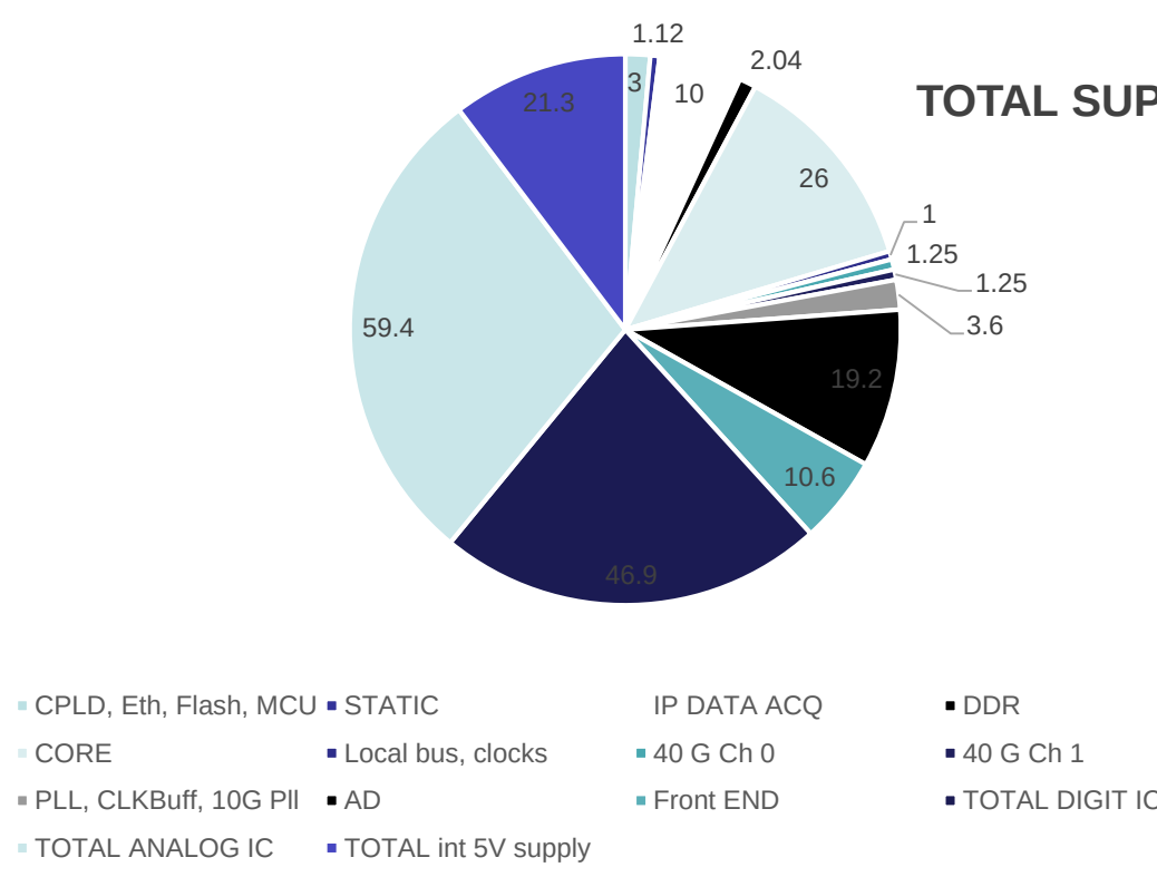
ITPM Power Budget for Components (W)
