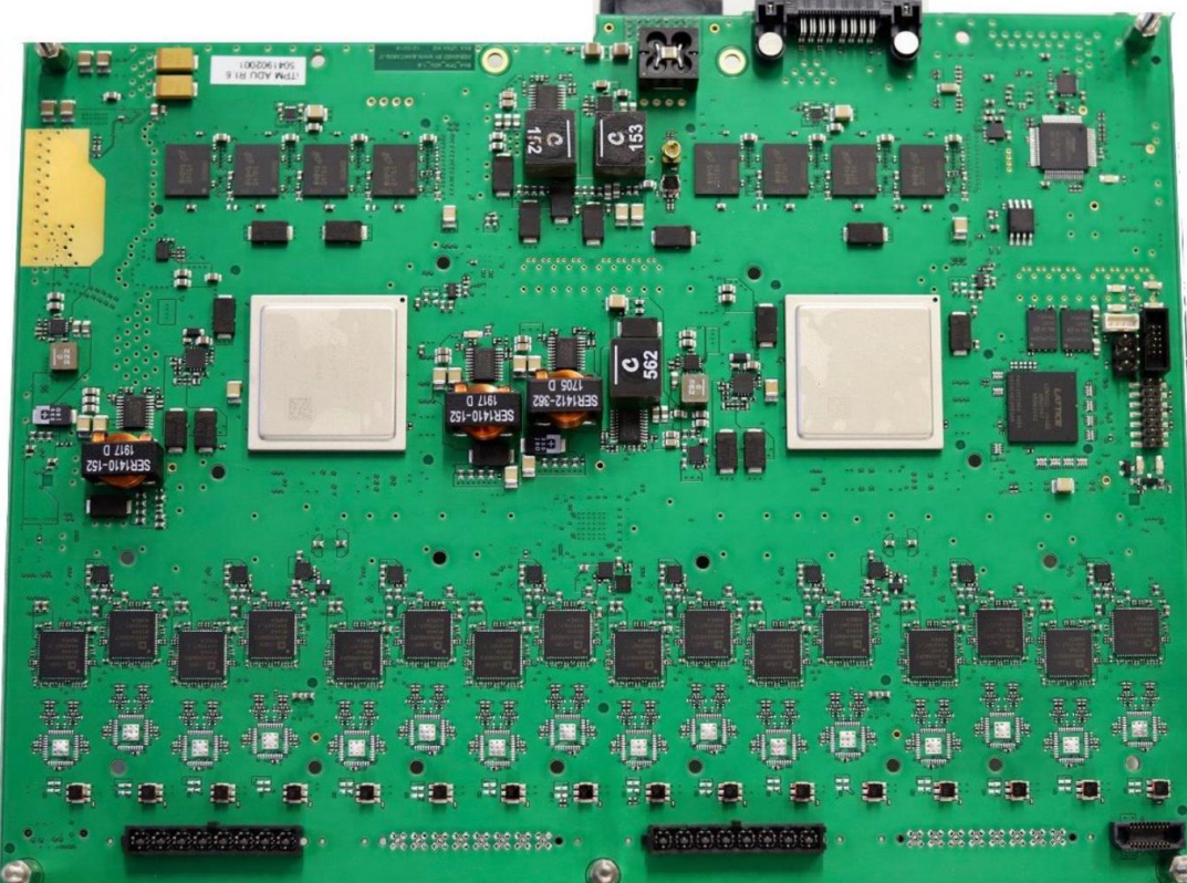
ITPM 1.6 ADU Board top view
