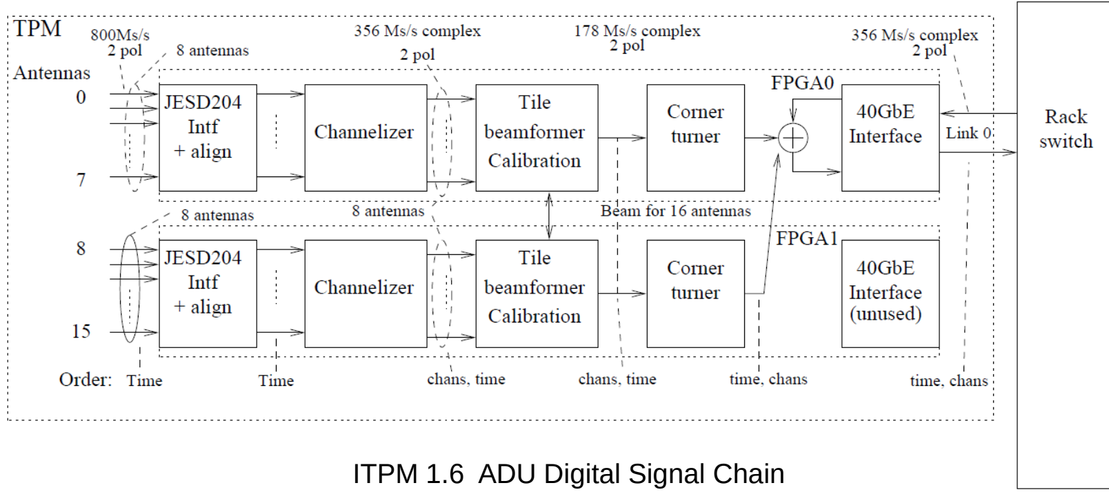
ITPM 1.6 ADU Digital Signal Chain
