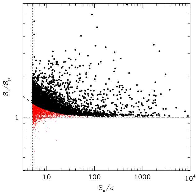
Figure 6. Integrated to peak flux ratio as a function of the source signal-to-noise ratio. Lines indicate the S/N = 5 cut-off adopted in the source catalogue extraction (dotted), the locus S_p/S_p = 1 (solid), and the envelop function defined by equation (2) (dashed). Red dots correspond to unresolved sources; and black filled circles correspond to resolved or partially resolved sources (i.e. those sources that are resolved only along the major axis).
