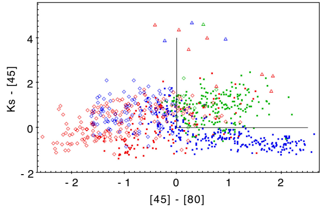
Figure A3. KI diagnostic plot for the identified sources with S \geq 0.12 mJy: 4.5–8.0 \mu\text{m} against K_s - 4.5 \mu\text{m} (all quantities are AB magnitudes). Source colour-coding as in Fig. A2. Sources detected at all three bands ( K band, 4.5 and 8.0 \mu\text{m} ) are shown as filled points; sources not detected at 8.0 \mu\text{m} only are shown as open diamonds; sources not detected at K band only are shown as upward triangles. Sources detected only at 4.5 \mu\text{m} are shown as crosses. Sources not detected at any of the three bands cannot be constrained and are not shown. The black solid lines represent the AGN wedge as defined by Messias et al. (2012).
