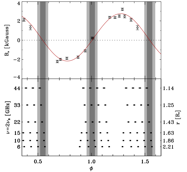
Figure 12. Top panel: effective magnetic field curve of HR 7355, are from Rivinius et al. (2010) and Oksala et al. (2010), a sinusoidal fit of the data is superimposed. Bottom panel: phase coverage of the radio observations. The y-axis on the right indicates the distances of the layers where the observing frequencies coincide with the second harmonic of the local gyro-frequency. Gray areas represent a phase interval that is 5% of the full rotation period; the light-gray areas represent an interval of \Delta\phi = 10\% around the phases where the effective magnetic field of HR 7355 is null.
