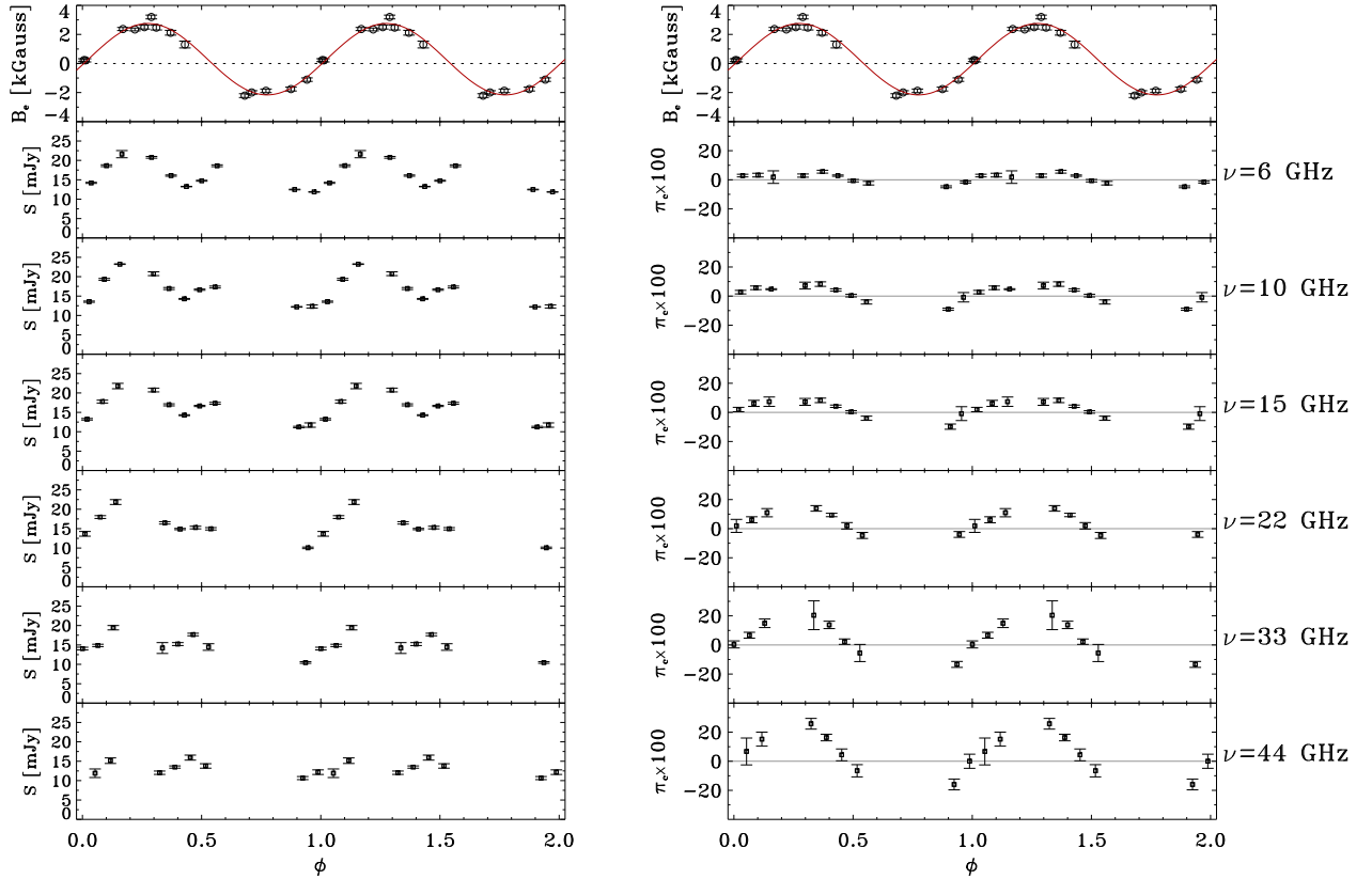
Figure 2. Left and right top panels show the magnetic curve of HR 7355 and data taken by Oksala et al. (2010) and Rivinius et al. (2010) . The other left panels show the radio light curves for Stokes I obtained at all the observing frequencies. Right panels display the rotational modulation of the fractionally circularly polarized radio emission.
