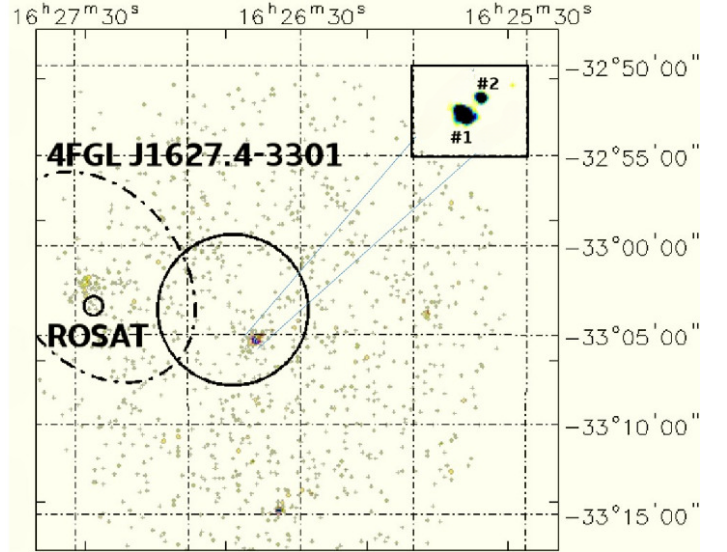
Figure 2: XRT 0.3–10 keV image of the region surrounding IGR J16267–3303. Two X-ray sources (see close-up inset of the region) lie within the 90% IBIS positional uncertainty (black circle). Also plotted are the error ellipse of the Fermi source 4FGL J1627.4–3301 (black dash-dotted ellipse), which partially intersects the IBIS error circle, and the ROSAT Faint source 1RXS J162725.1–330322 displayed with its positional uncertainty (smaller black circle).
