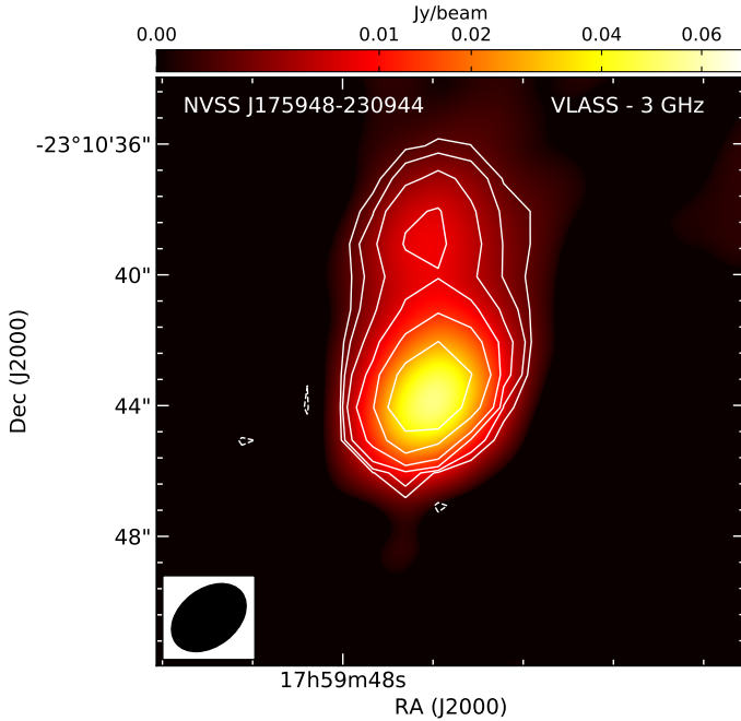
Figure 9: VLASS image of NVSS J175948–230944.
