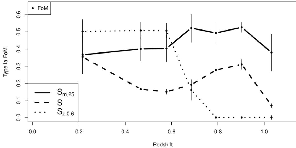
Figure 9.4: Values for the FoM-Ia as function of redshift from (Richards et al. 2012, Figure 11). Curves are reported for different training sets. Dashed curve is relative to SNPhotCC training set. Is has to be compared with continuous curve in Figure 9.3.
