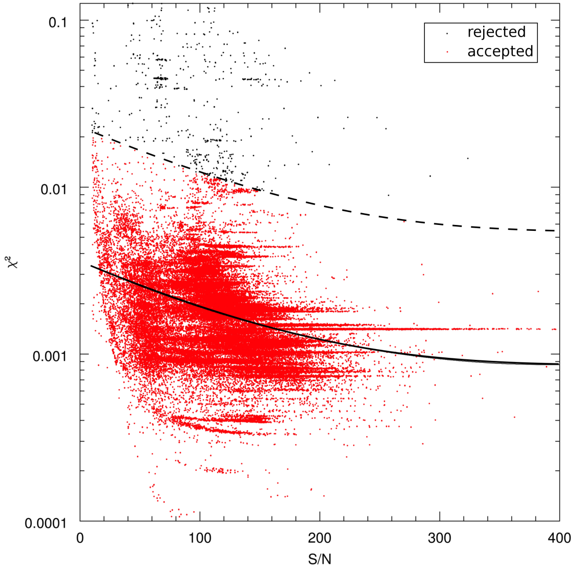
Figure 1.7: Spectra selection on the basis of the \chi^2 quality criterion as function of S/N for stars with 5\,000\text{ K} < T_{\text{eff}} \leq 6\,500\text{ K} . The solid line traces the second degree polynomial fit to those spectra. The red points are the selected spectra, starting from a threshold of three times the standard deviation above the fit.
