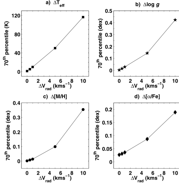
Figure 1.4: Internal error for each parameter as function of uncertainty on the V_{\text{rad}} . Panel a reports the \Delta T_{\text{eff}} that the 70% of the synthetic sample were less than or equal to when calculating the difference between the nominal T_{\text{eff}} and the T_{\text{eff}} determined for the respective V_{\text{rad}} uncertainty. Panel b as for a but for \log g . Panel c as for a but for [\text{M/H}] . Panel d as for a but for [\alpha/\text{Fe}] . Figure 11 from Worley et al. (2012).
