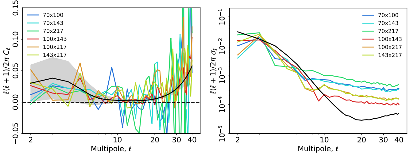
Fig. 83. Left: Cross-power spectra for the four Planck frequency maps at 70, 100, 143, and 217 GHz compared to the Planck2018 best-fit model for EE (solid black line). Right: Standard deviation of the sum of noise, systematics, and uncertainties related to foreground cleaning for the cross-frequency spectra computing using Monte Carlos as compared to the cosmic variance (solid black line).
