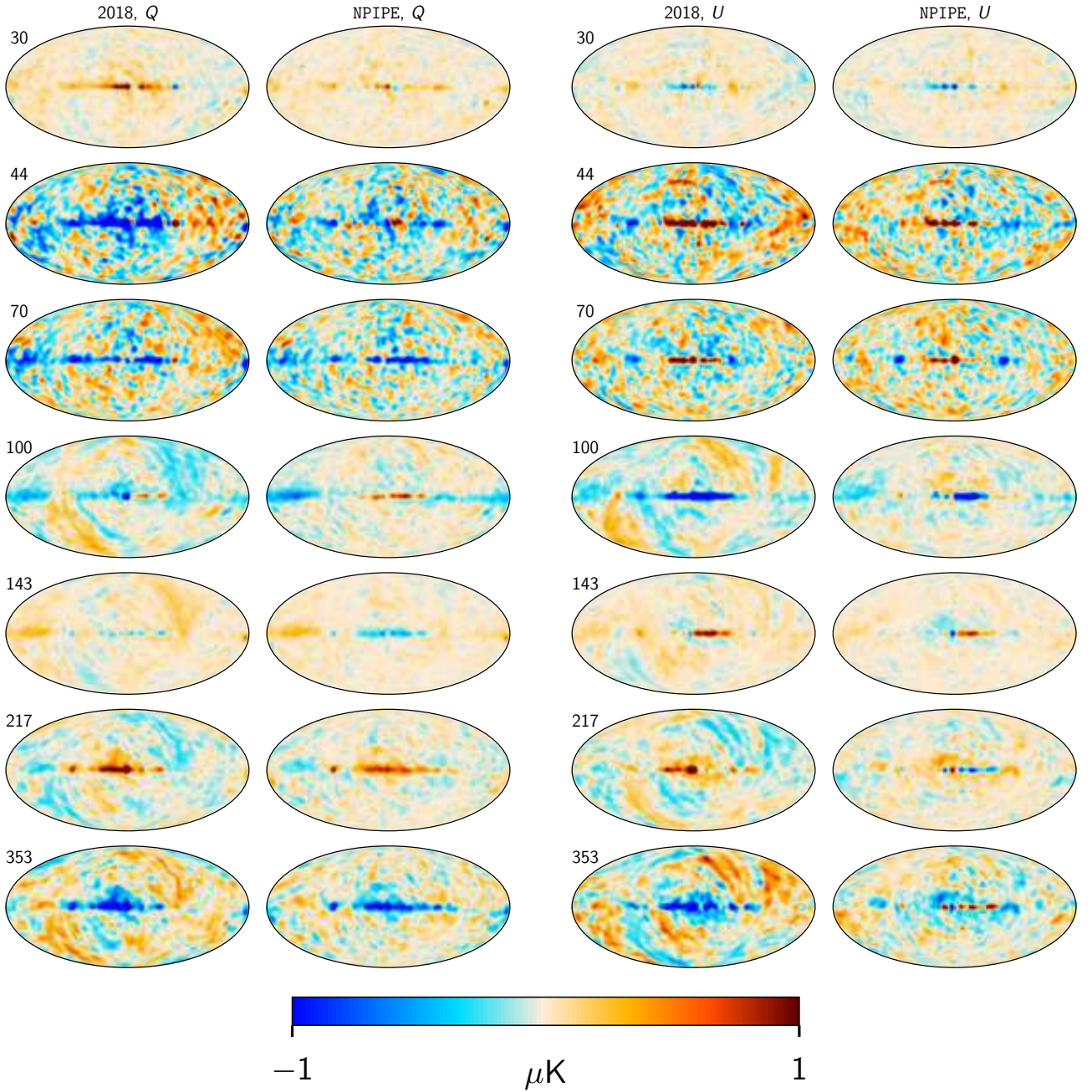
Fig. 54. Comparison between Commander residual maps, d_\nu - s_\nu , for each polarized Planck frequency map between (from top to bottom) 30 and 353 GHz. The two leftmost columns show residual maps for Stokes Q for Planck 2018 and NPIPE, while the two rightmost columns show the same for Stokes U . All maps have been smoothed to a common angular resolution of 3^\circ FWHM.
