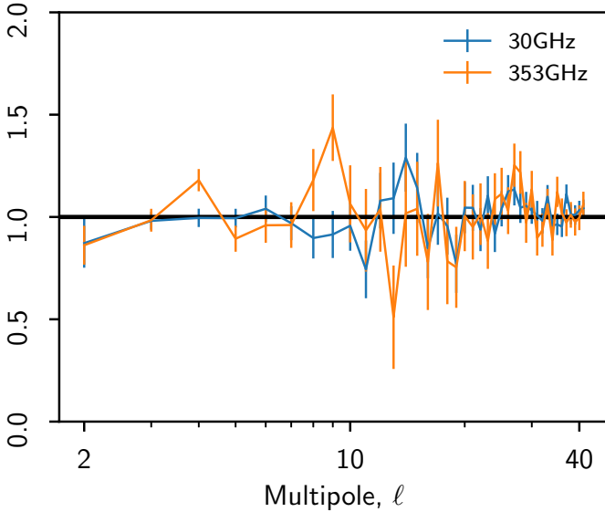
Fig. 21. NPIPE E -mode transfer functions, measured by comparing simulated CMB input and foreground-cleaned output maps over 60 % of the sky. The 30 and 353 GHz frequencies are not expected to have a measurable transfer function because they are not calibrated with a polarization prior. These two transfer functions are merely of diagnostic value (to demonstrate the absence of signal suppression) and are not applied in any analysis. The error bars reflect the statistical uncertainty of the measured transfer function, not the total Monte Carlo scatter. Tabulated values of the transfer functions are listed in Table G.1.
