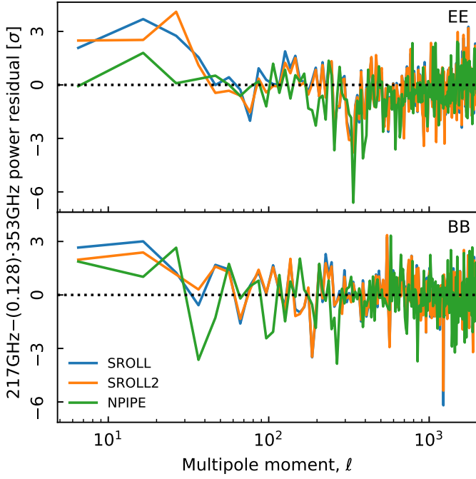
Fig. 49. Angular cross-spectra evaluated from m_{217} - 0.128 m_{353} difference maps. For NPIPE, the cross-spectra are evaluated from detector-split difference maps, while for SROll and SROll2 they are evaluated from half-mission split difference maps.
