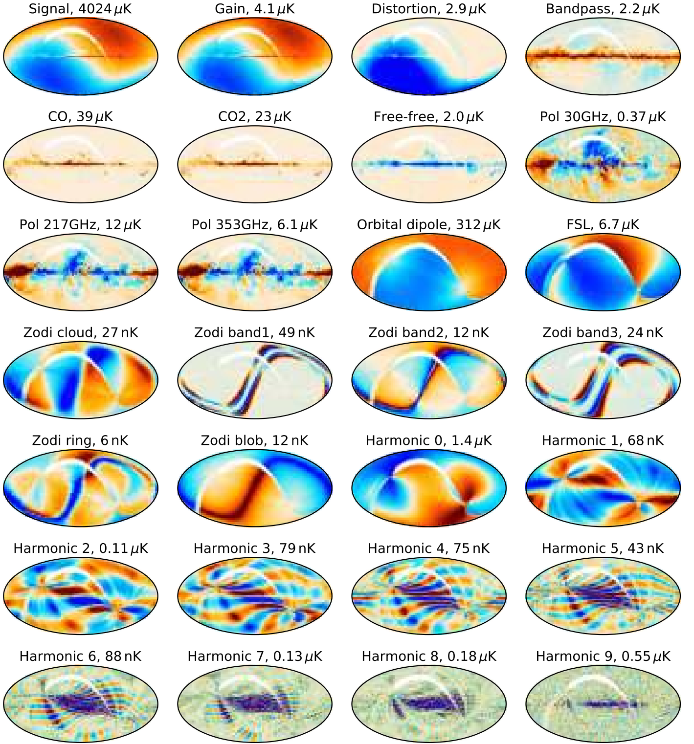
Fig. E.2. Binned maps of detector 100-1a signal and systematics templates for the first survey. For details, see the caption for Fig. E.1.
