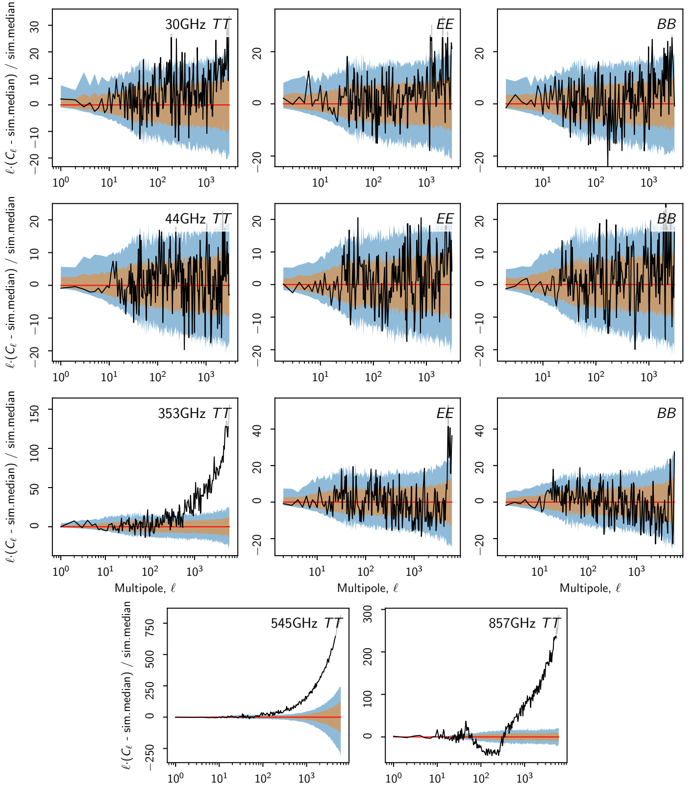
Fig. 34. Simulated A/B difference versus flight data at 30, 44, 353, 545, and 857 GHz. All spectra are differenced and divided by the median simulated spectrum. The flight data are shown in black, and the median simulated power in each bin is plotted in red. The coloured bands represent the asymmetric 68 % and 95 % confidence regions. The power spectra are binned into 300 logarithmically-spaced bins. The spectra shown here are the same as in Fig. 28. Notice the \ell -scaling.
