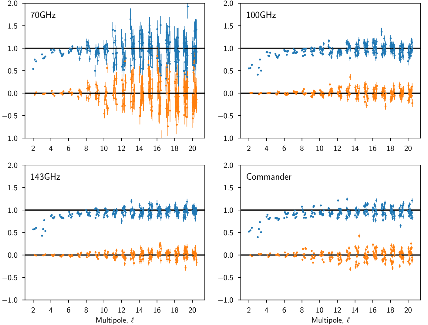
Fig. 24. Full anisotropic transfer functions for 70, 100, and 143 GHz and Commander. These demonstrate that the signal suppression is not completely uniform for the quadrupole and the octupole. The real part of the transfer function is shown in blue. The imaginary part (orange) of the transfer function is consistent with zero. These transfer functions correspond to minimizing Eq. (18) over 80 % of the sky. The different m modes are slightly staggered here, with m = 0 \dots \ell plotted left to right, to aid visualization.
