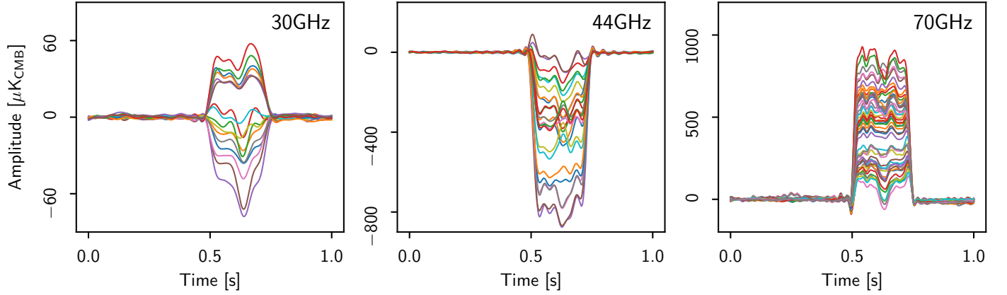
Fig. 5. LFI spike templates built from the harmonic templates fitted to each of the 44 timelines. Each of the coloured curves represents a different diode. The CMB temperature fluctuations have a maximum amplitude of about 250 \mu\text{K}_{\text{CMB}} and the polarization fluctuations about 2 \mu\text{K}_{\text{CMB}} . The 1-Hz features would be seen at approximately \ell = 60 .
