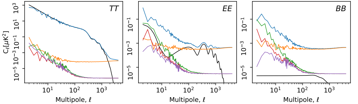
Fig. F.2. Power spectra of the simulated full-mission ADCNL effect over 50 % of the sky, corrected for the sky fraction. The green curve shows the full, unmitigated effect. Red shows the residual after the linear (first order) gain correction, and magenta shows the residual after applying the gain and distortion templates (second order), as is done in NPIPE. For scale, the power spectrum of the full 143 GHz frequency map is shown in blue, and an instrumental noise estimate (from the half-ring, half-difference map) is shown in orange. The theoretical input power spectrum ( \tau = 0.06 ) used in the simulation is in black. The residual maps are shown in Fig. F.1. The EE residuals are deconvolved from the NPIPE transfer function (Sect. 4.3).
